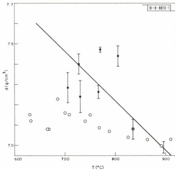
Fig. II-2. Density ( d ) of \text{Bi}_2\text{Te}_3(\ell) as a function of temperature. Present data are shown with error bars of \pm one standard deviation. Open circles are from Ref. 6.
