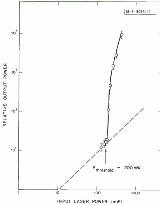
Fig. I-11. Spin-flip Raman output power versus pump power in InSb ( n = 1 \times 10^{16} \text{ cm}^{-3} , H = 35 \text{ kG} , \lambda_{\text{pump}} = 5.32 \text{ } \mu\text{m} , T \sim 30^\circ\text{K} ).
