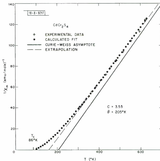
Fig. III-4. Agreement obtained by using high-temperature expansion to fit our experimental inverse susceptibility data for \text{CdCr}_2\text{S}_4 . Dashed extrapolation illustrates standard procedure for determining \theta ; solid line represents true asymptote as computed from power series.
