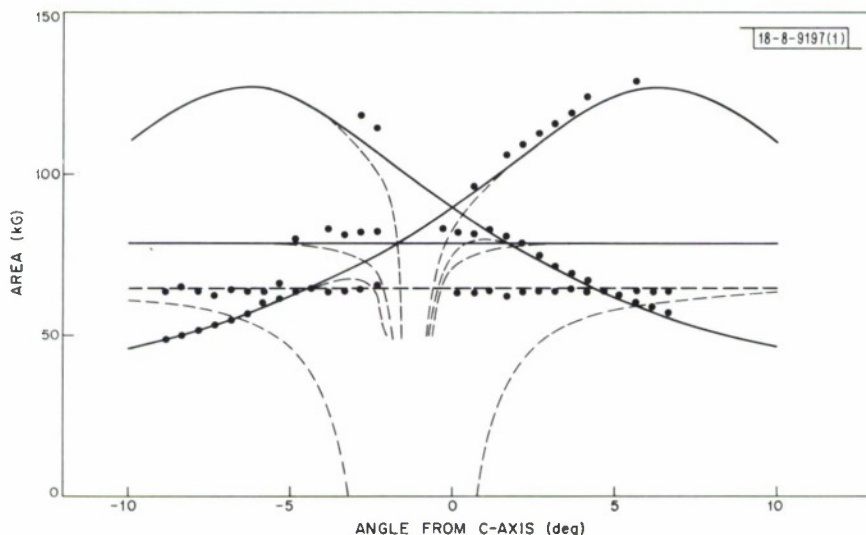
Fig. III-1. Fermi surface cross-sectional area versus angle \theta between magnetic field and trigonal axis. Sound is propagated along binary axis. Solid lines are electron extremal cross sections, and broken line is hole extremal cross section. Dashed lines show nonextremal areas that should be observed according to Ref. 8.
