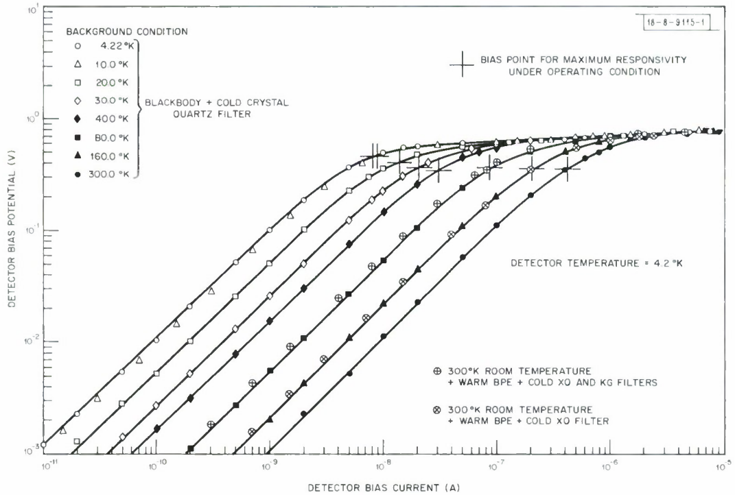
Fig. I-5. Variotien of detector V-I choracteristic with blackbody background temperoture.
