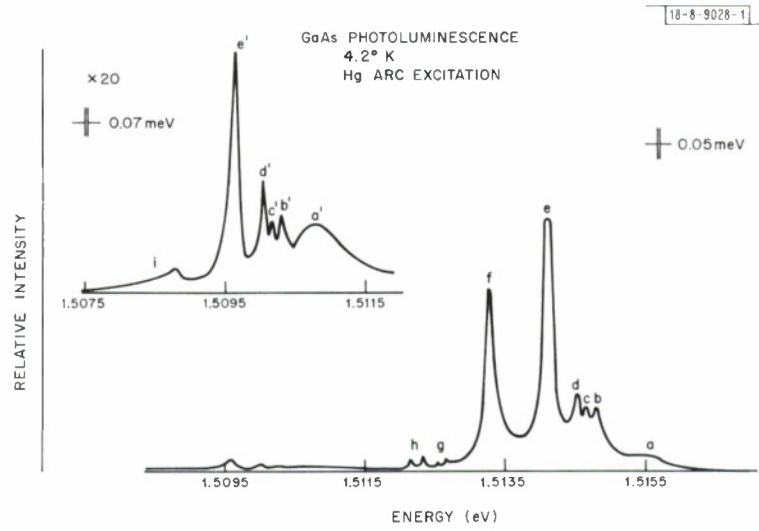
Fig. 1-8. Photoluminescence spectrum of high purity GaAs epitaxial layer ( N_D + N_A = 7.6 \times 10^{13} \text{ cm}^{-3} ). Inset shows repeated scan (at higher gain) of lower energy portion.
