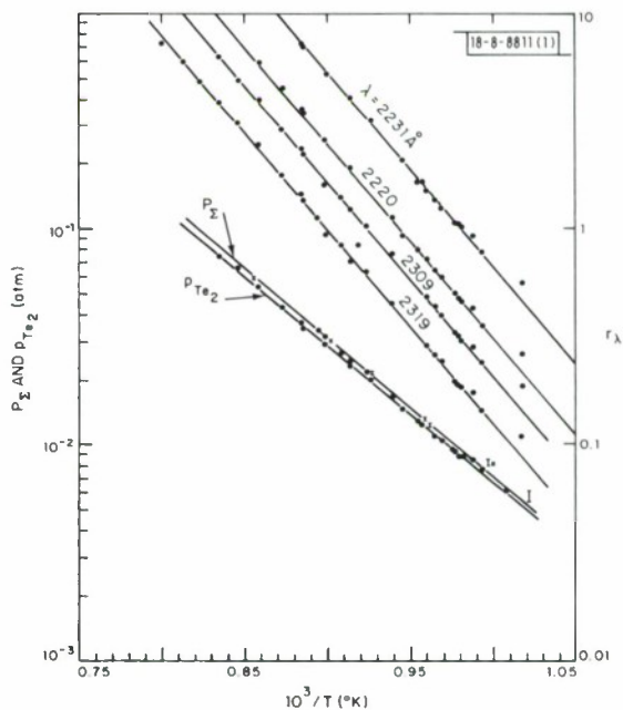
Fig. II-3. Two lowest lines: temperature dependence of total vapor pressure ( P_\Sigma ) and partial pressure of \text{Te}_2 ( p_{\text{Te}_2} ) over \text{Bi}_2\text{Te}_3(\ell) .
