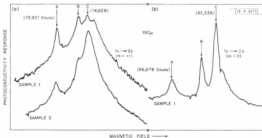
Fig. III-2. Photocurrent signals (bias = 0.5 \mu A) taken with 190- \mu DCN laser as a function of magnetic field: (a) two different samples ( n_1 = 2.0 \times 10^{14} \text{cm}^{-3} and n_2 = 4.3 \times 10^{13} \text{cm}^{-3} ) showing 1s \rightarrow 2p ( m = +1 ) transition; (b) 1s \rightarrow 2p ( m = 0 ) transition taken at higher magnetic fields.
