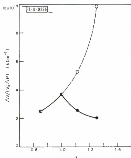
Fig. II-8. Volume compression of TiO_x versus x . Open circles: initial compression (extrapolated to 1 atm). Closed circles: compression at pressures above 20 kbars. Half-closed circles: compression uniform over entire pressure range.
