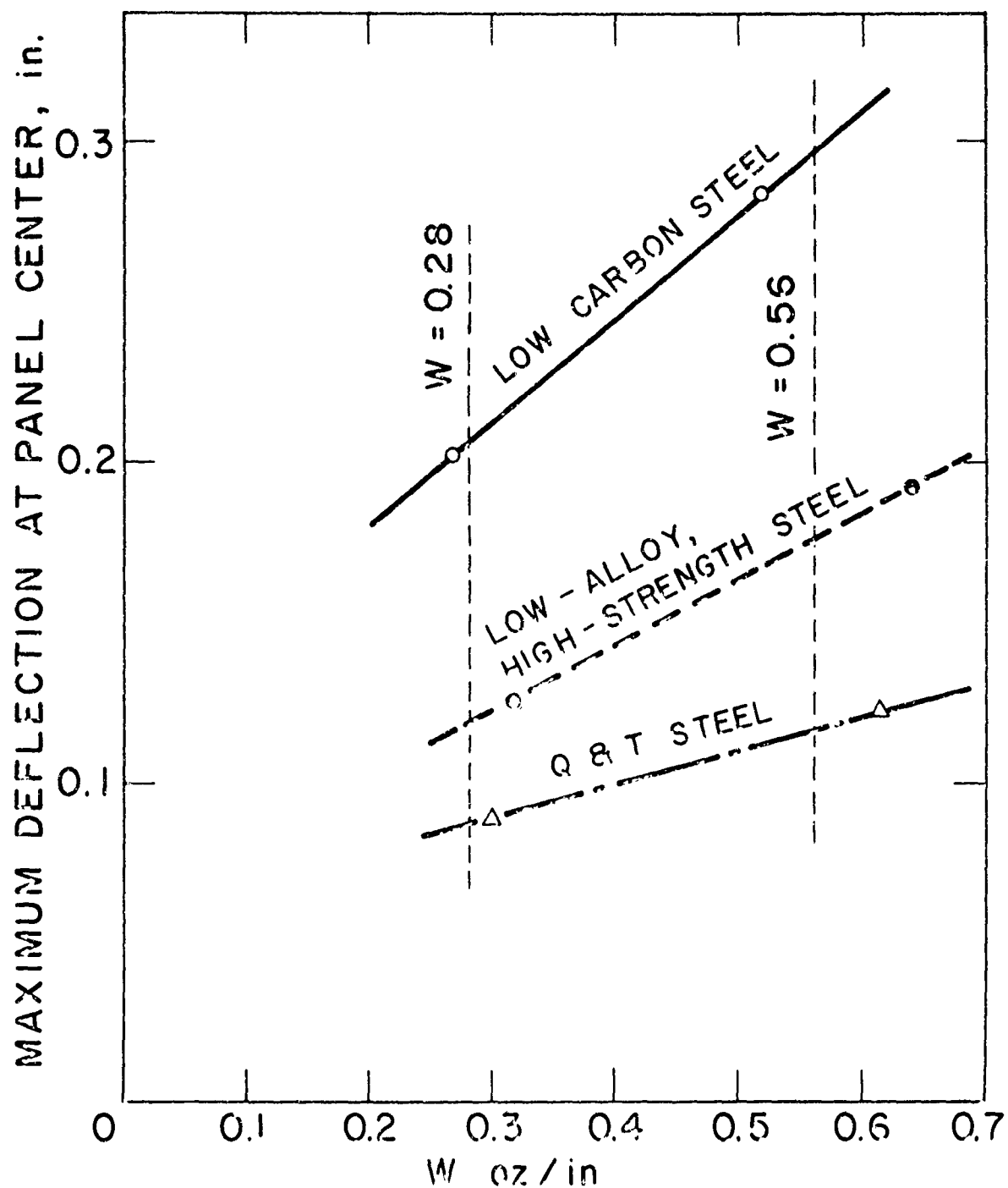
FIGURE 9 RELATIONSHIPS BETWEEN MAXIMUM DEFLECTION AT THE PANEL CENTER AND THE AMOUNT OF ELECTRODES CONSUMED, W (oz/in)
