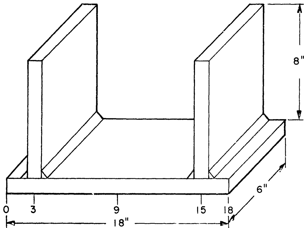
b. SPECIMENS NO. PP-MS-3,4; PP-80-3,4 FIGURE 1 PERPENDICULAR PLATES
