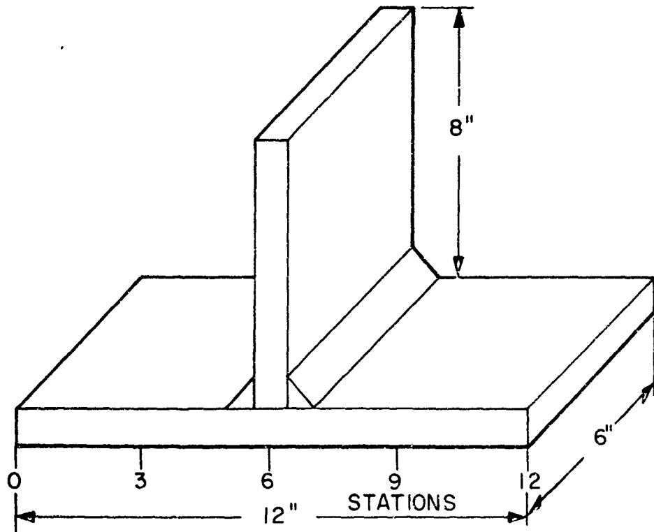
a. SPECIMENS NO. PP-MS-1,2; PP-80-1,2
