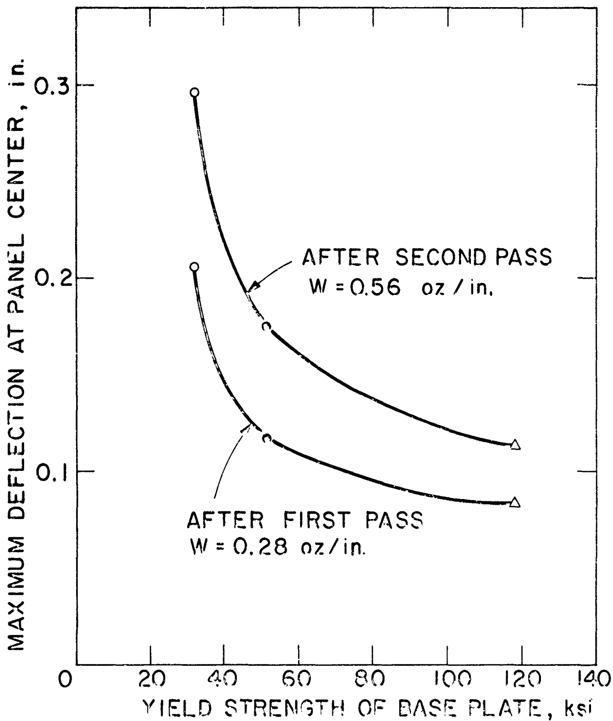
FIGURE 10 RELATIONSHIP BETWEEN THE YIELD STRENGTH OF BASE METAL AND MAXIMUM DEFLECTION AT THE PANEL CENTER
