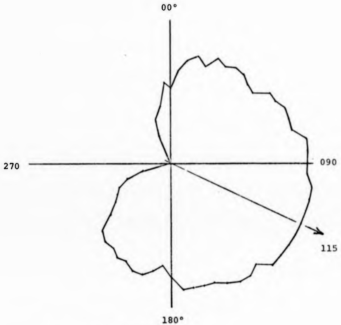
Figure 3.a. Intensity Pattern.
