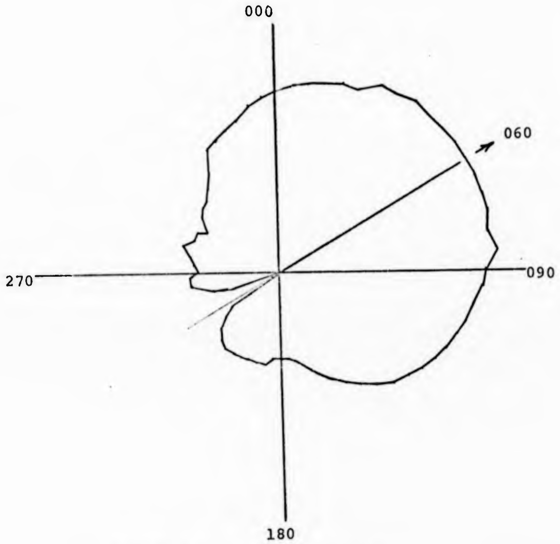
Figure 4.a. Intensity Pattern
