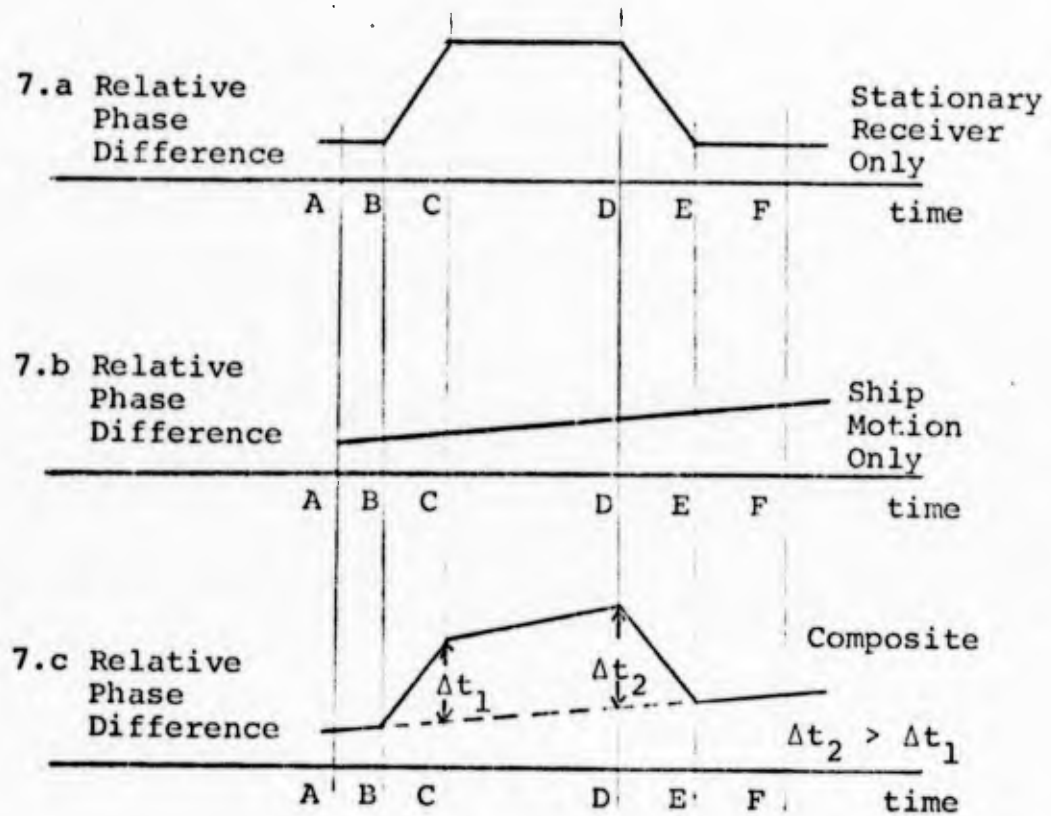
Figure 7. Diurnal Shift with Ship Motion.
