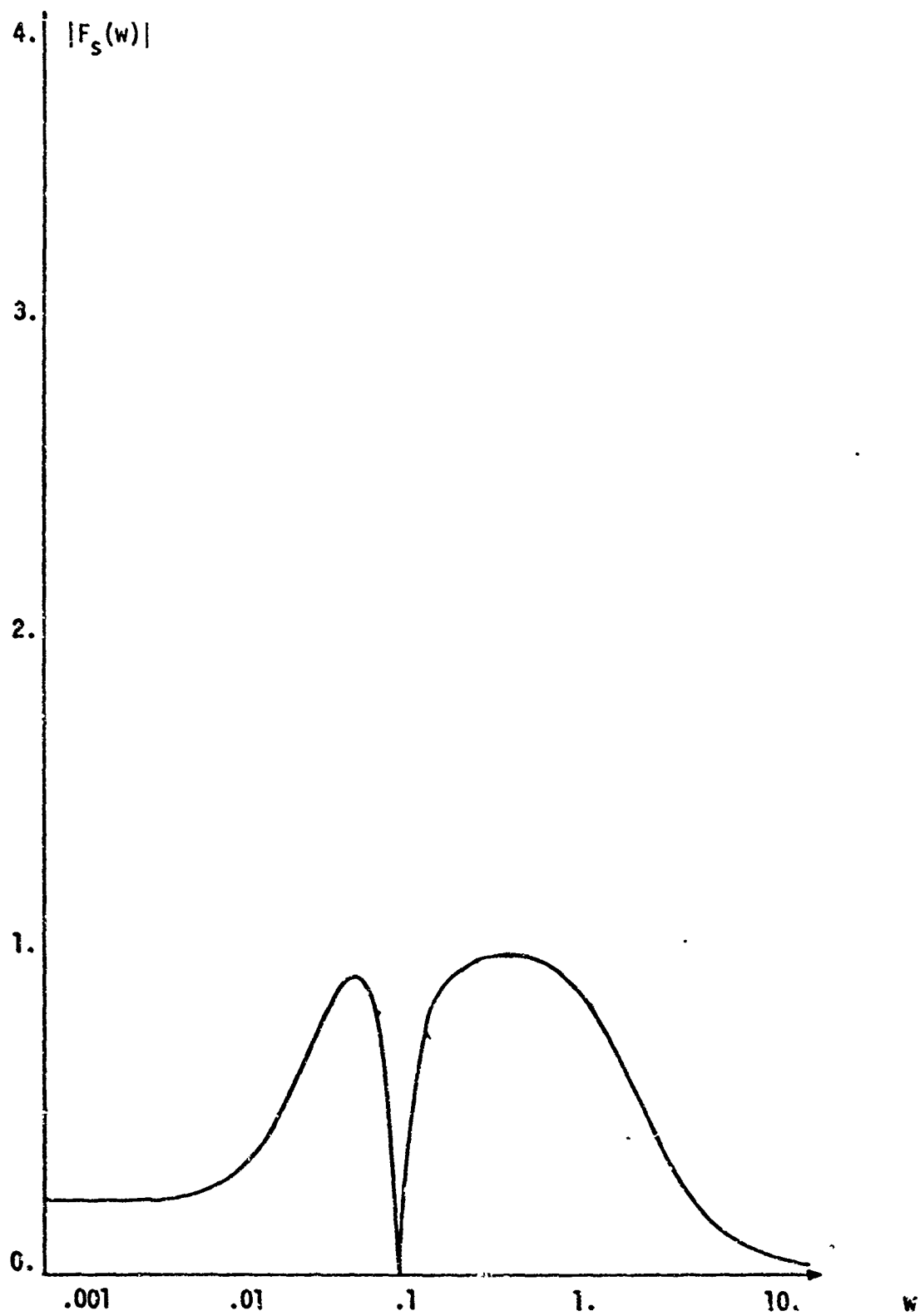
Figure 13. Sensitivity of I_1/V_1 to R_1 .
