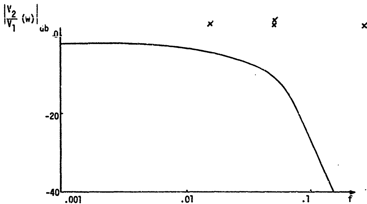
Figure 5. V_2/V_1 , Primary Test Circuit
