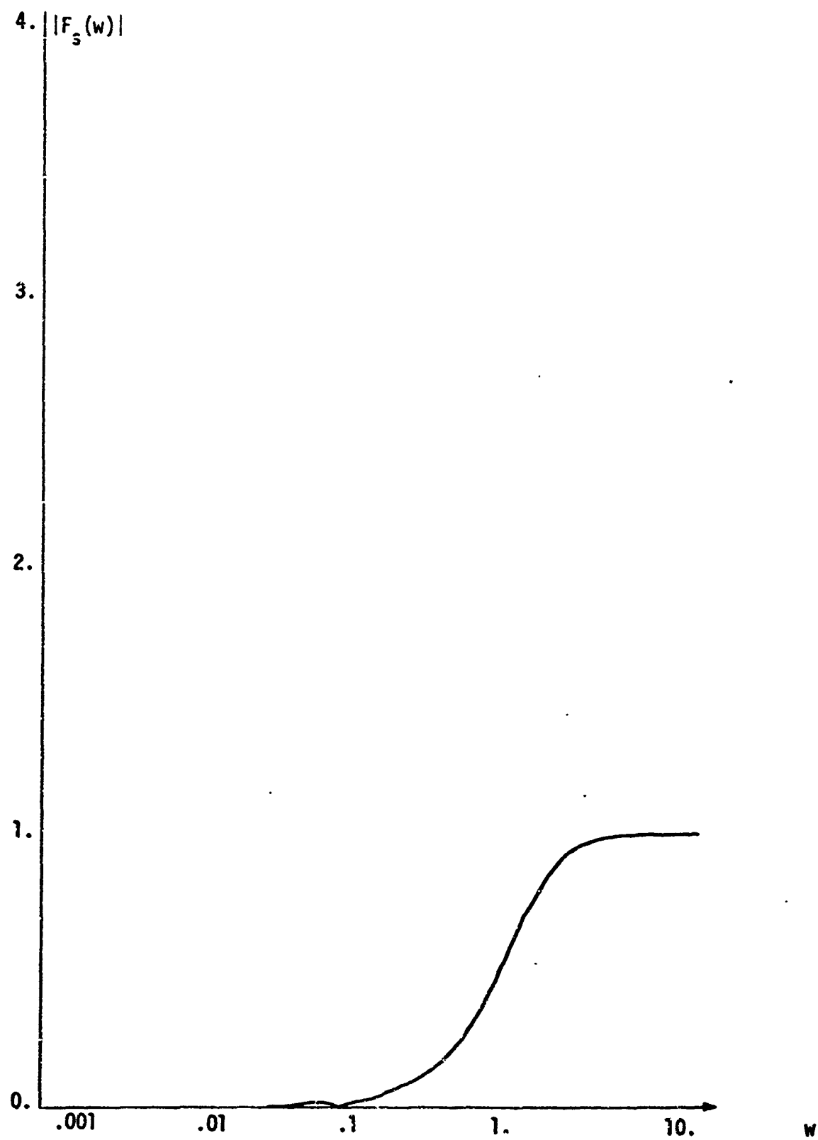
Figure 9. Sensitivity of V_2/V_1 to C_1 .
