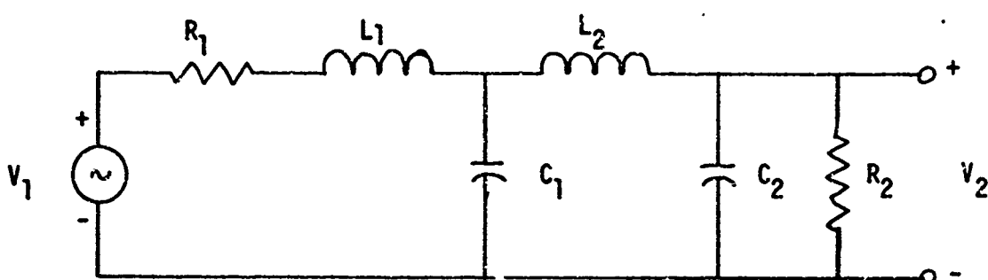
Figure 4. Primary Test Circuit.
