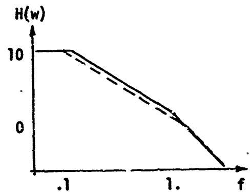
Figure 3c. V_2/V_1 , L_1 Increased.
