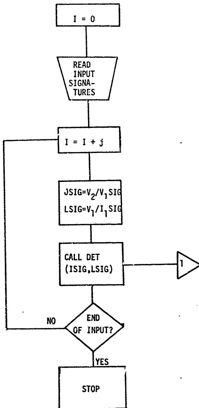
Figure 22. Flowgraph of Main Program for DET
