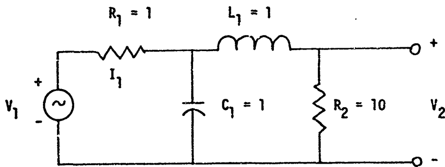
Figure 1. Example 1 - Low Pass Filter
