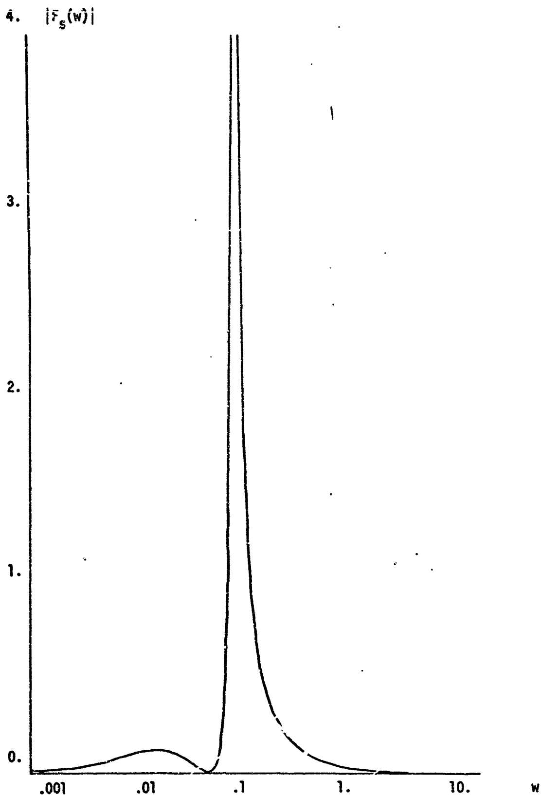
Figure 14. Sensitivity of I_1/V_1 to L_1 .
