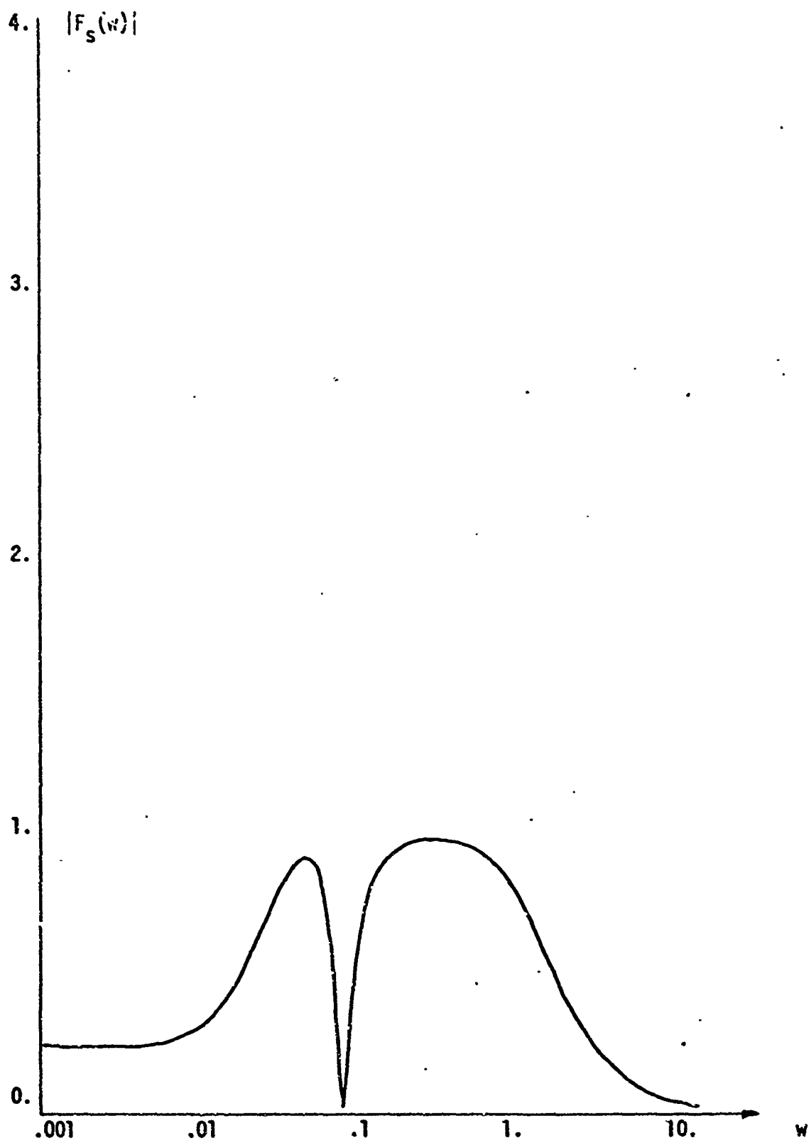
Figure 7. Sensitivity of V_2/V_1 to R_1 .
