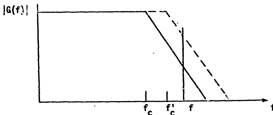
Figure 2. Bode Plot of Simple Pole
