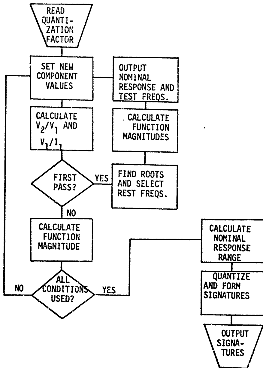
Figure 21. Flowgraph of Primary Analysis Program
