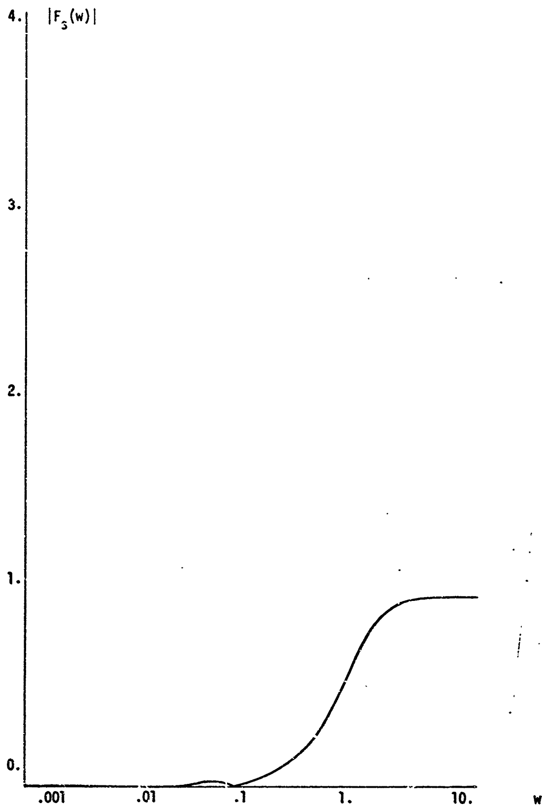
Figure 15. Sensitivity of I_1/V_1 to C_1 .
