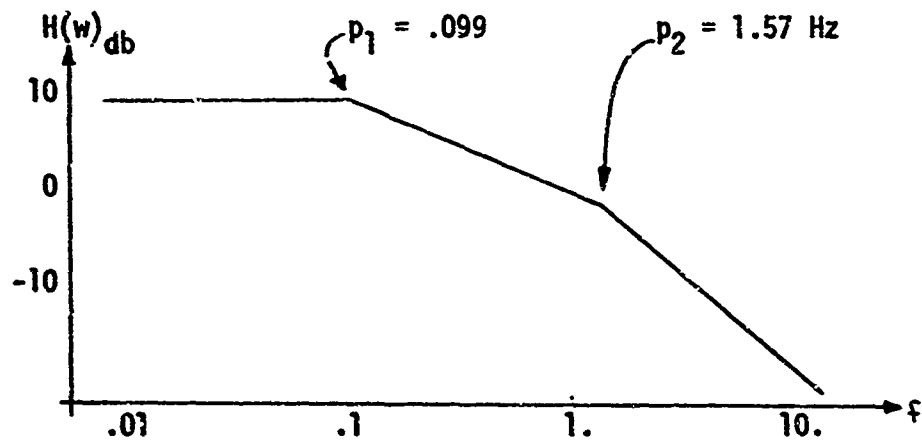
Figure 3a. V_2/V_1 Bode Plot.
