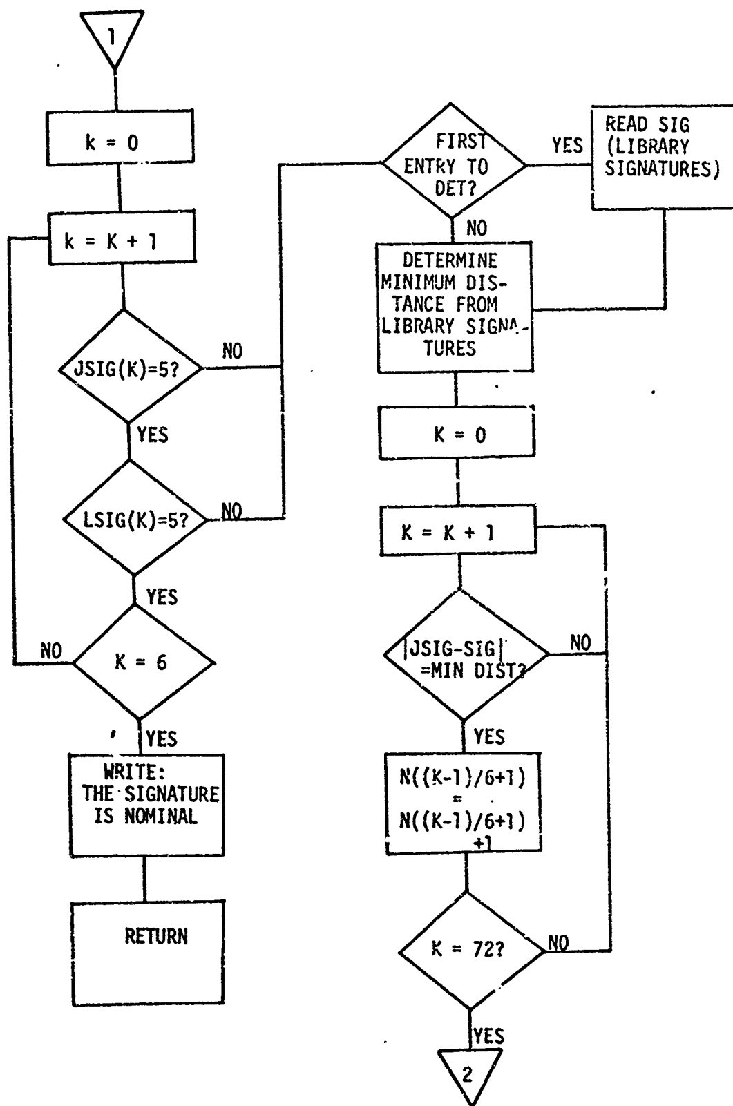
Figure 23. Flowgraph of Subroutine DET
