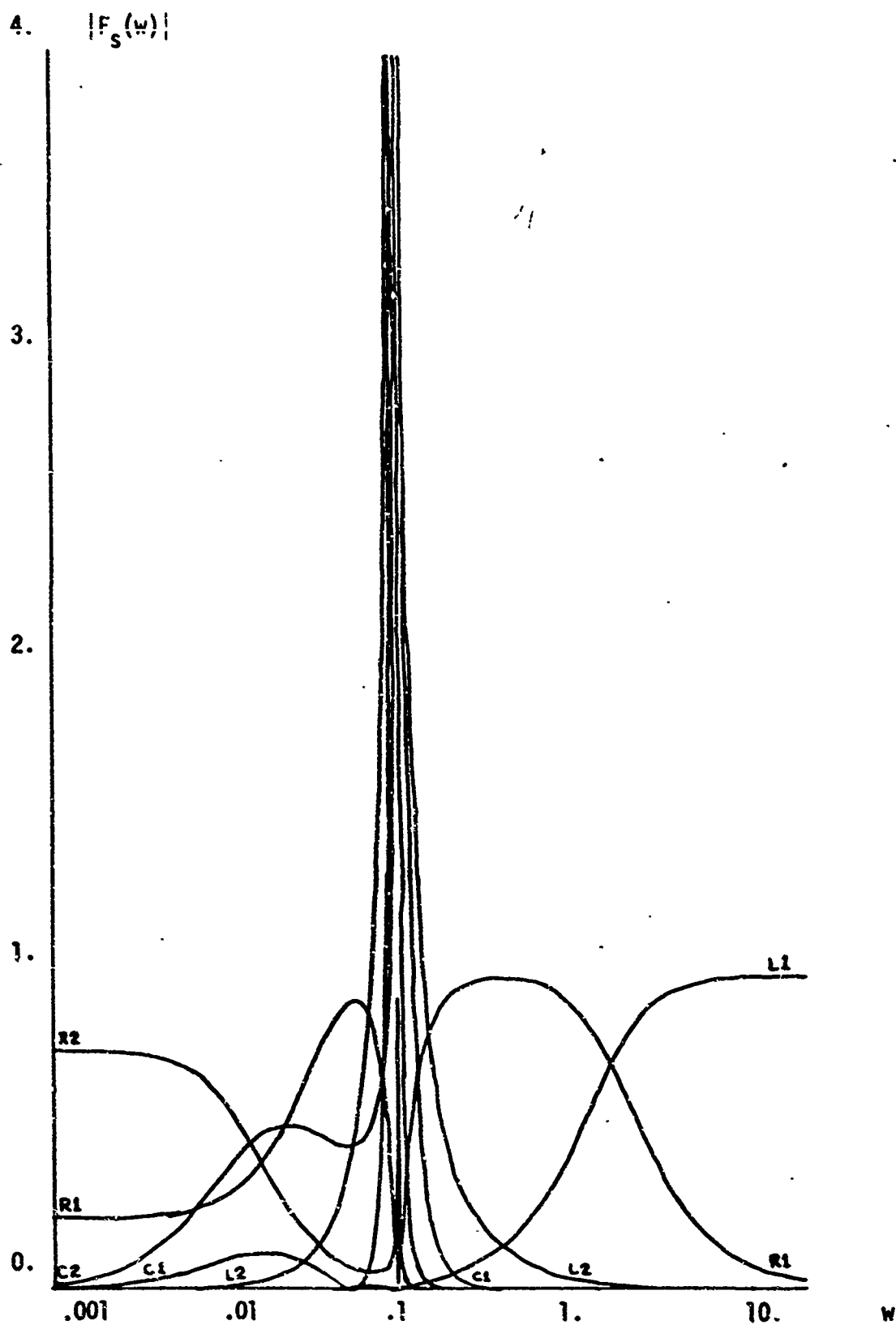
Figure 19. I_1/V_1 Composite Sensitivity Functions.
