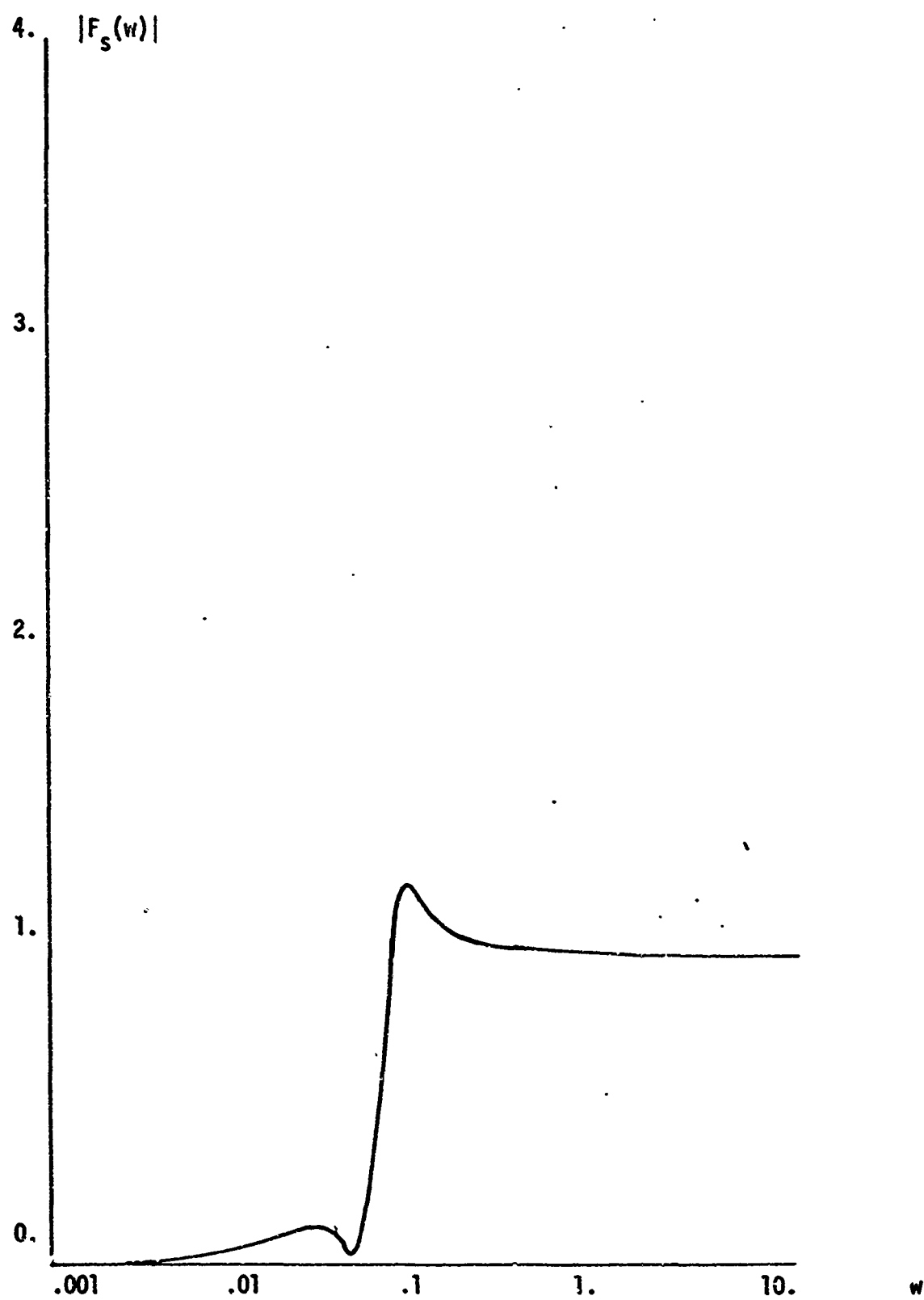
Figure 8. Sensitivity of V_2/V_1 to L_1 .
