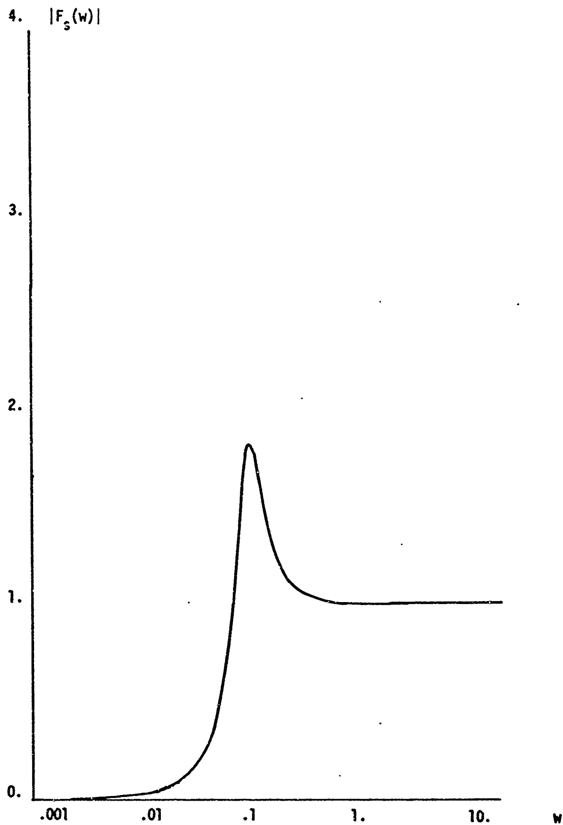
Figure 11. Sensitivity of V_2/V_1 to L_2
