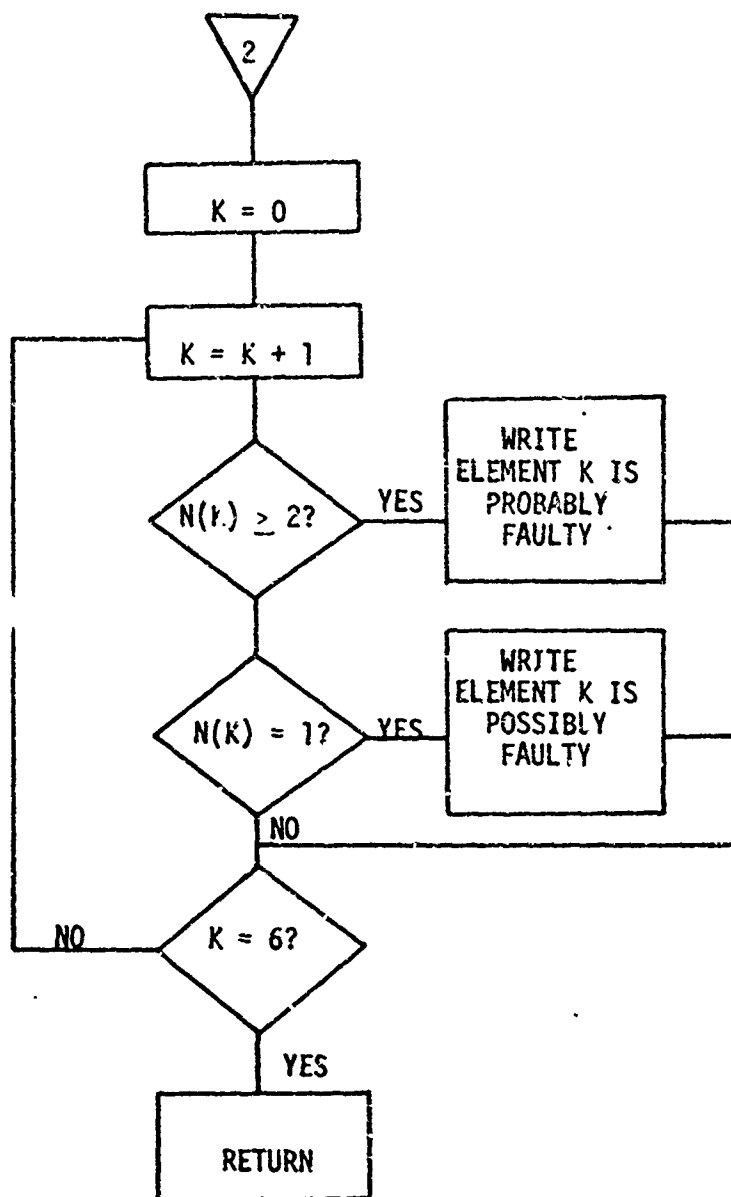
Figure 24. Flowgraph of Subroutine DET (Continued)
