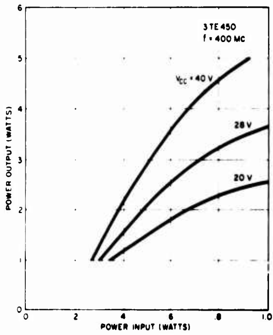
TYPICAL 400 Mc POWER OUTPUT vs POWER INPUT
