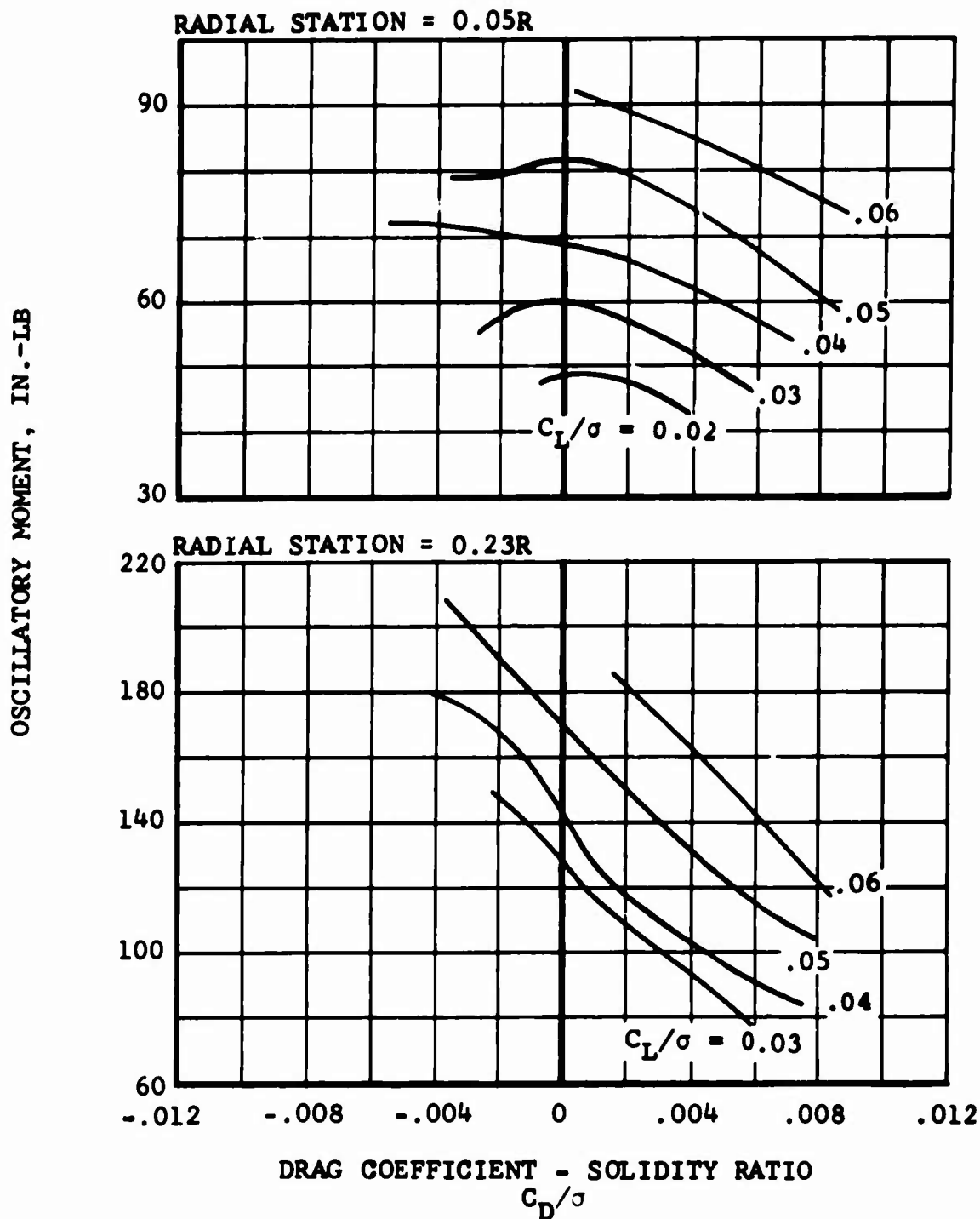
(a) FLAPWISE
