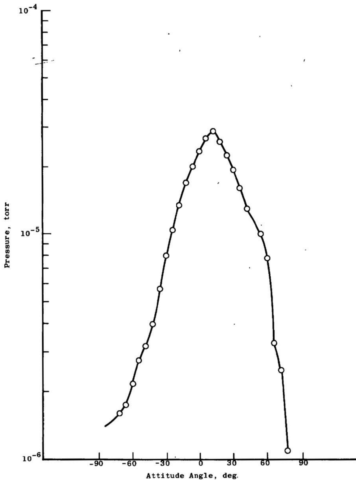
Fig. 12 Pressure Profile for Constant Azimuth
