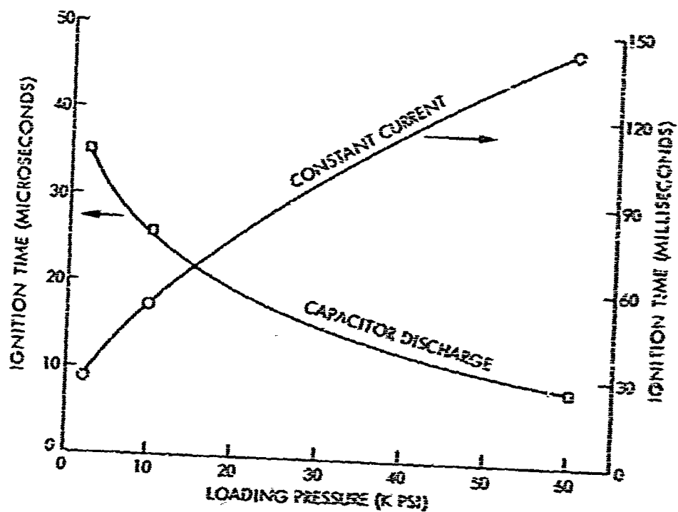
FIG. 4 EFFECT OF LOADING PRESSURE ON IGNITION TIME OF NORMAL LEAD STYRHINATE BY CONSTANT CURRENT AND CAPACITOR DISCHARGE SIGNALS IN THEIR TYPICAL TIME REGIMES
