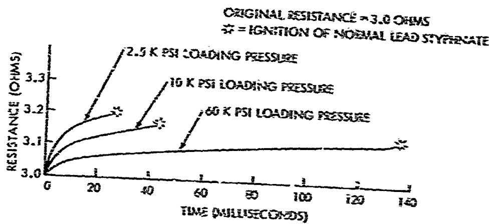
FIG. 5 TYPICAL RESISTANCE CHANGES DURING CONSTANT CURRENT PULSE
