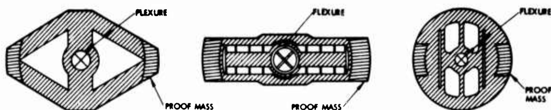
Figure 4-6. Arm designs
