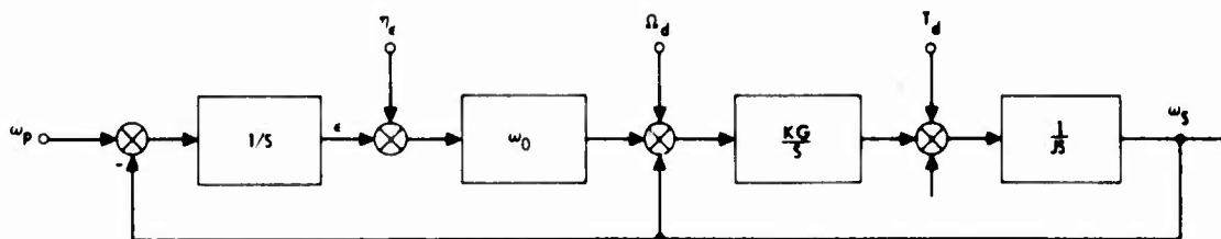
Figure 4-5. Single-axis multiple loop design, simplified block diagram
