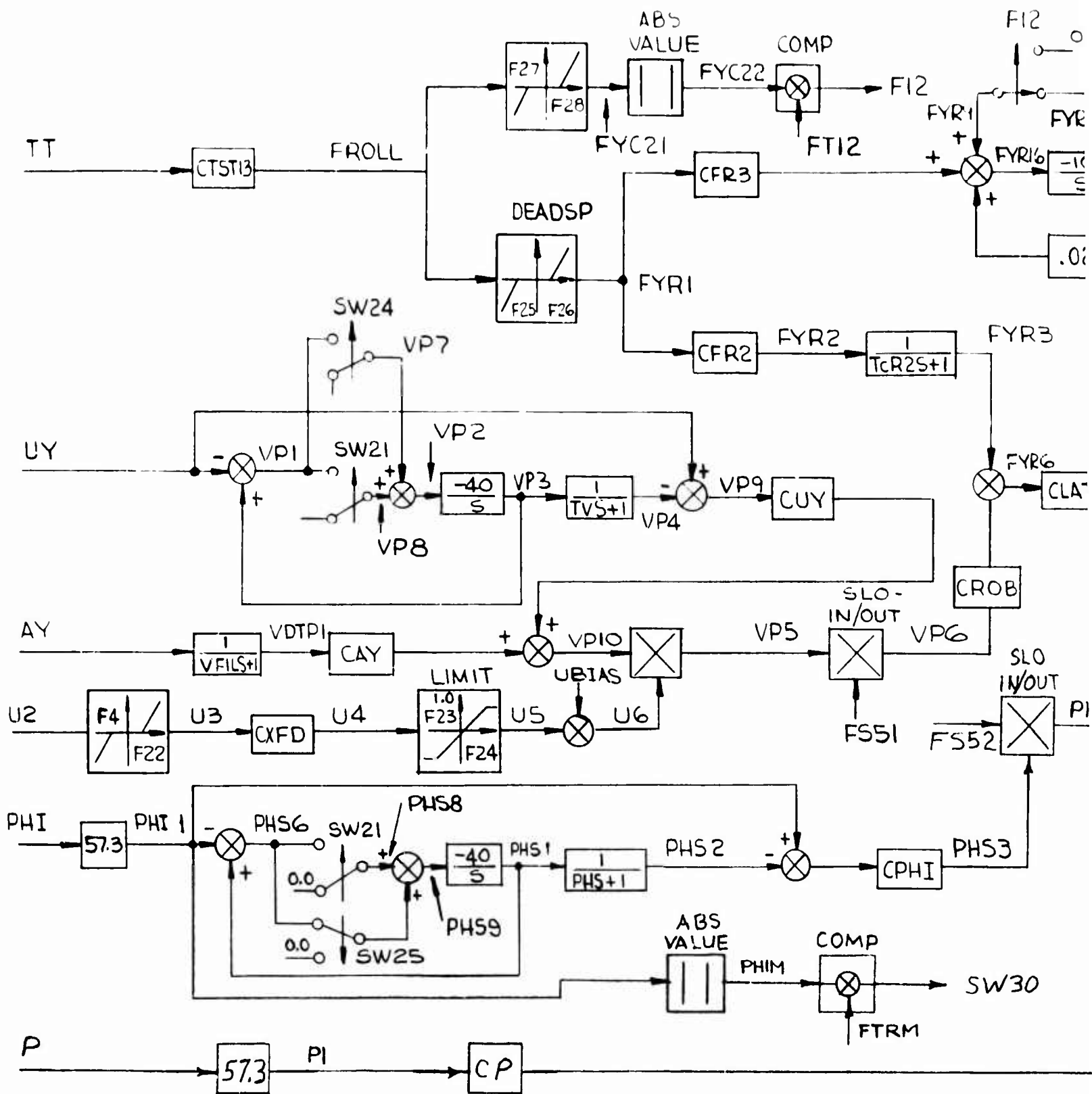
Figure 21. Roll Axis CSMP Diagram.
