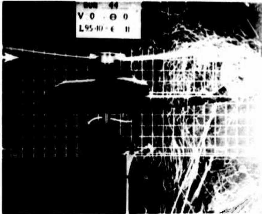
Figure 8. Side Observation of the Distortion of the Main Rotor Wake Through Tail Rotor Wake Ingestion, Out of Ground Effect, in Hover.
