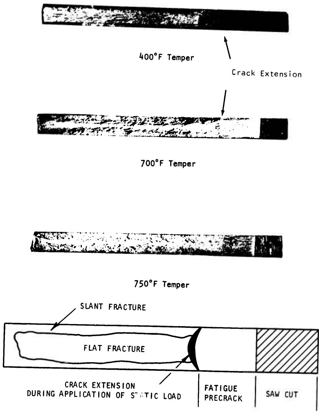
SCHMATIC OF CRACK SURFACE
