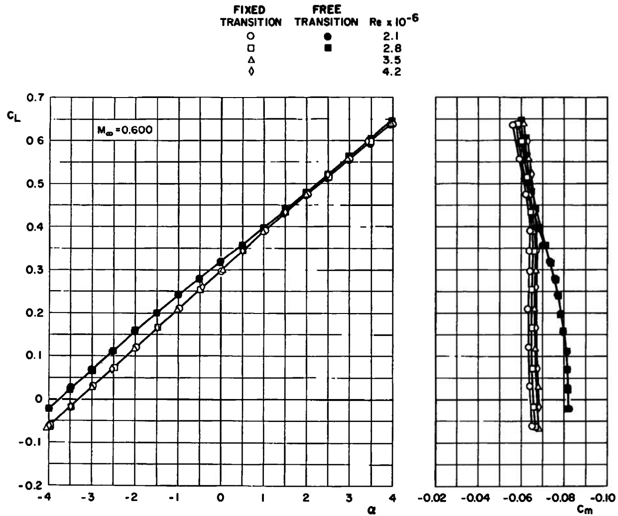
Fig. 9 Effects of Reynolds Number Variation on the Aerodynamic Coefficients of the Wing-Fuselage Configuration at Mach Numbers from 0.600 to 0.825
