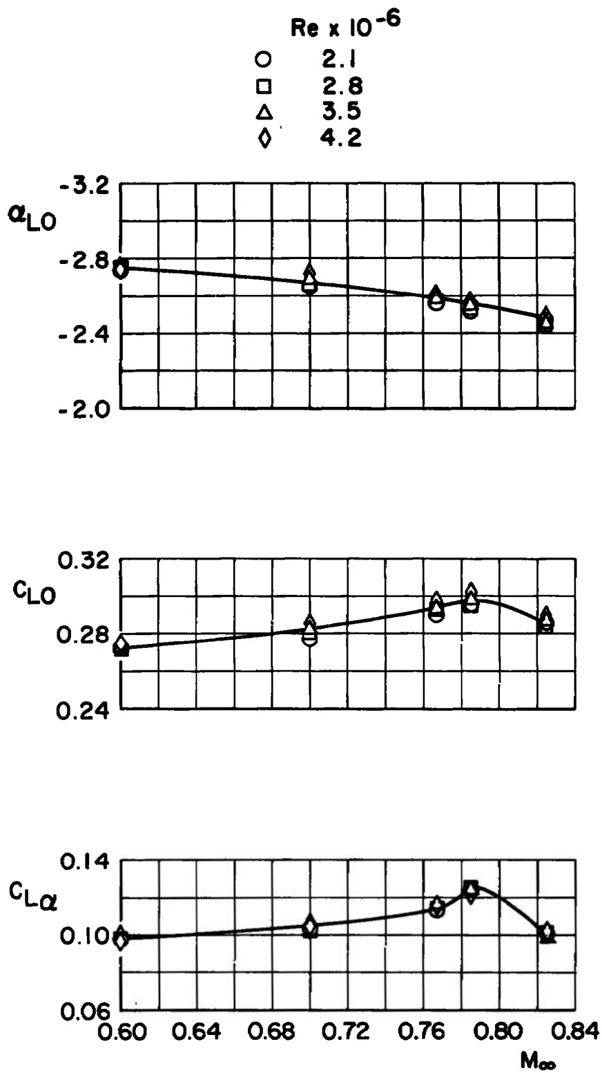
Fig. 14 Variation of \alpha_{L0} , C_{L0} , and C_{L\alpha} with Mach Number for the Wing-Fuselage-Tail Configuration
