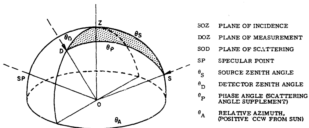
Figure 12. Geometry for Reflectance Measurement
