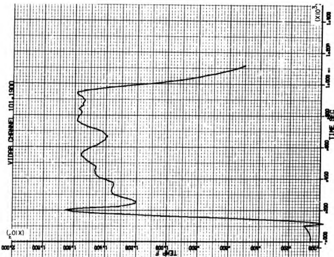
FIGURE 18 TIME TEMPERATURE PLOT OF THERMOCOUPLE (7) ON MK 379
