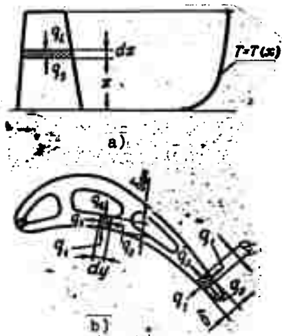
Fig. 2. Taking into consideration of longitudinal flows of heat during the calculation of temperatures in a transverse cross section by the ETA method: a) the change in a temperature over the height of the blade; b) the transverse cross section of a blade at a distance x from the root.
