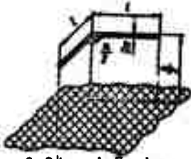
Fig. 3-24. A \Gamma -shaped wire, parallel to an impenetrable boundary.
