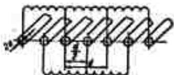
Fig. 3-43. 2n loaded wires of alternating polarity lying in one plane.
