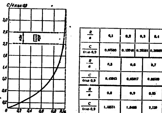
Fig. 5-51. Graph for determination of capacitance between an infinitely long shell of circular section and a circular disc inside it (dotted line — extrapolation).
