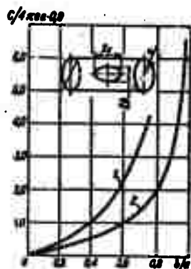
Fig. 5-66. A graph for determination of the capacitance of a spheroid inside an infinitely long cylinder: 1 - drawn out (the ratio of axes 1/2); 2 - condensed (ratio of axes 2/1); dotted line - extrapolation.
