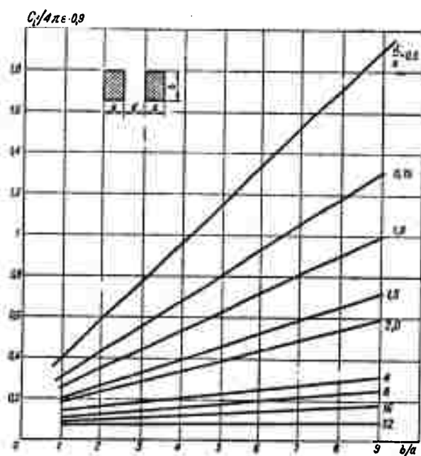
Fig. 5-32. A graph for determining capacitance per unit of length between two rectangular shells.
