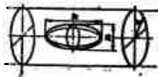
Fig. 5-65. A spheroid inside an infinitely long cylinder.
