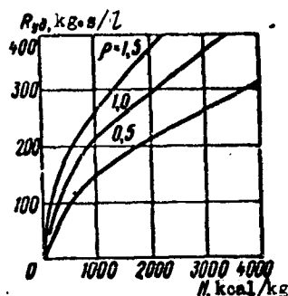
Fig. 69. Dependence of the specific thrust of a liquid fuel rocket engine on the heat of combustion and the density of the propellant.
