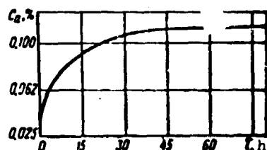
Fig. 103. Change in the content of asphaltenes in the oil during the operation of a piston engine.
