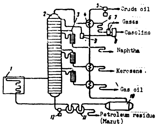
Fig. 1. Line diagram of a tubular installation with a one-time vaporization for the direct distillation of oil.
