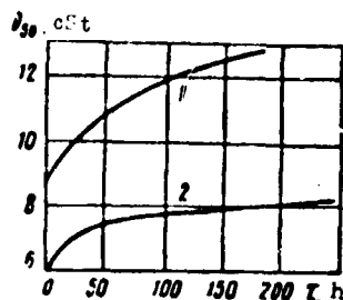
Fig. 96. Change in the viscosity of oil in the process of its operation in an engine: 1 - MK-8; 2 - MK-6.
