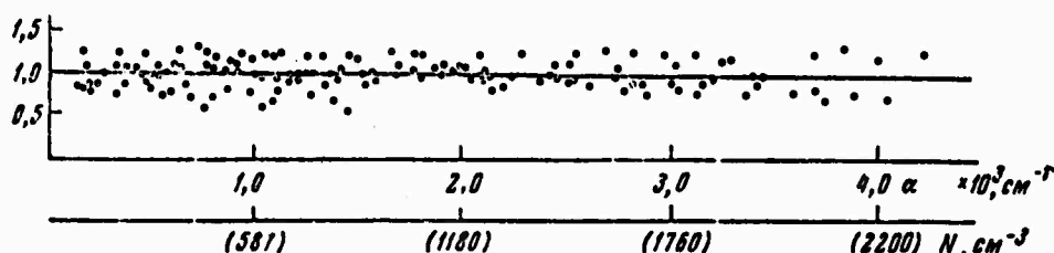
Fig. 1. Calculated vs. measured attenuation factor for laser propagation in fog.
