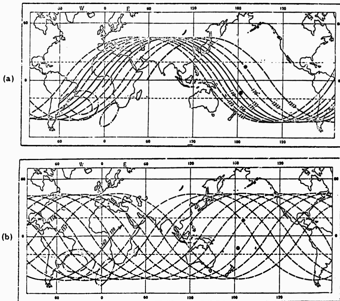
Fig. 1. Trajectory of Kosmos-3 (a) and Kosmos-6 (b).
