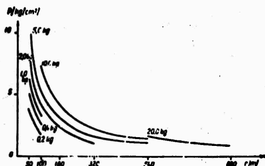
Fig. 1. Pressure vs. distance for various charge sizes.
