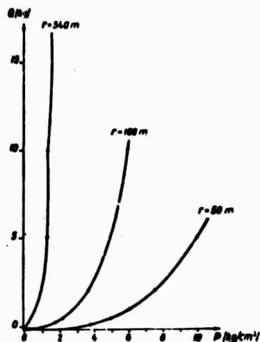
Fig. 2. Pressure vs. charge size at various recording ranges.
