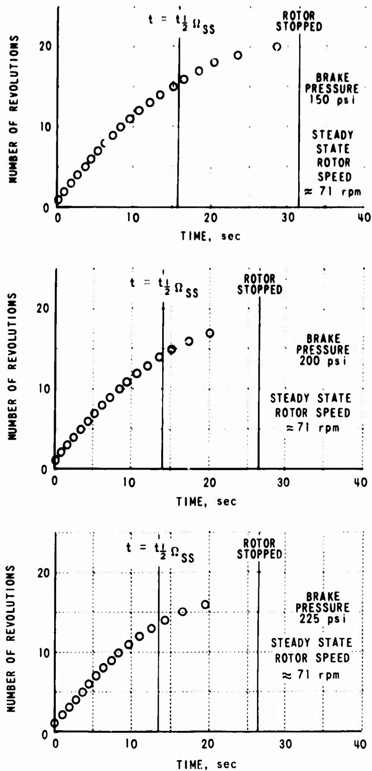
Figure 31. TIME HISTORIES OF NUMBER OF ROTOR REVOLUTIONS FROM BRAKE APPLICATION TO STOP AT A FREESTREAM VELOCITY OF 140 FPS EMPLOYING SEVERAL DIFFERENT BRAKE PRESSURES.
