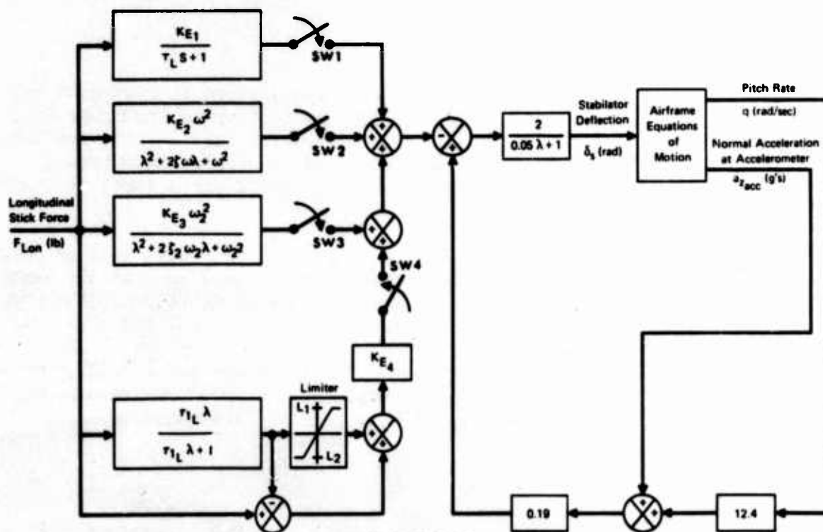
FIGURE 13 LONGITUDINAL FLIGHT CONTROL SYSTEM
