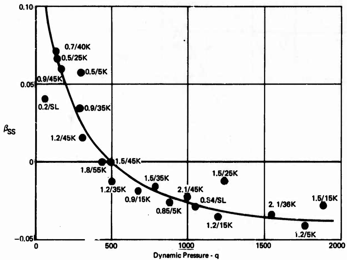
FIGURE 45 SIDSLIP VARIATION WITH DYNAMIC PRESSURE
