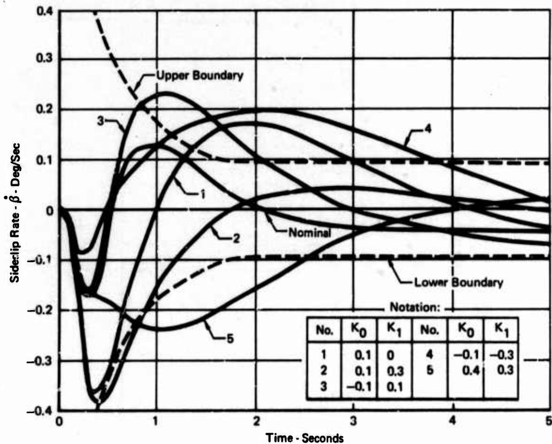
FIGURE 25 TIME HISTORY RESPONSE TRACES FOR ADVERSE/PROVERSE YAW CONFIGURATIONS WITH AILERON STEP INPUT
