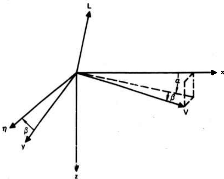
FIGURE 50 WIND AXIS COORDINATES ( V, \eta, L ) WITH RESPECT TO THE BODY AXIS COORDINATES ( x, y, z )
