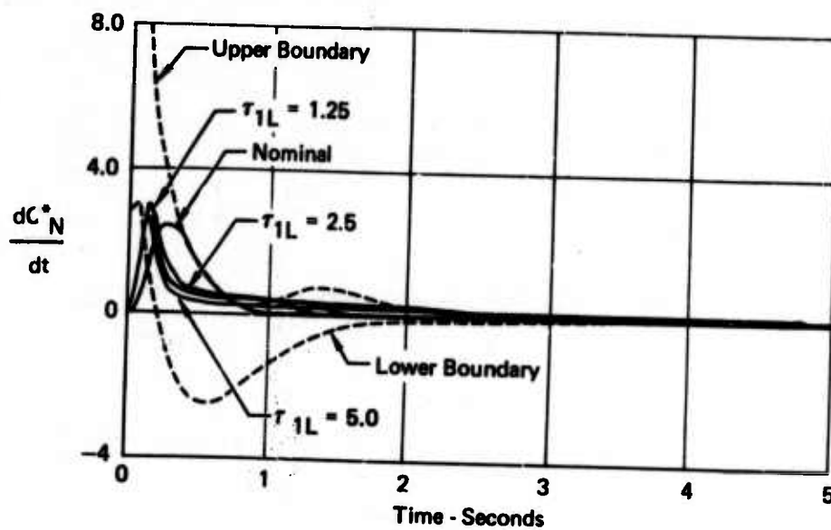
FIGURE 19 LONGITUDINAL TIME HISTORY RESPONSE TRACES FOR NONLINEAR PREFILTER CONFIGURATIONS
