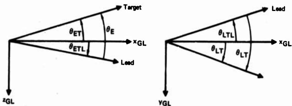
FIGURE 53 GEOMETRY OF THE ELEVATION AND LATERAL TRACKING ERRORS WITH RESPECT TO THE GUNLINE
