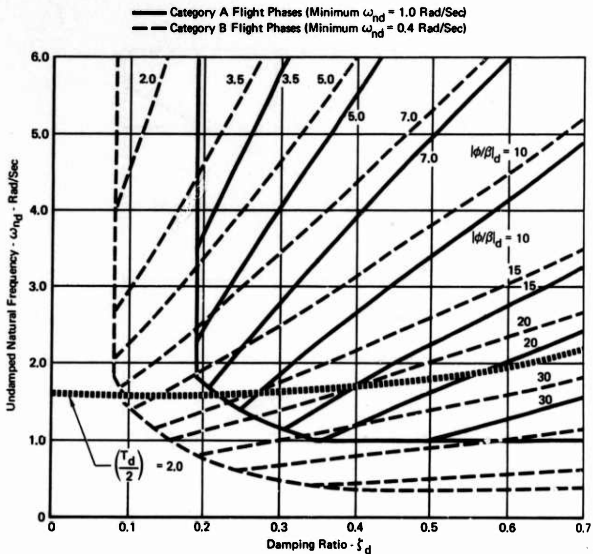
FIGURE 6 DUTCH ROLL FREQUENCY AND DAMPING REQUIREMENTS (CLASS IV, CATEGORY A AND B, LEVEL 1)
