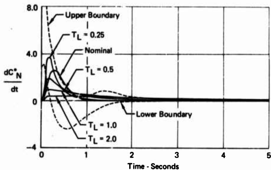
FIGURE 18 LONGITUDINAL TIME HISTORY RESPONSE TRACES FOR PREFILTER TIME CONSTANT CONFIGURATIONS
