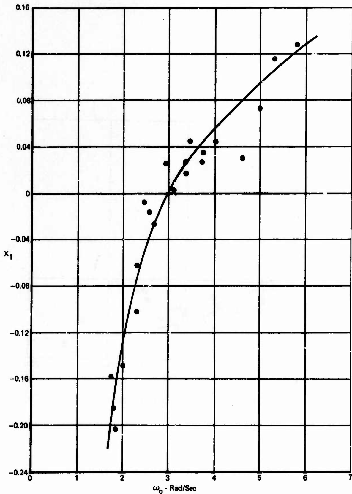
FIGURE 44 COUPLING PARAMETER RELATIONSHIP TO DUTCH ROLL FREQUENCY
