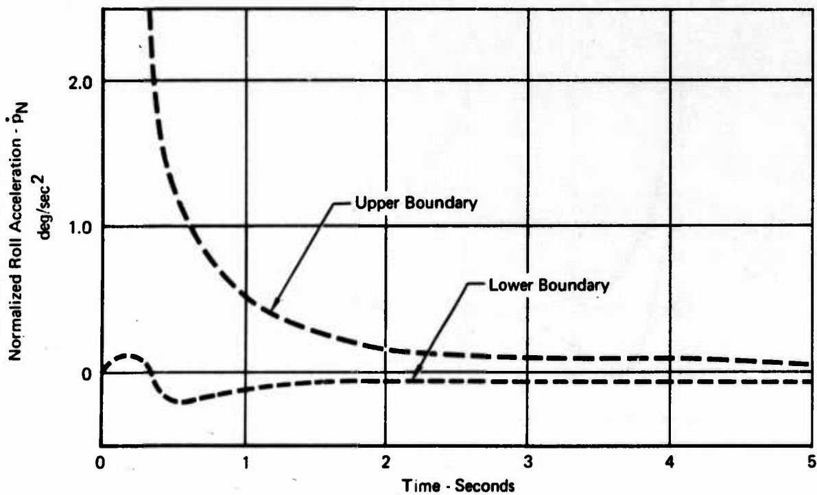
FIGURE 38 SFCS ROLL AXIS TIME HISTORY CRITERION
