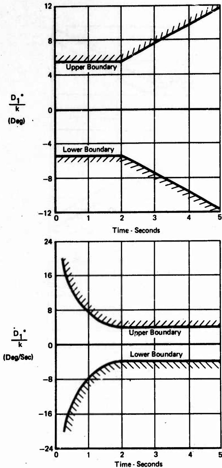
FIGURE 40 SFCS YAW AXIS TIME HISTORY CRITERION
