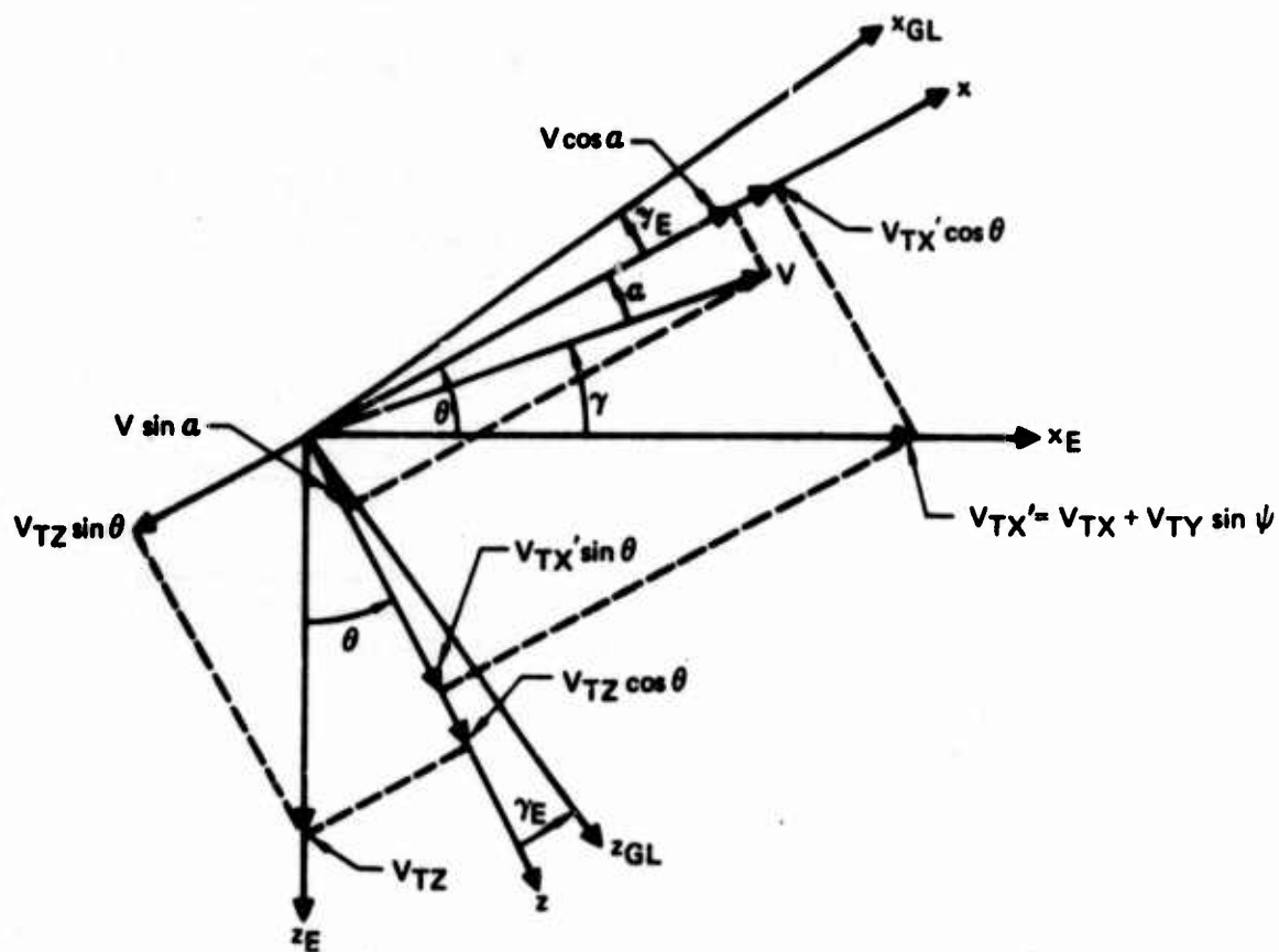
FIGURE 52 GEOMETRY OF THE RELATIVE VELOCITY VECTOR
