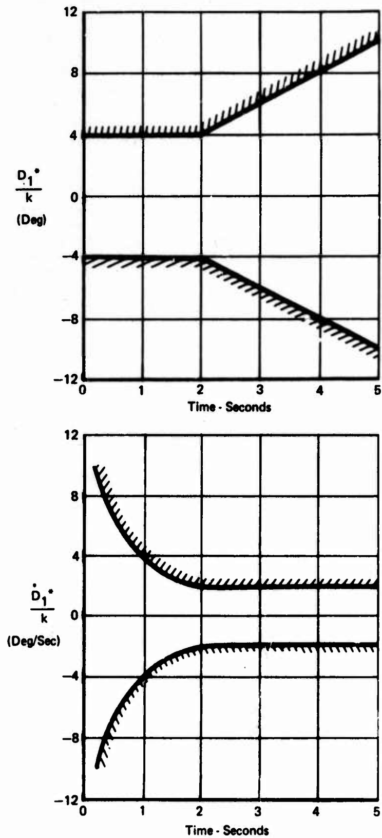
FIGURE 9 DIRECTIONAL TIME HISTORY CRITERION FOR LATERAL STICK FORCE INPUT
