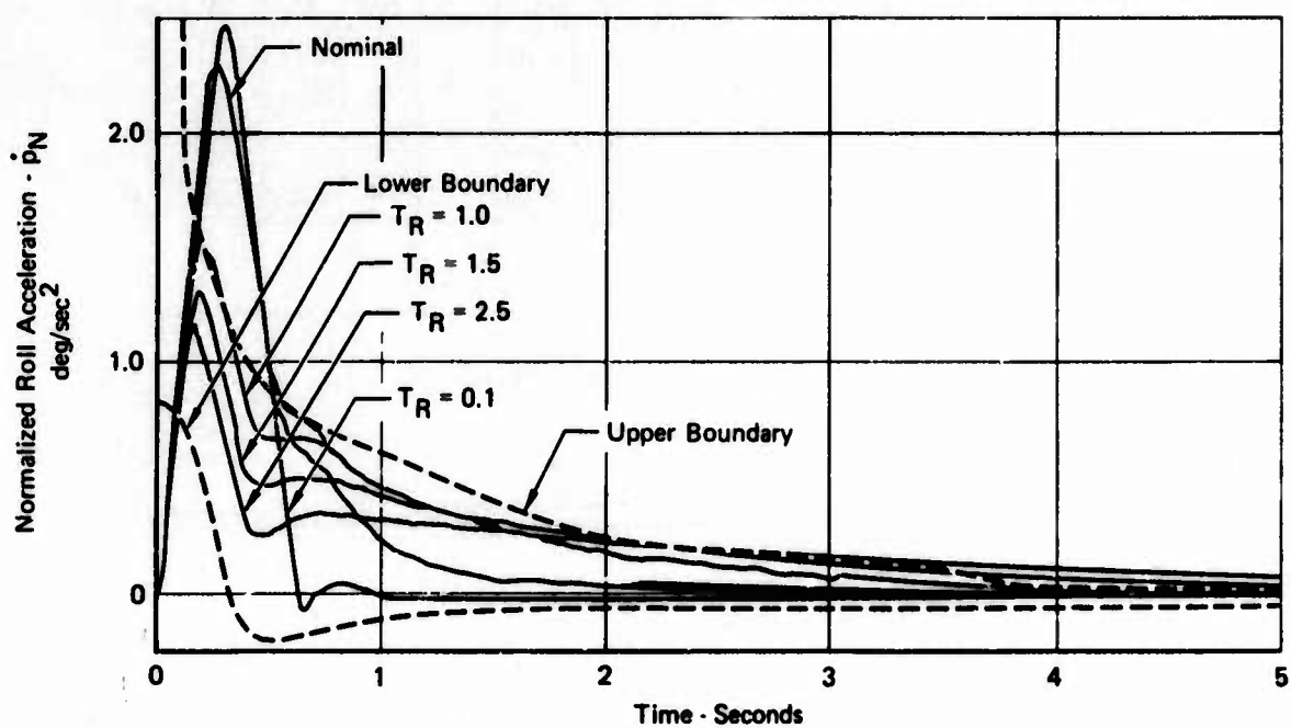
FIGURE 21 LATERAL DIRECTIONAL TIME HISTORY RESPONSE TRACES FOR ROLL TIME CONSTANT CONFIGURATIONS WITH AILERON STEP INPUT
