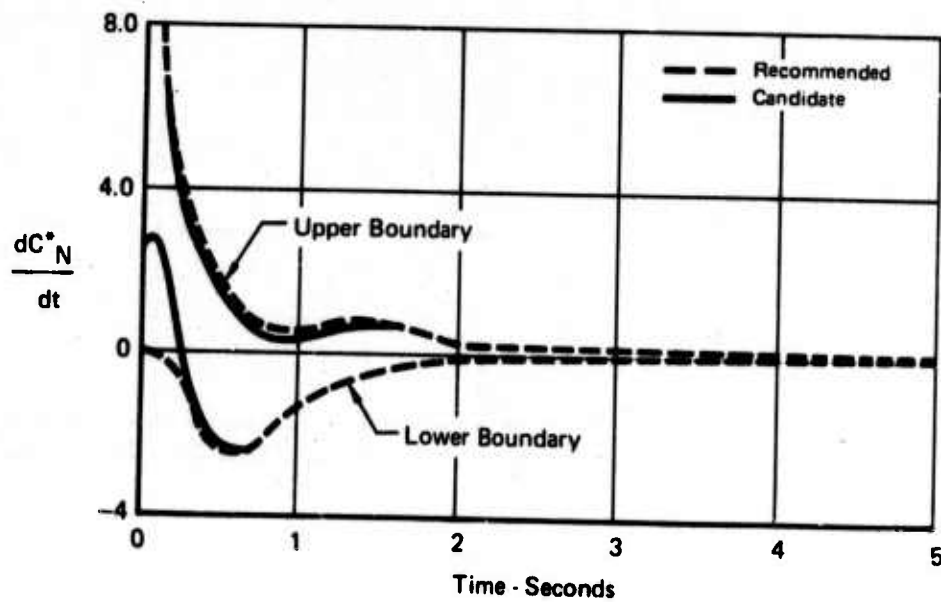
FIGURE 37 SFCS PITCH AXIS TIME HISTORY CRITERION
