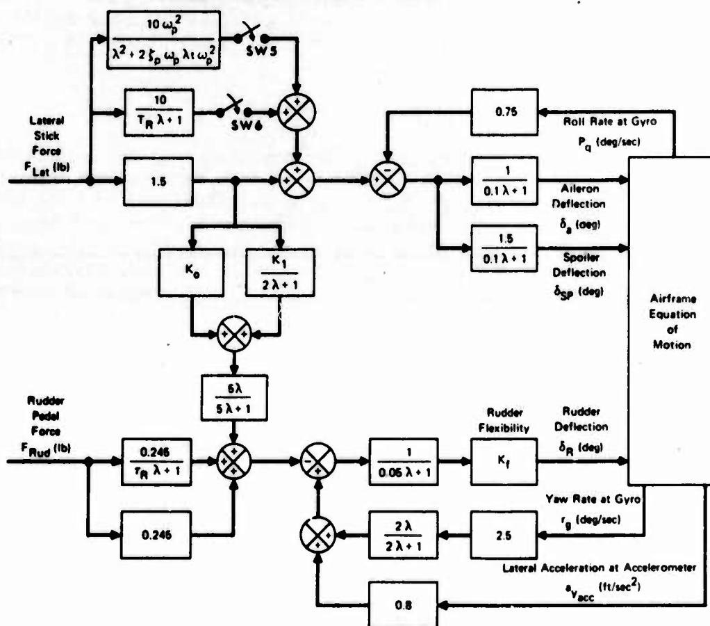
FIGURE 14 LATERAL DIRECTIONAL FLIGHT CONTROL SYSTEM
