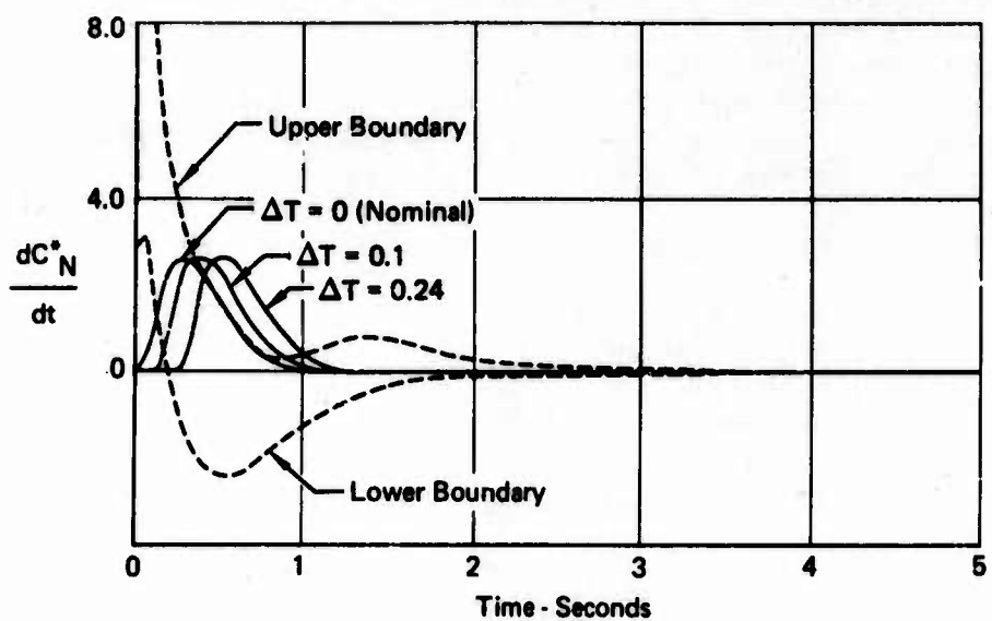
FIGURE 17 LONGITUDINAL TIME HISTORY RESPONSE TRACES FOR TIME DELAY CONFIGURATIONS
