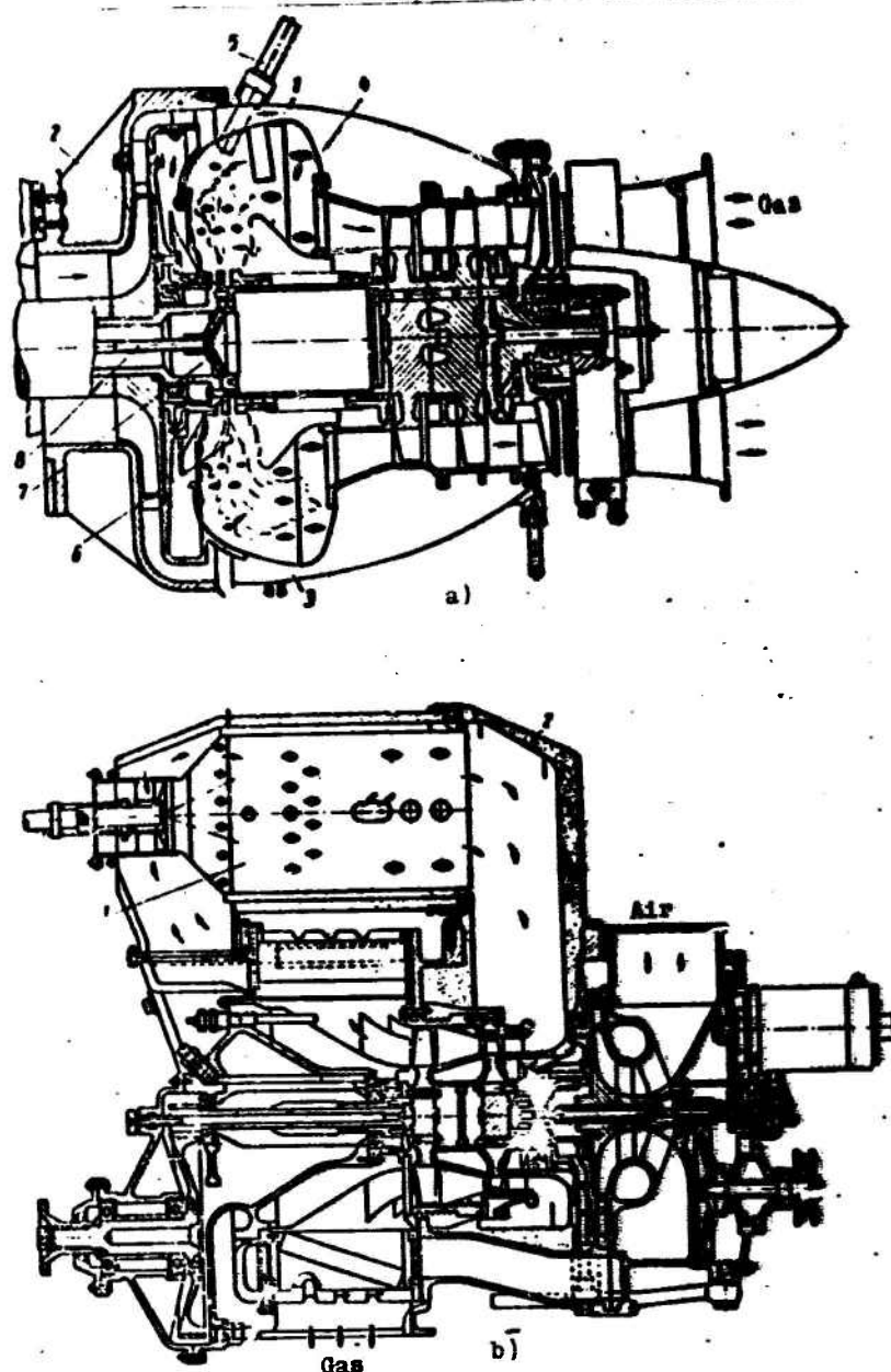
Fig. 69. Diagrams of GTD: a) marine with annular combustion chamber; b) of a sea-going launch with individual combustion chamber.
