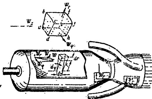
Fig. 2.1. Diagram of the element of burning flow in the internal cavity of the combustion chamber.
