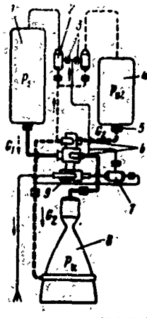
Fig. 1.1. Open configuration of liquid-propellant rocket engine "liquid-liquid": 1, 4 - tanks; 2 - generator (mixer) for tank pressurization; 3 - pressurizing throttle; 5 - component feed valve; 6 - bipropellant pump; 7 - gas generator; 8 - combustion chamber with nozzle; 9 - turbine of turbo-pump assembly; — - main lines; - - - additional lines.
