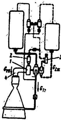
Fig. 1.2. Closed configuration of liquid-propellant rocket engine "liquid-gas": 1 - centrifugal turbine; 2 - bi-propellant gas generator; 3 - propellant component flow rate regulator; 4 - exhaust turbogas (afterburning) pipe.
