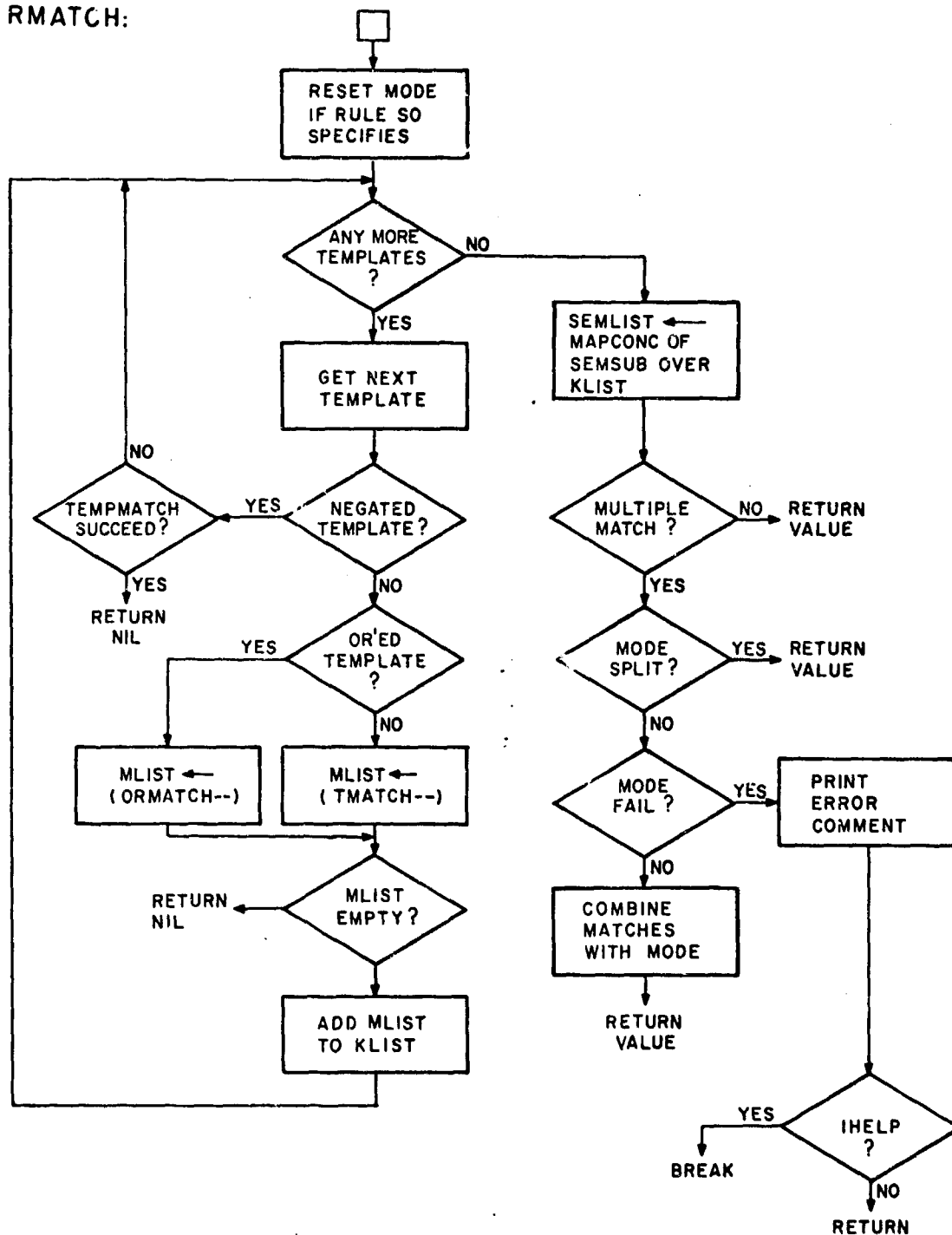
Figure 2-8. The Function RMATCH
