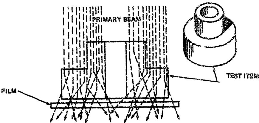
Figure 16. Internal Scatter
