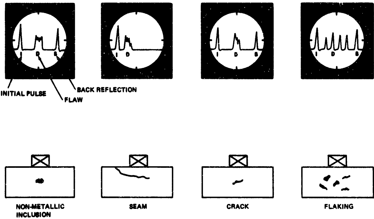
Figure 44. Typical Contact Test Flaw Indications
