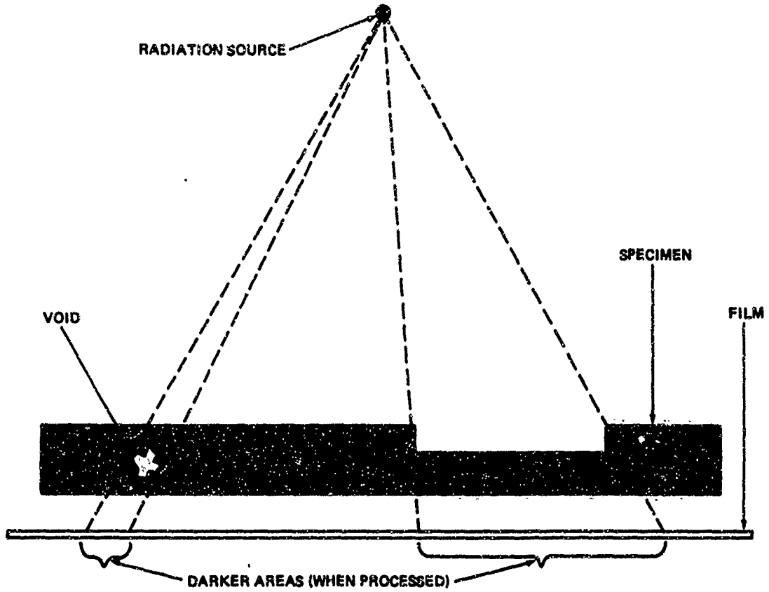
Figure 11. Basic Radiographic Process Showing Differential Absorption
