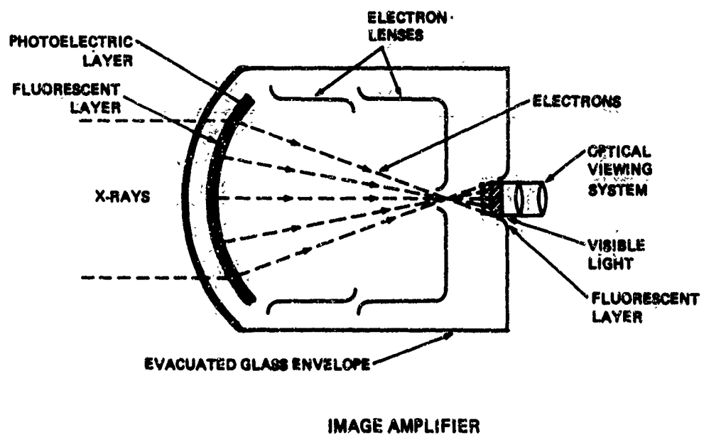
Figure 28. Fluoroscopy Equipment
