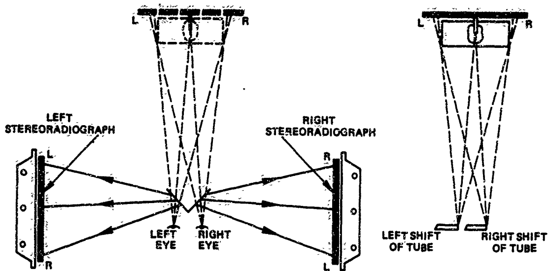
Figure 30. Stereoscopic Radiography
