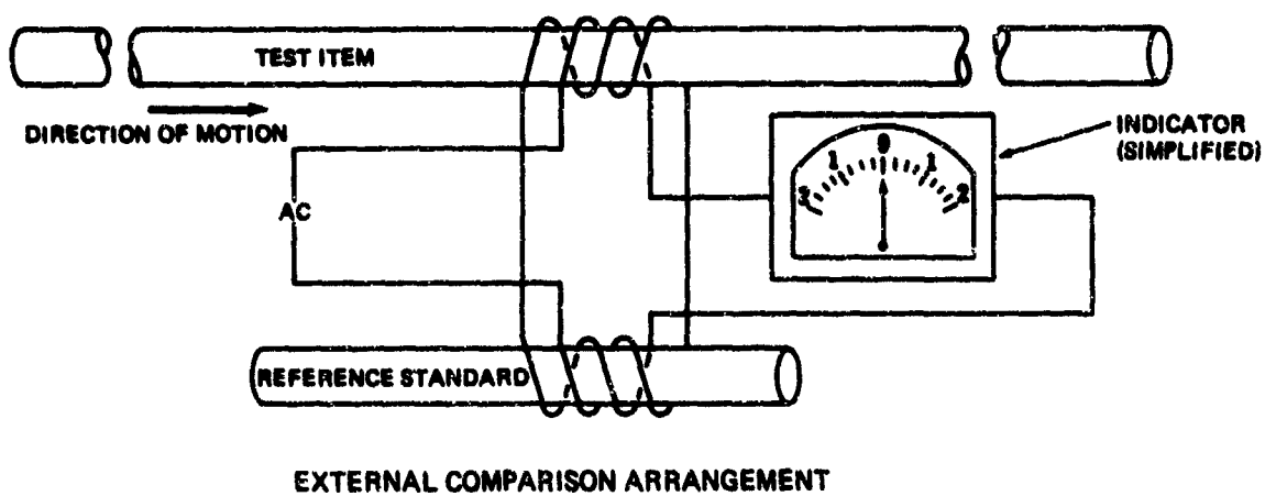
Figure 50. Eddy Current Test Setups
