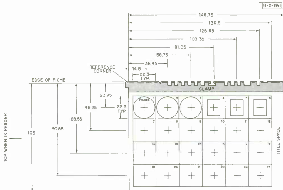
Fig. 12. LTS-3 microfiche card format — right reading emulsion side, looking toward light source (dimensions in millimeters).
