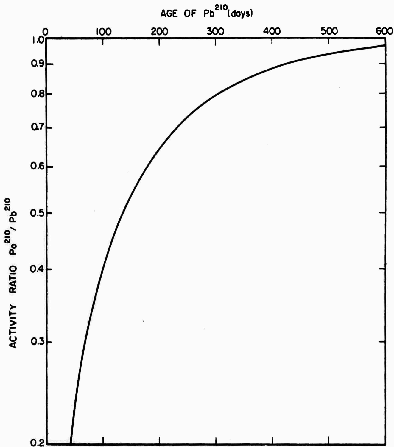
FIGURE 125. VARIATION OF THE ACTIVITY RATIO \text{Po}^{210} / \text{Pb}^{210} WITH THE AGE OF THE LEAD-210
