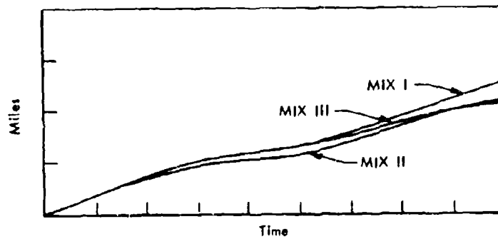
Fig. 9.9 - Case 2: Movement of the FEBA (west)
