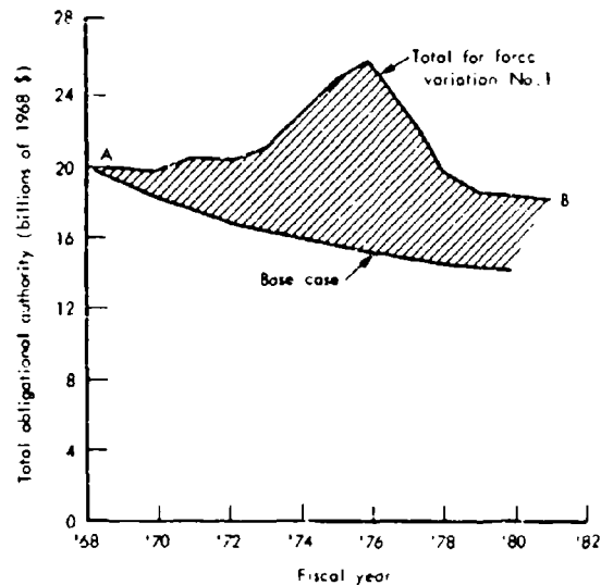
Fig. 4.17 - Net impact on TOA of force variation No. 1
