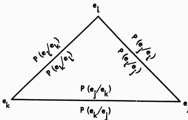
Fig. 1—Rule of the triangle
