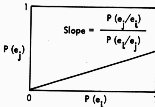
Fig. 2--Geometric representation of the rule of the product
