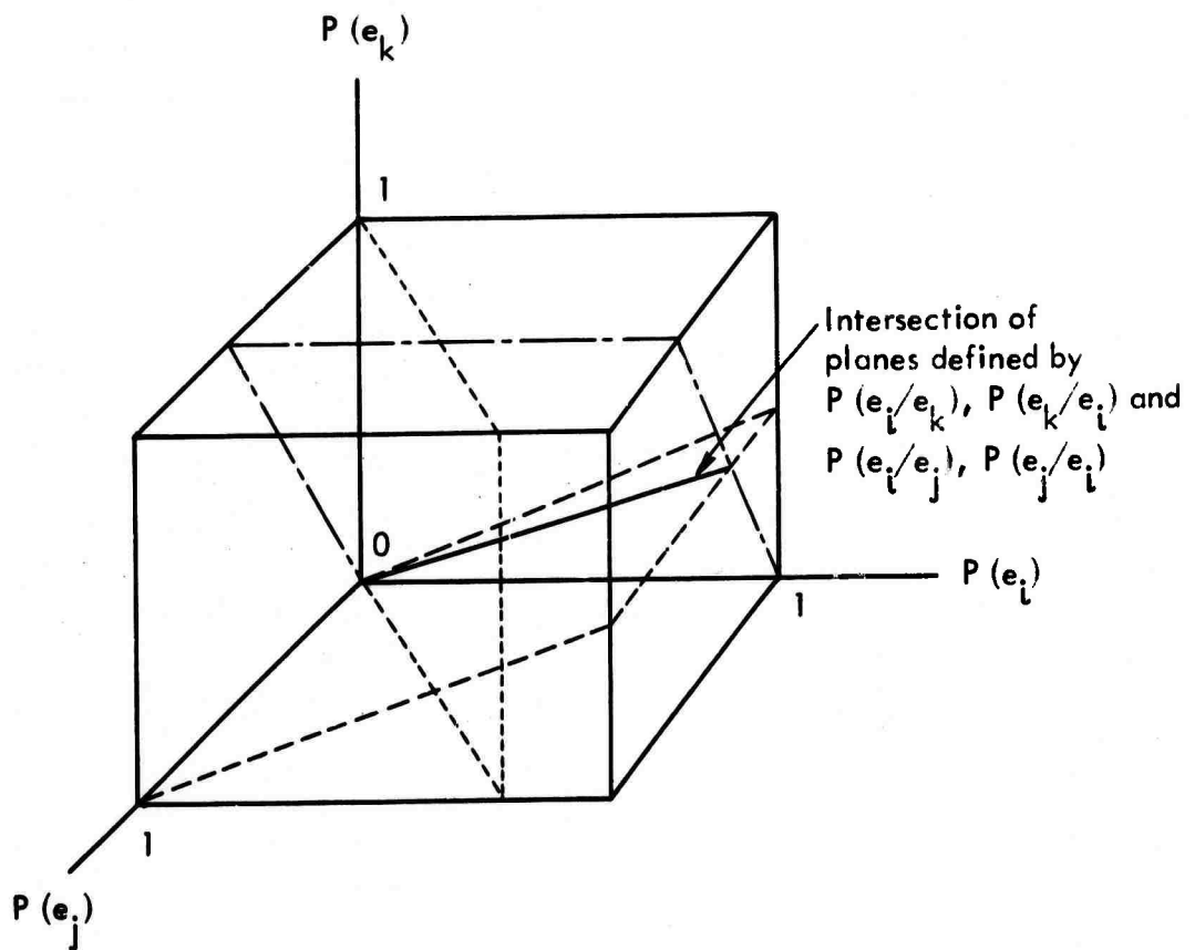
Fig. 3--Inconsistent relative probabilities for three events
