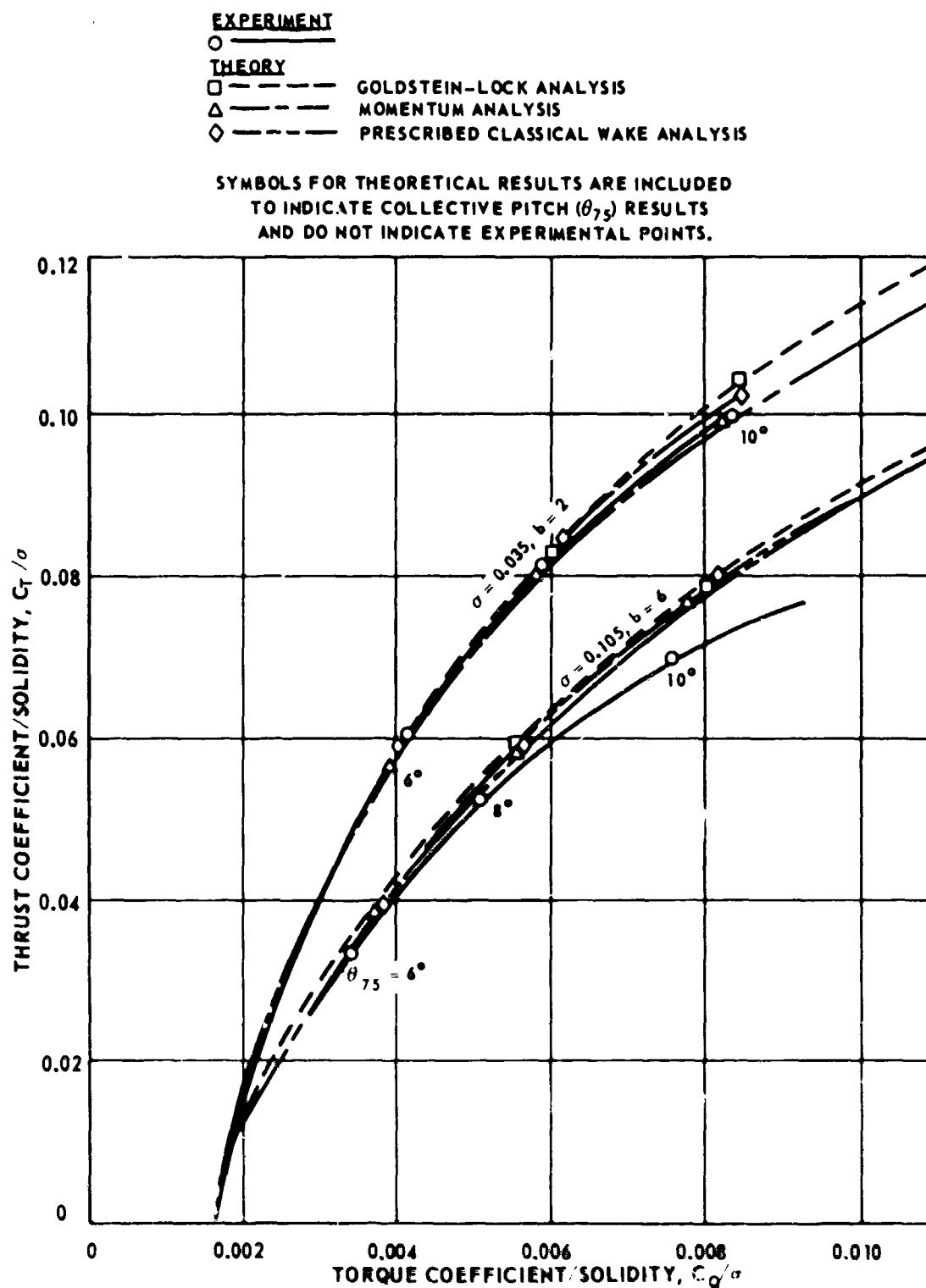
Figure 9. Comparison of Results of Uncontracted Wake Analyses With Experimental Performance Results for Two- and Six-Bladed Model Rotors -- \alpha_1 = 0^\circ , AR = 18.2 , 11R = 700 fps.
