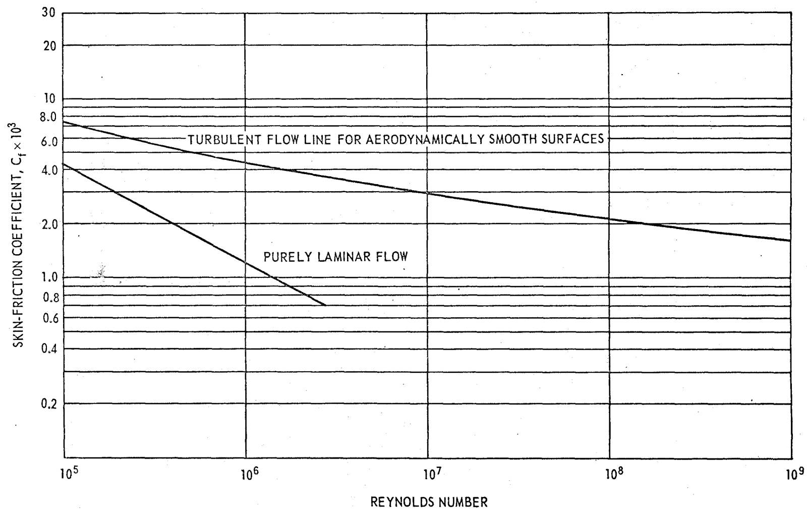
Figure 9 – Incompressible Skin Friction Coefficient (from Reference 9)
