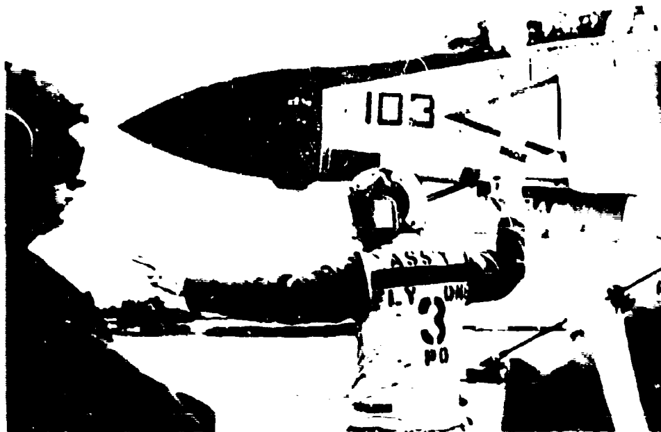
Figure 4. An F4 Phantom (A) being brought into position on the port bow catapult and (B) with bridle in place on the starboard bow catapult, being handed-off from the Fly One Director to the Catapult Officer.
