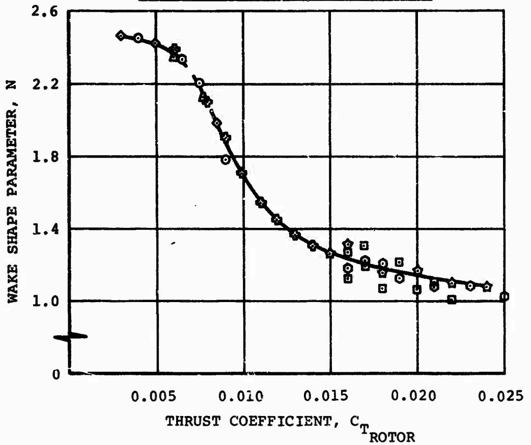
Figure 50. Rotor Wake Shape Parameter.
