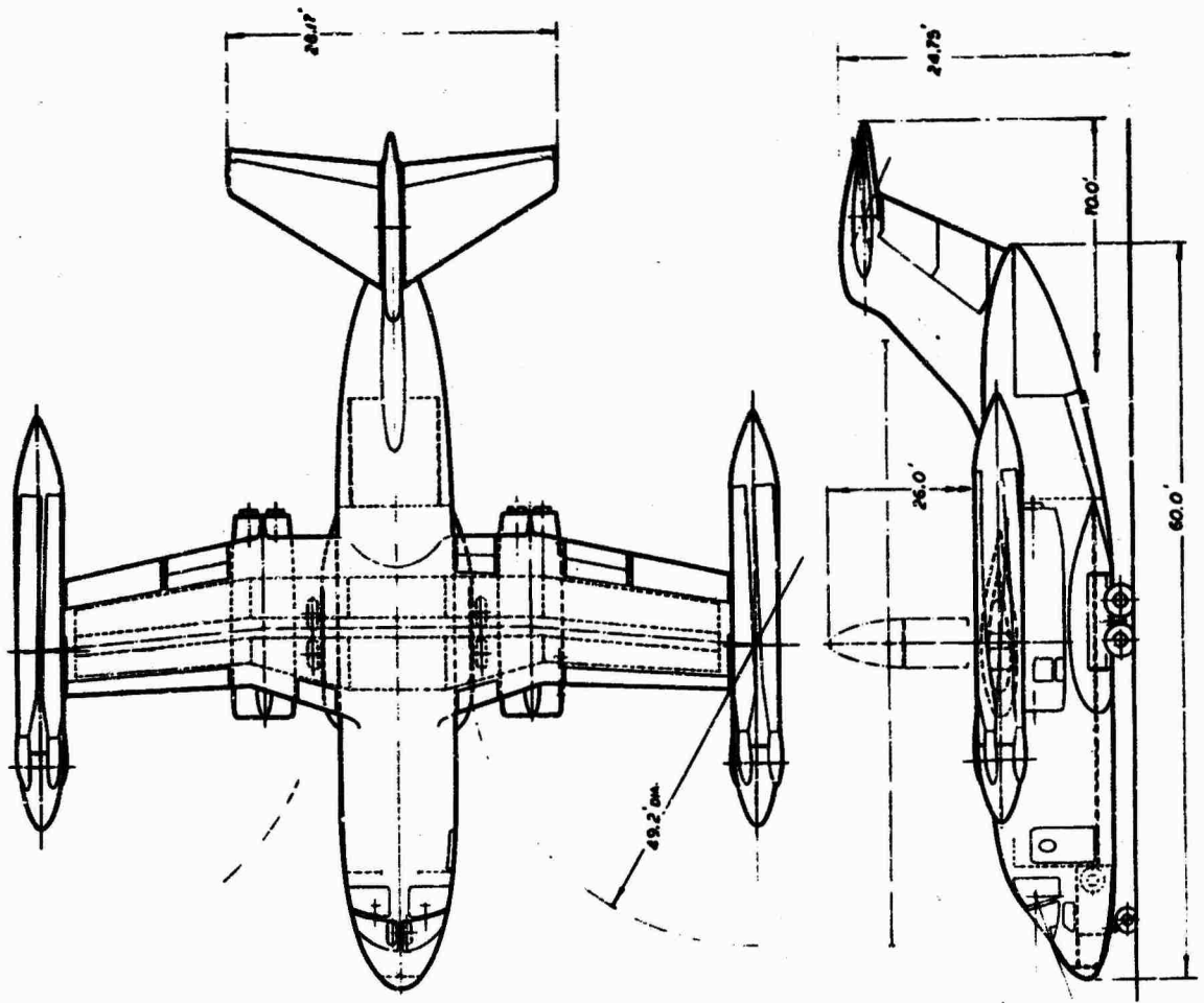
Figure 38. 3-View of Baseline Transport Aircraft.
