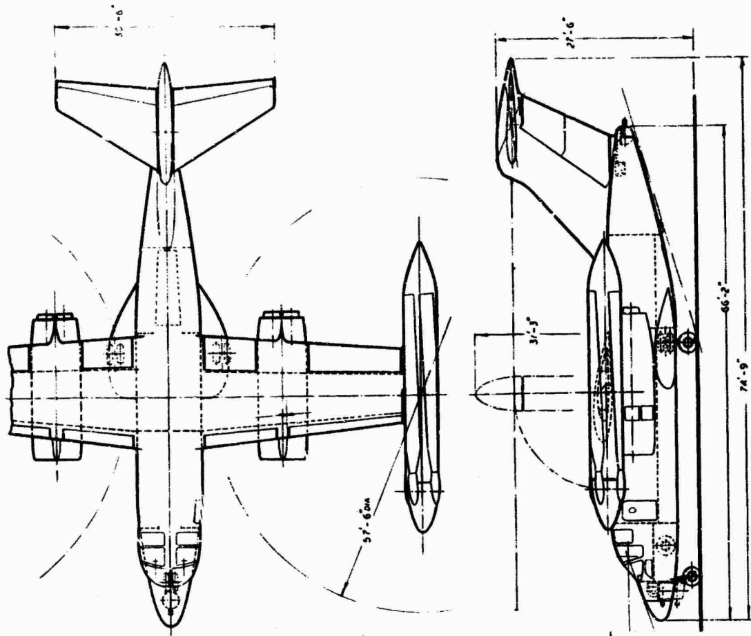
Figure 27. 3-View of Design Point III Multimission Aircraft, Rescue Version.
