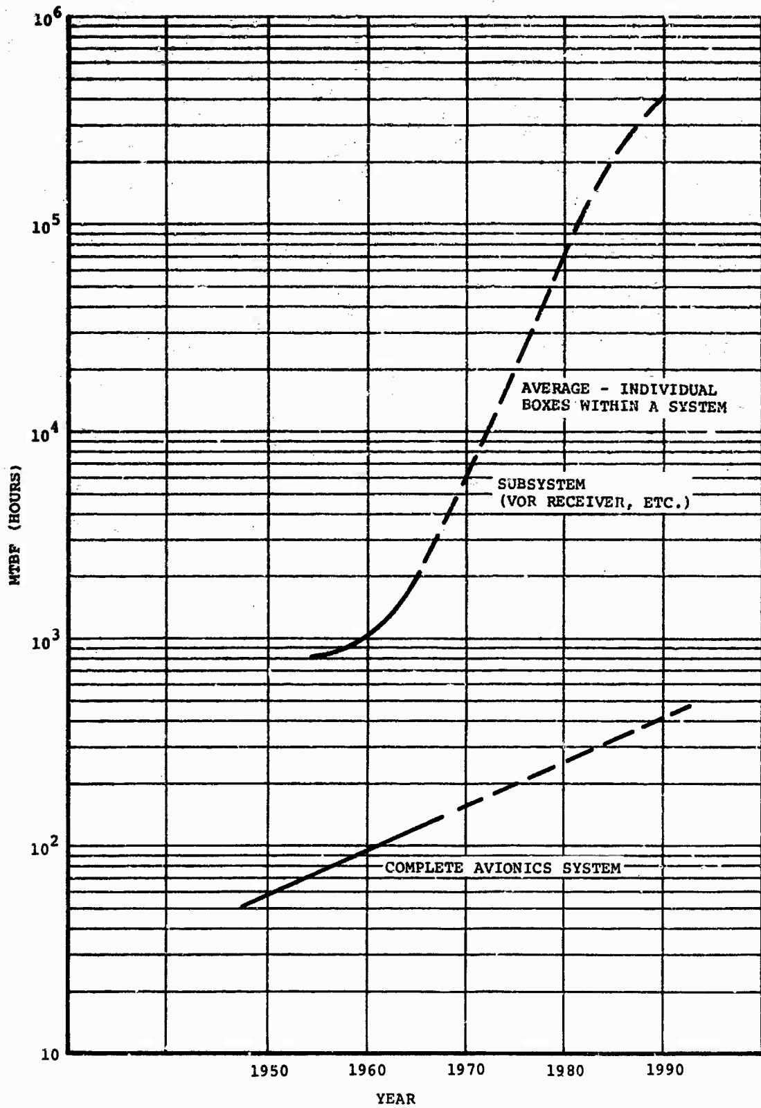
Figure 127. Avionics System Reliability Trends.
