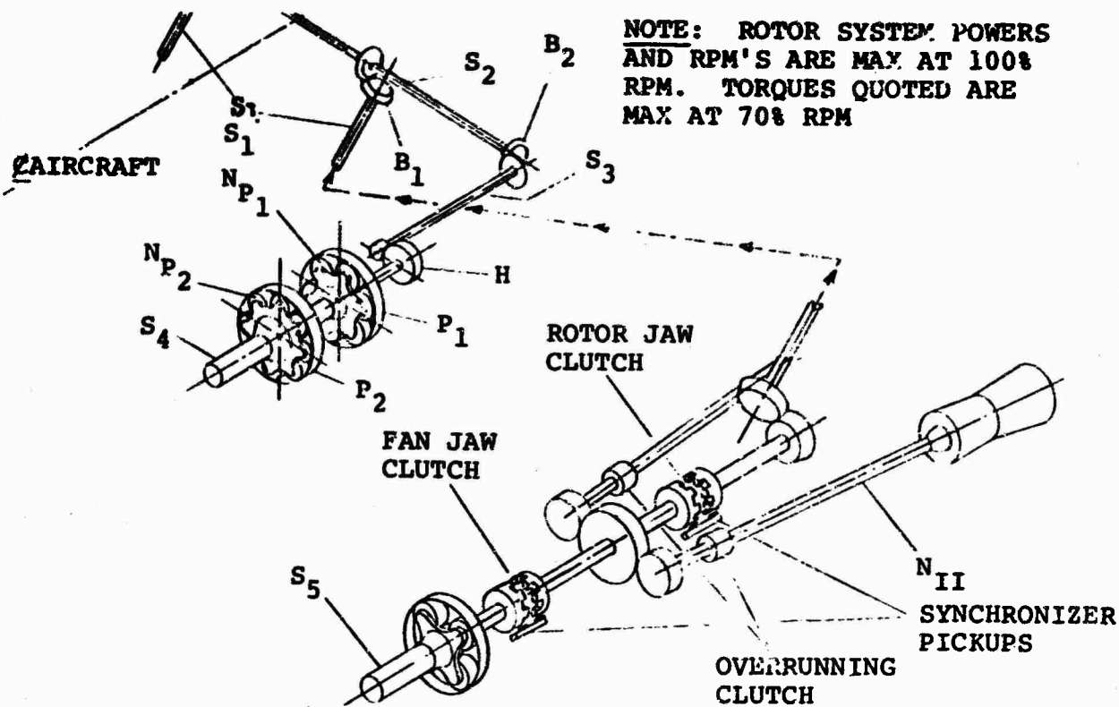
Figure 70. Design Point IV Drive Schematic.
