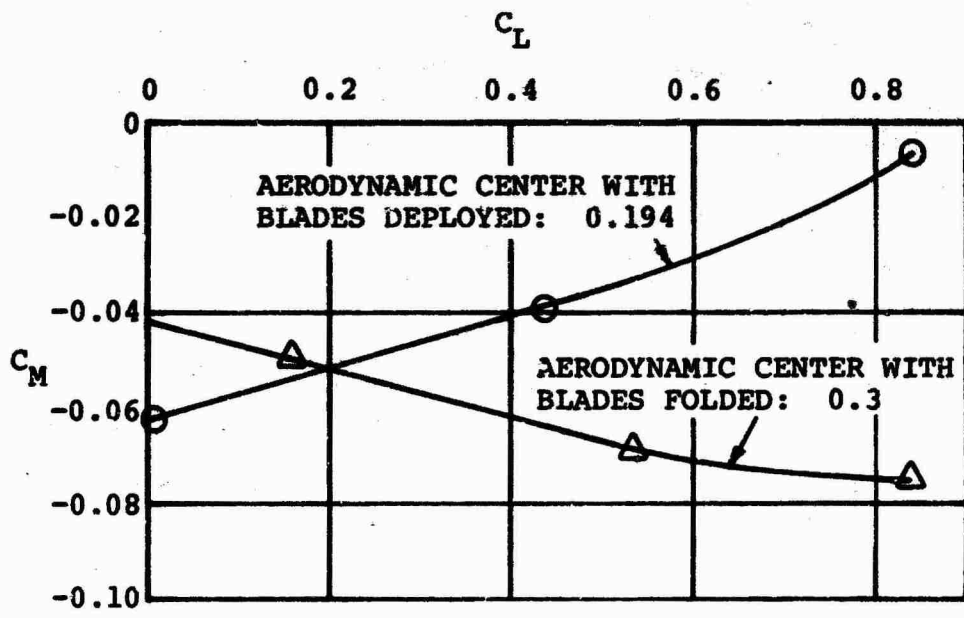
Figure 84. Effect of Blade Folding on Longitudinal Stability.
