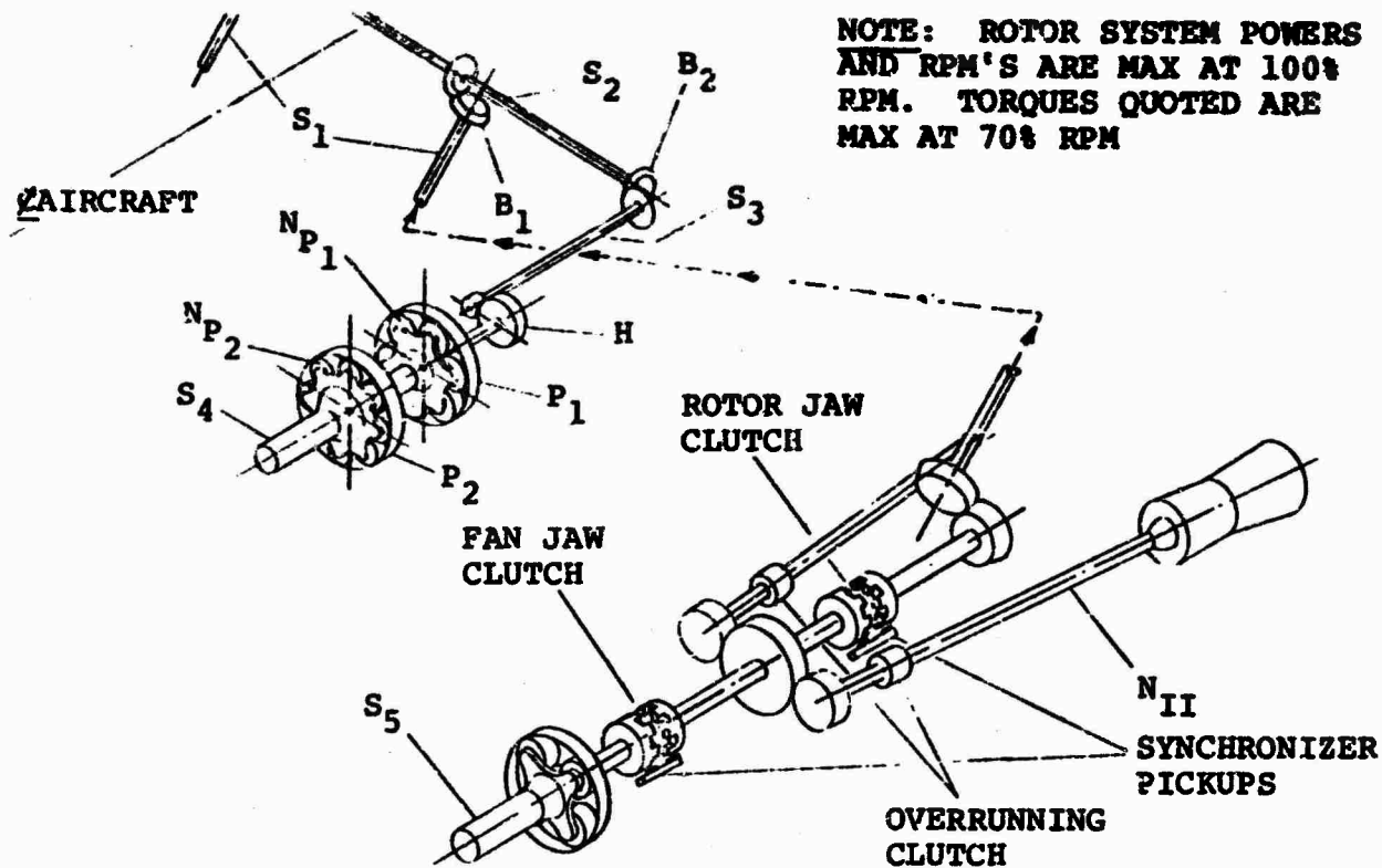
Figure 71. Design Point V Drive Schematic.
