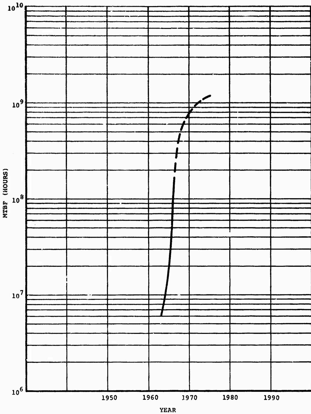
Figure 128. Improvement in High Reliability Microcircuits.
