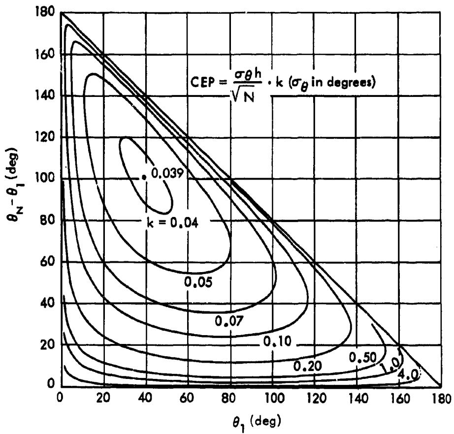
Fig.3a—CEP isocontours for multiple bearing measurements
