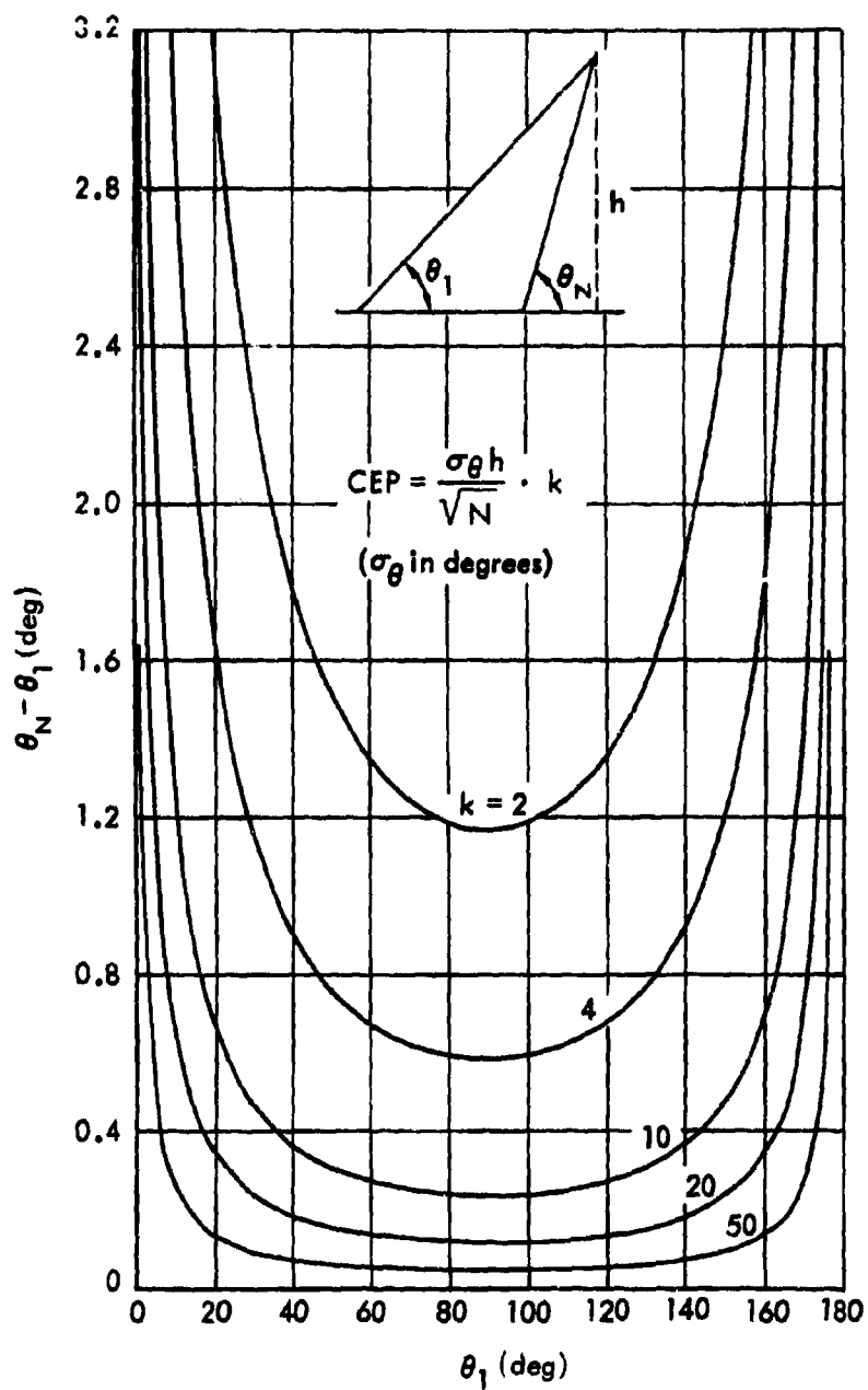
Fig.3b—CEP isocontours for multiple bearing measurements (small included angles)
