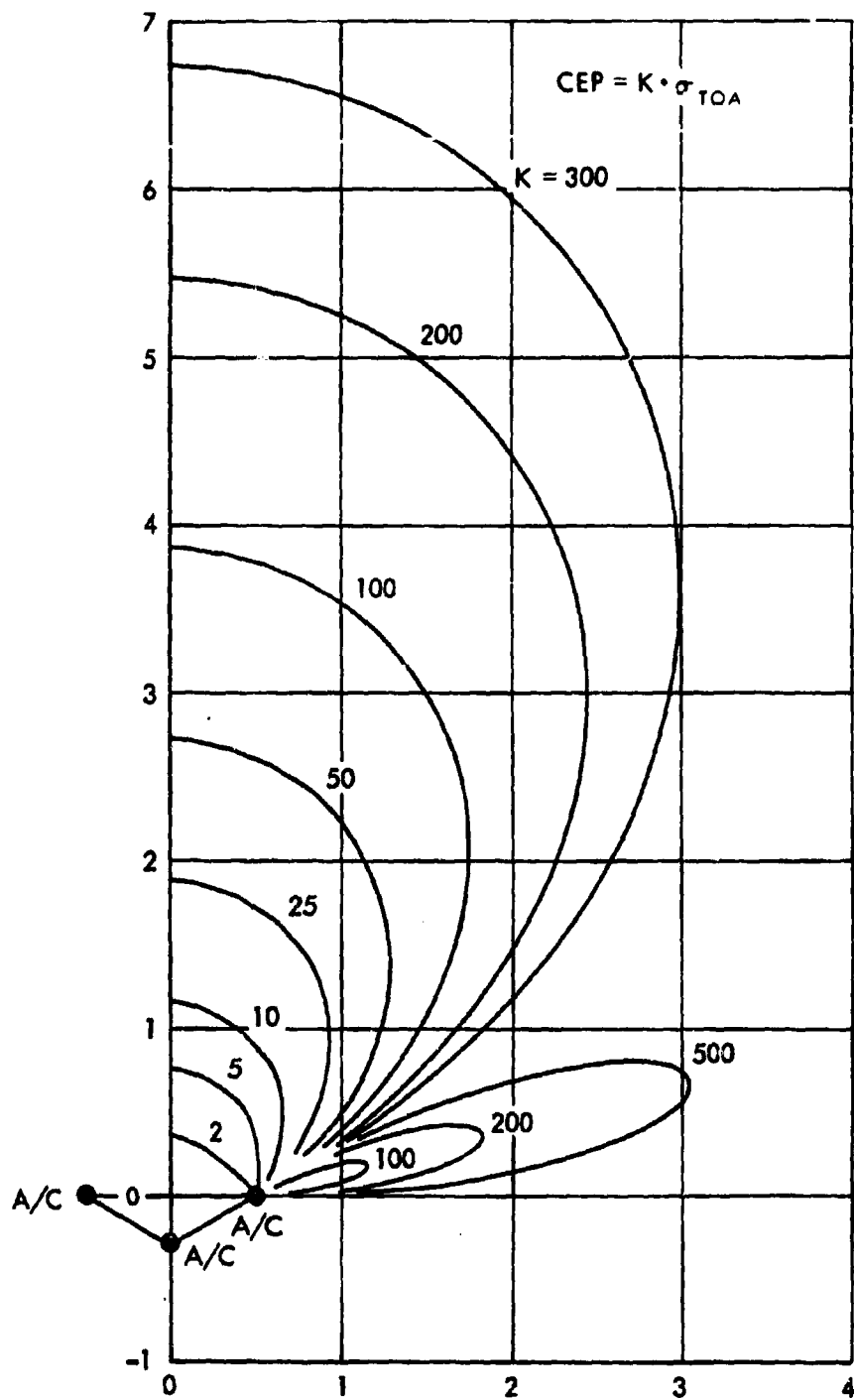
Fig.6—CEP Isocontours for 120-deg isosceles triangle (TOA)
