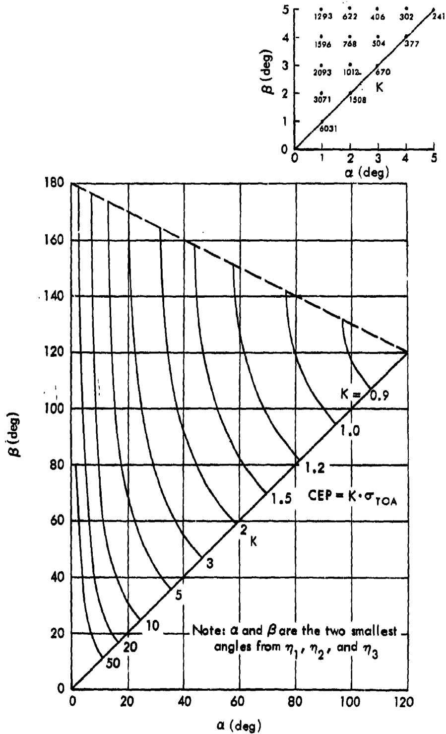
Fig. 4—CEP Isocontours for arbitrary TOA aircraft triangles
