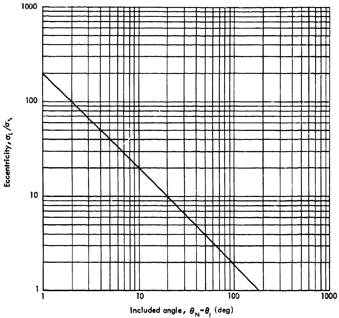
Fig.2—Eccentricity of location error distribution as a function of emitter included angle
