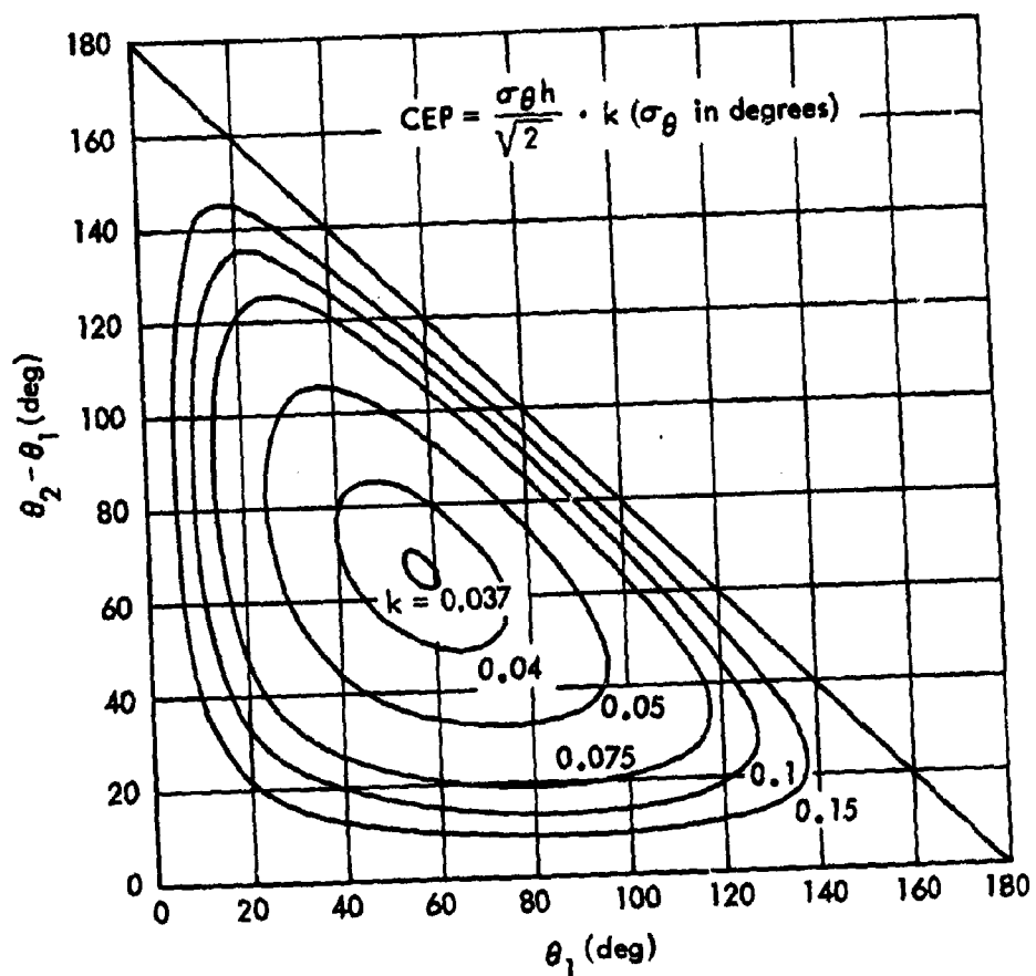
Fig.1—CEP isocontours for two bearing measurements
