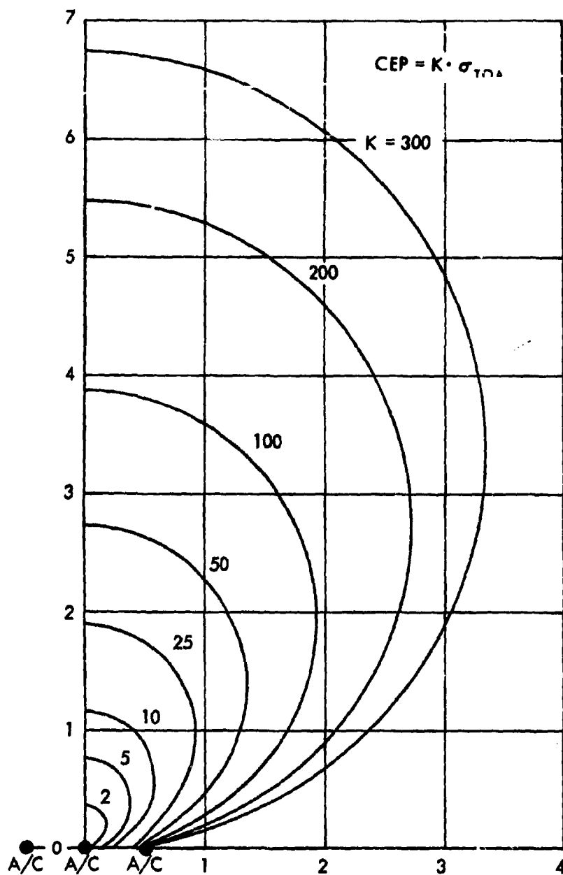
Fig.5—CEP isocontours for 180-deg isosceles (line) triangle (TOA)
