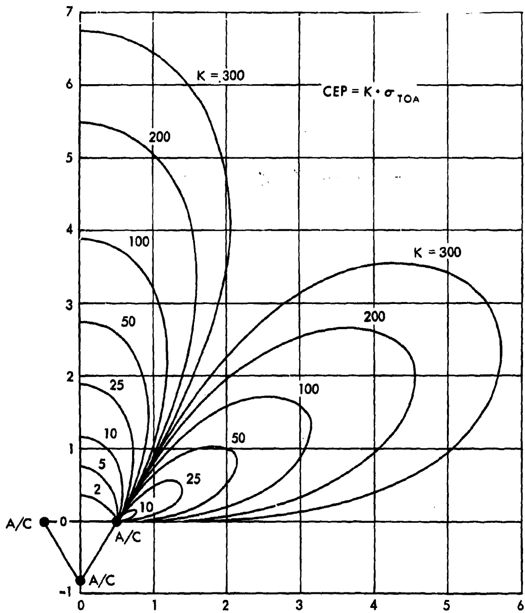
Fig.7—CEP isocontours for 60-deg isosceles (equilateral) triangle (TOA)
