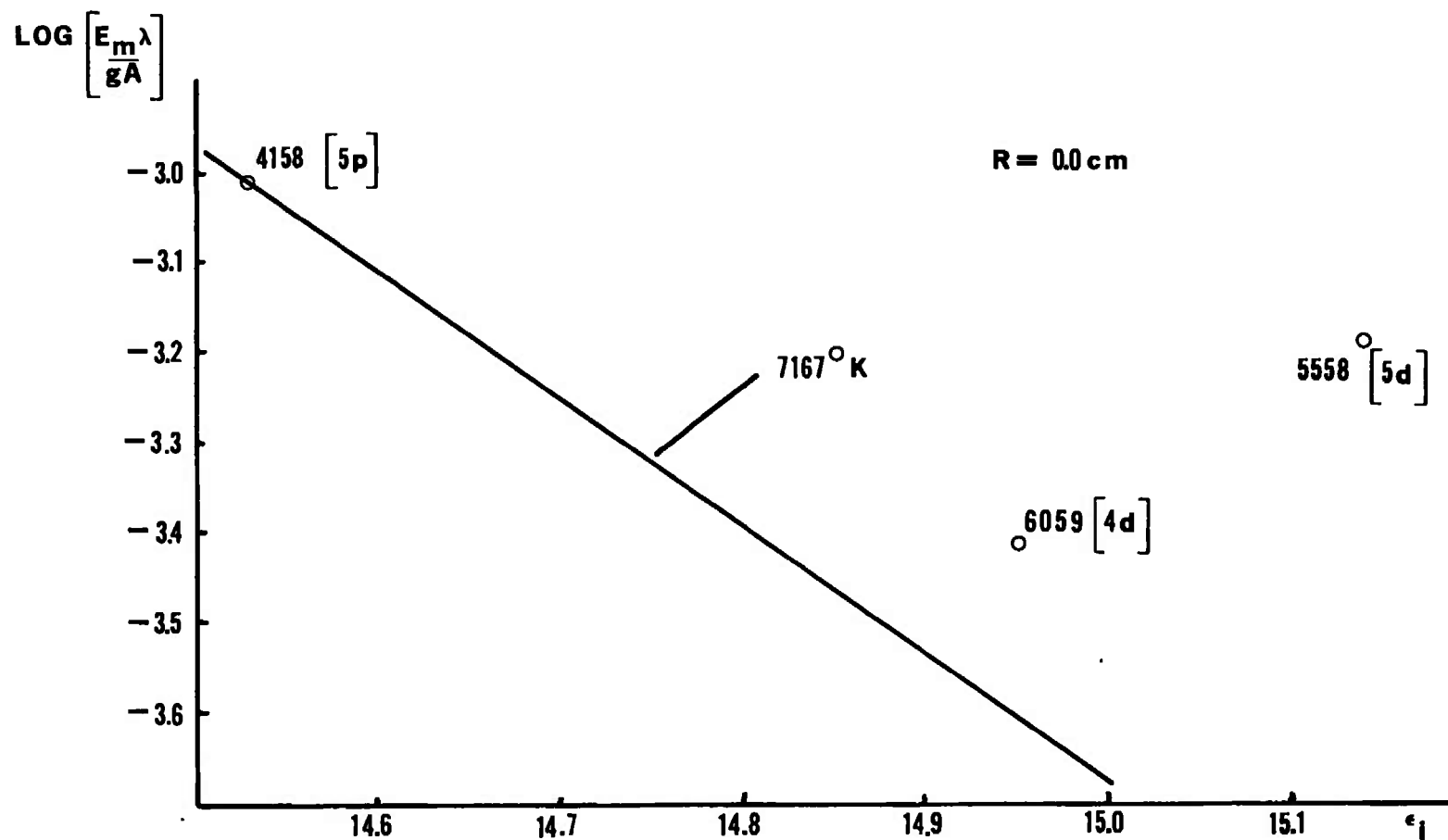
Fig. 13. Boltzmann plot at the discharge axis.
