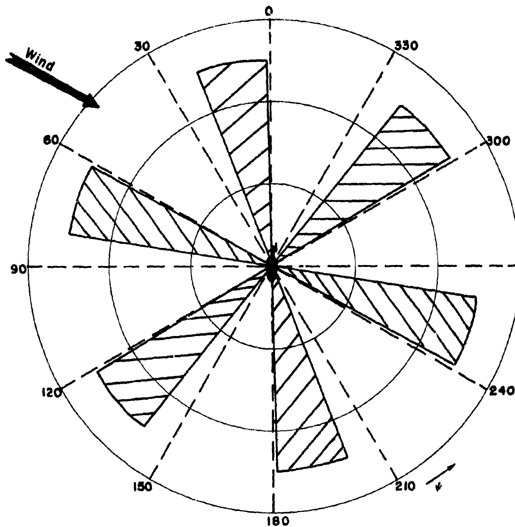
Figure 39. Range of Rotor Blade Locations at Instant of RIN Generation for OGE Hover.
