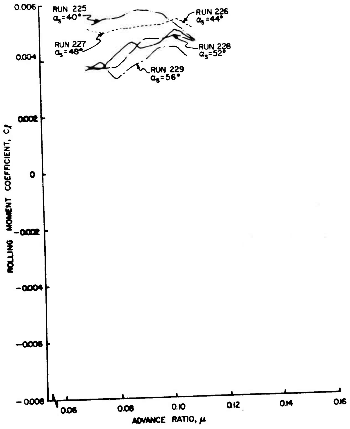
Figure 45b. Rotor Force and Moment Coefficients as Functions of Advance Ratio, \theta_{TSR} = 2^\circ , Large Wing on High.
