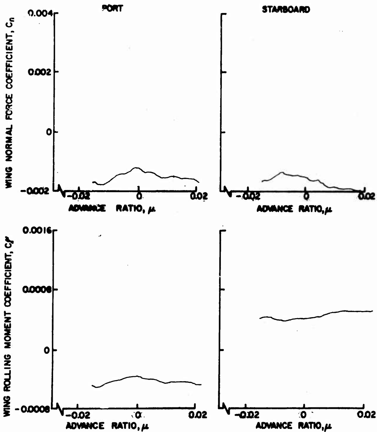
Figure 77. Wing Normal Force and Rolling Moment Coefficients as Functions of Advance Ratio, \theta = 8^\circ , Large Wing on High, \frac{h}{D} = 0.75 .
