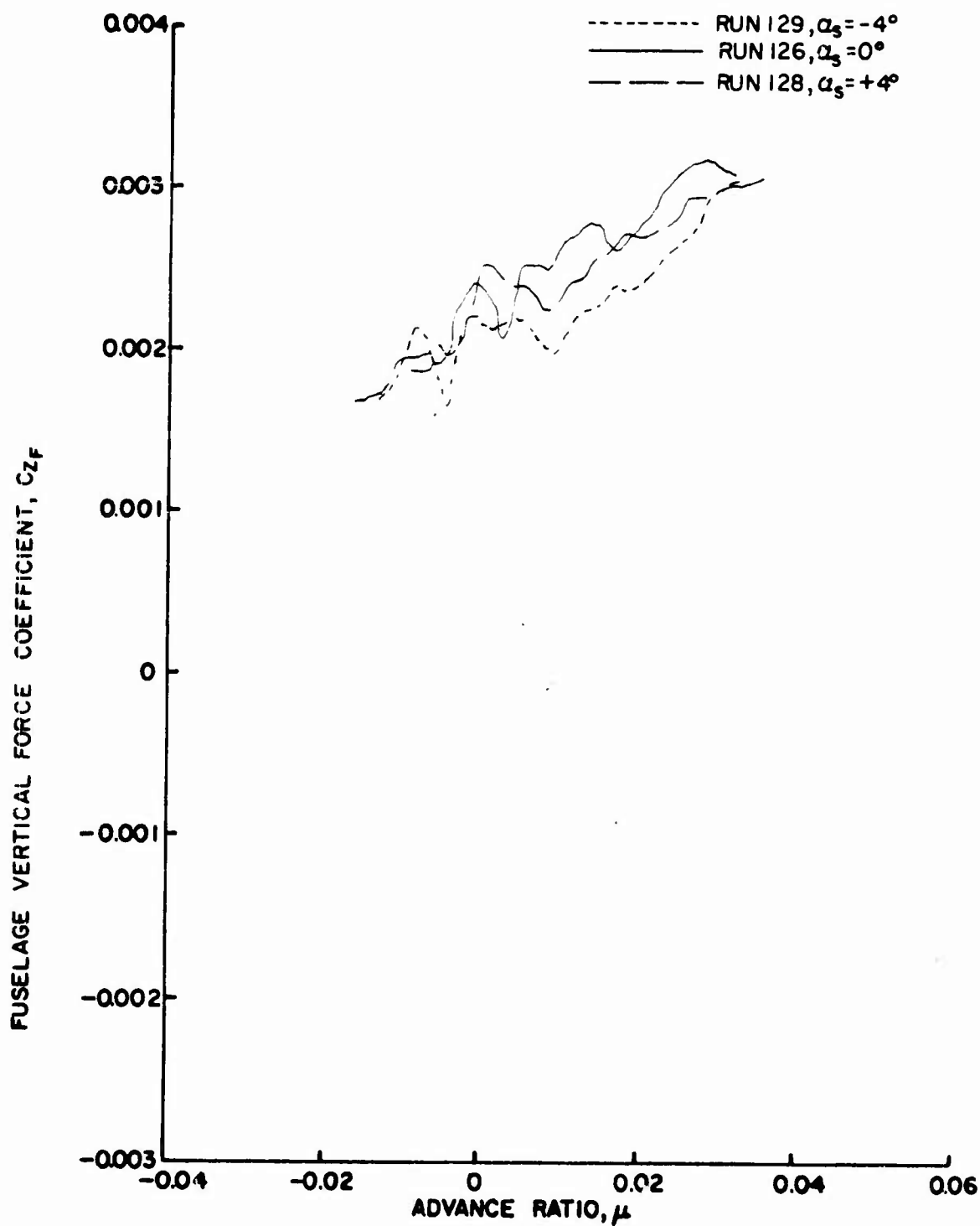
Figure 2a. Fuselage Vertical Force and Pitching Moment Coefficients as Functions of Advance Ratio, \theta_{\text{wing}} = 10^\circ , Wing Off, Fuselage On, \frac{z}{R} = 0 .
