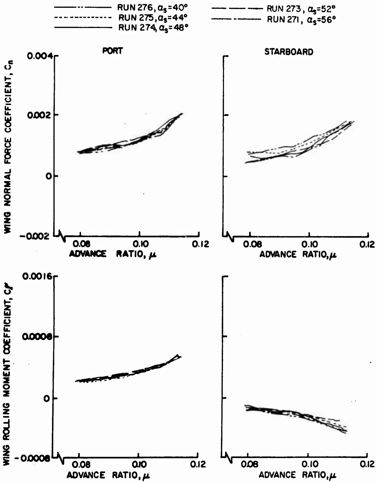
Figure 59. Wing Normal Force and Rolling Moment Coefficients as Functions of Advance Ratio, \theta = 6^\circ , Large Wing on High.
