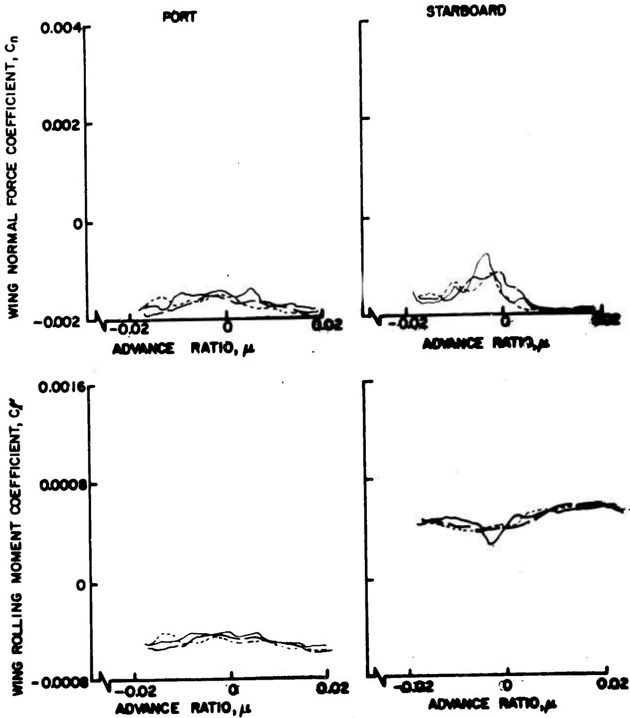
Figure 84. Wing Normal Force and Rolling Moment Coefficients as Functions of Advance Ratio, \theta = 10^\circ , Large Wing on Low, \frac{h}{D} = 0.75 .
