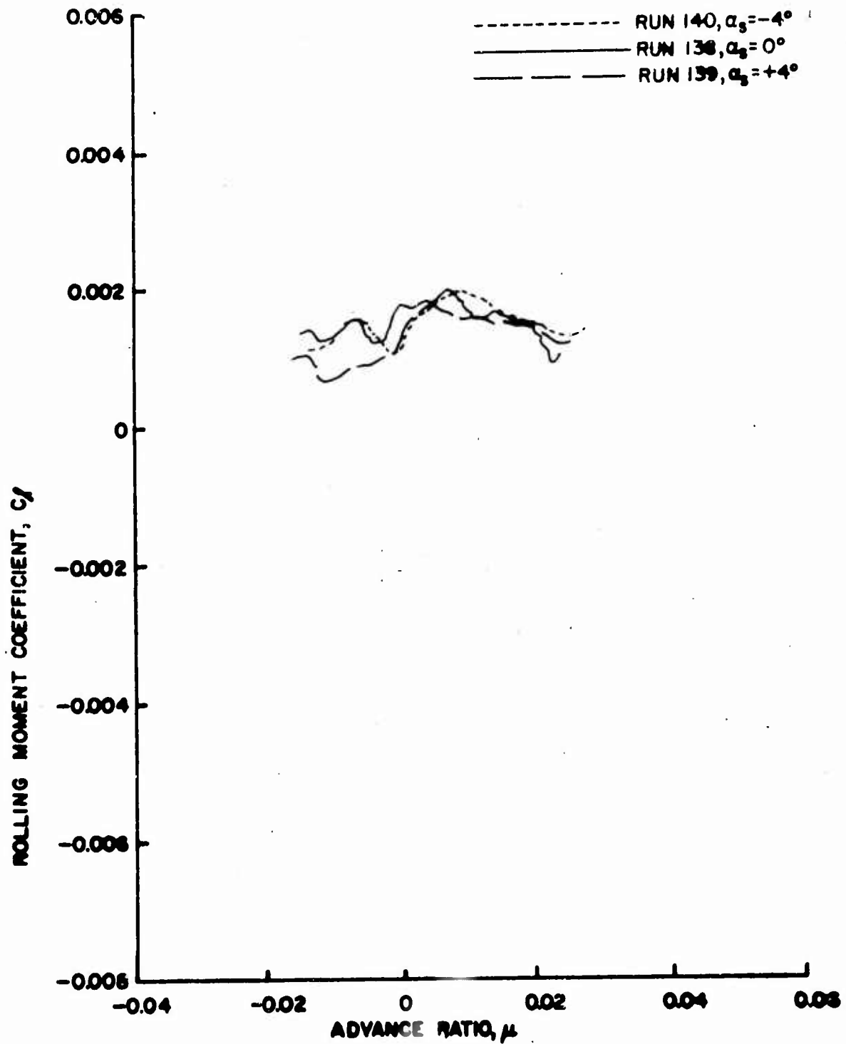
Figure 78. Rotor Force and Moment Coefficients as Functions of Advance Ratio, \theta_{.75R} = 10^\circ , Large Wing on High, \frac{h}{D} = 0.75 .
