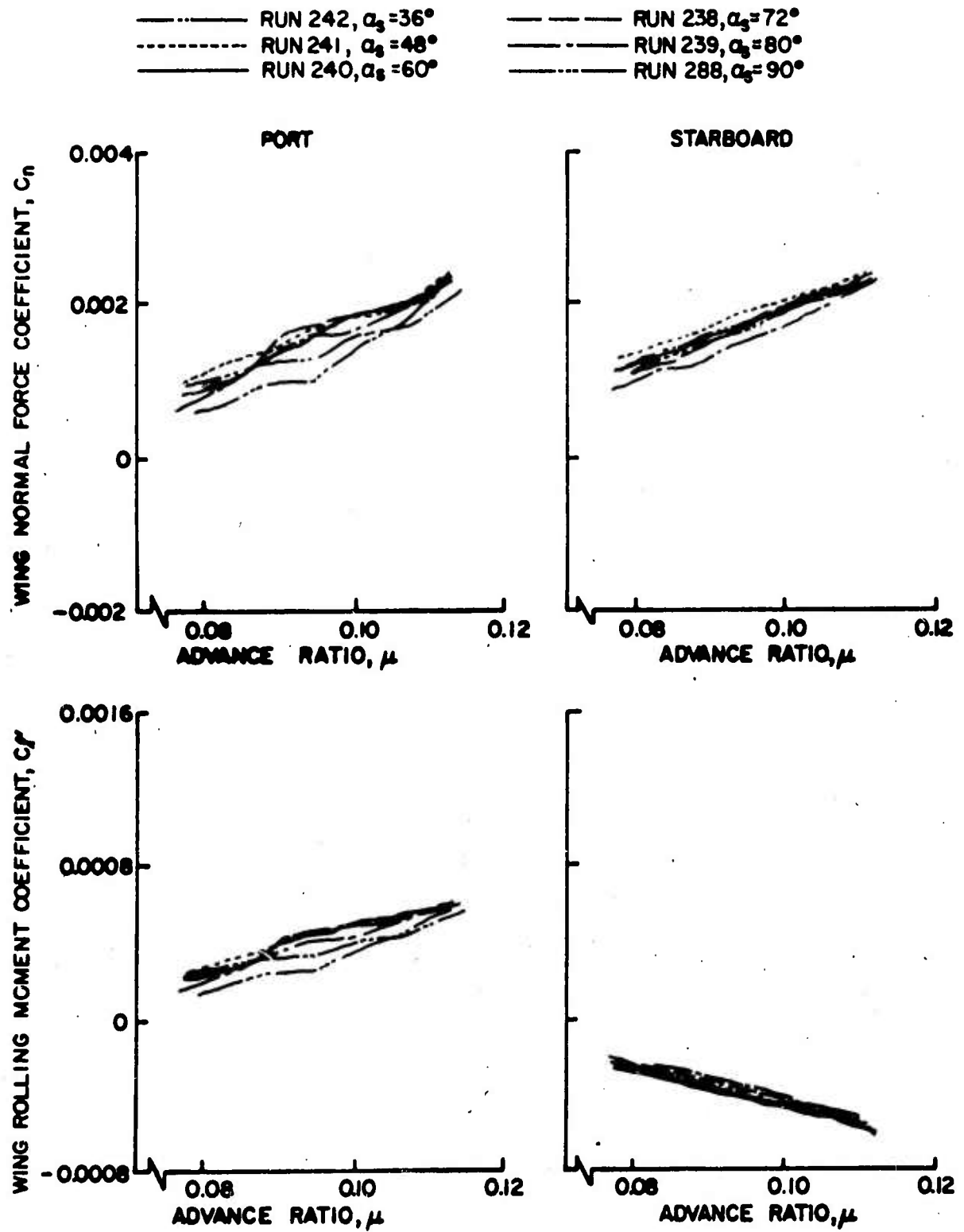
Figure 44. Wing Normal Force and Rolling Moment Coefficients as Functions of Advance Ratio, \theta_{.75R} = 0 , Large Wing on High.
