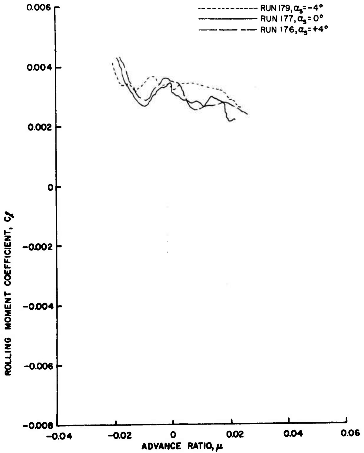
Figure 99c. Rotor Force and Moment Coefficients as Functions of Advance Ratio, \theta = 8^\circ , Large Wing on High,
