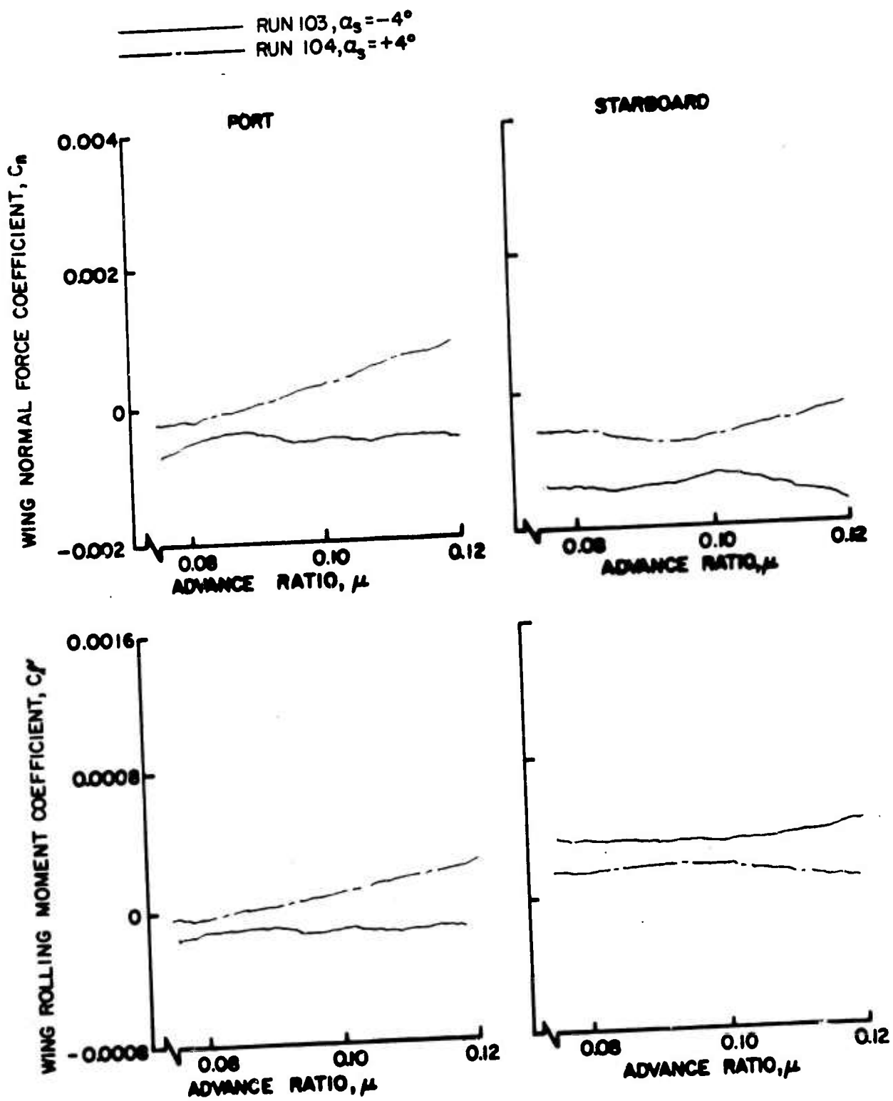
Figure 41. Wing Normal Force and Rolling Moment Coefficients as Functions of Advance Ratio, \theta = 12^\circ , Large Wing on Low.
