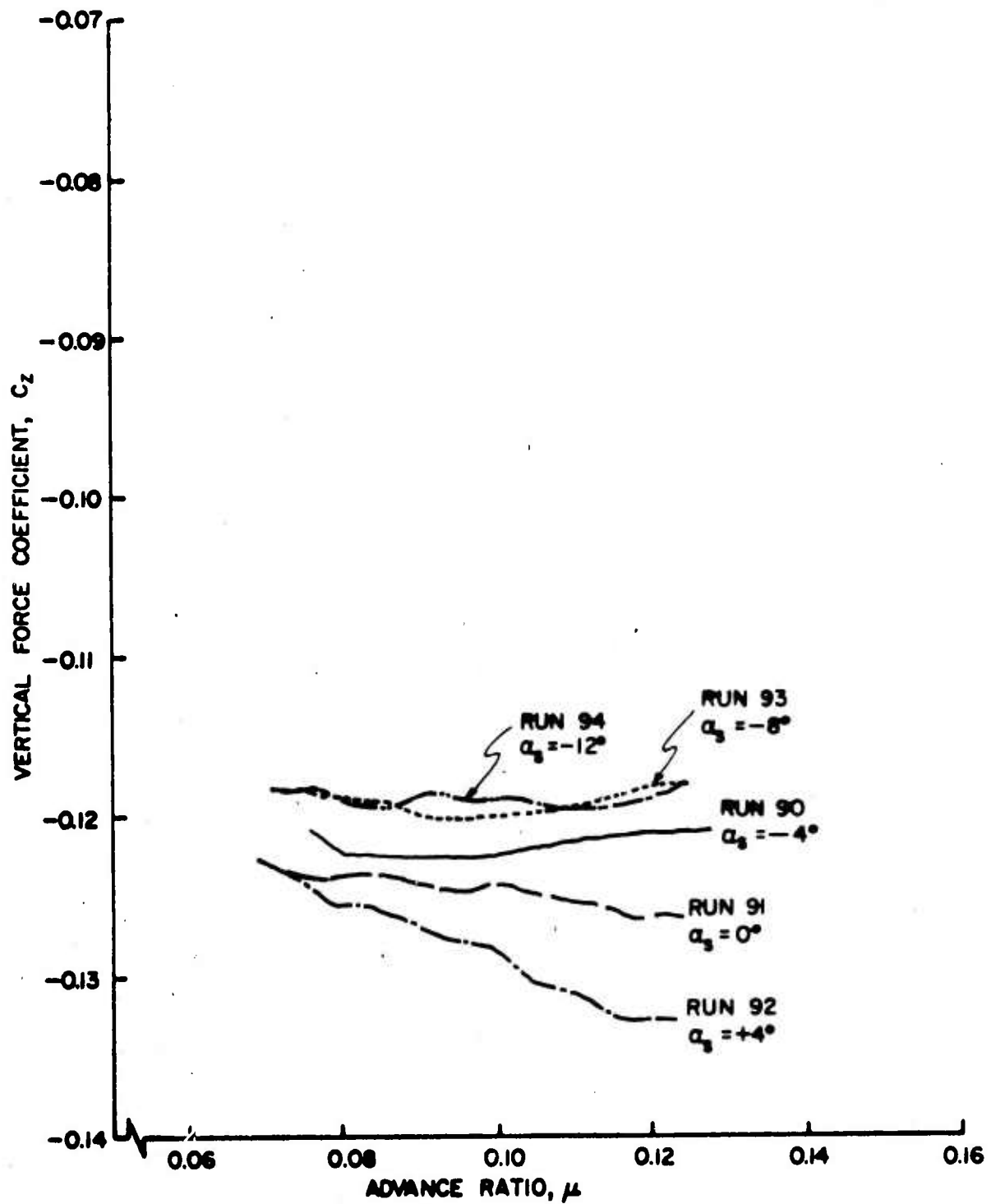
Figure 35b. Rotor Force and Moment Coefficients as Functions of Advance Ratio, \theta_{.75R} = 12^\circ , Wing Off.
