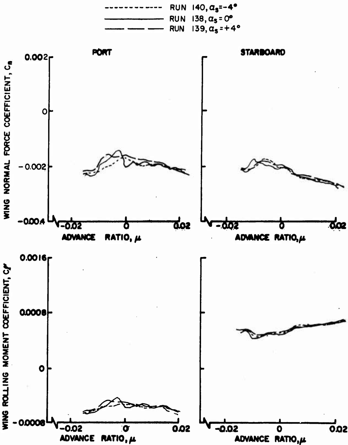
Figure 80. Wing Normal Force and Rolling Moment Coefficients as Functions of Advance Ratio, \theta = 10^\circ , Large Wing on High, \frac{h}{D} = 0.75 .
