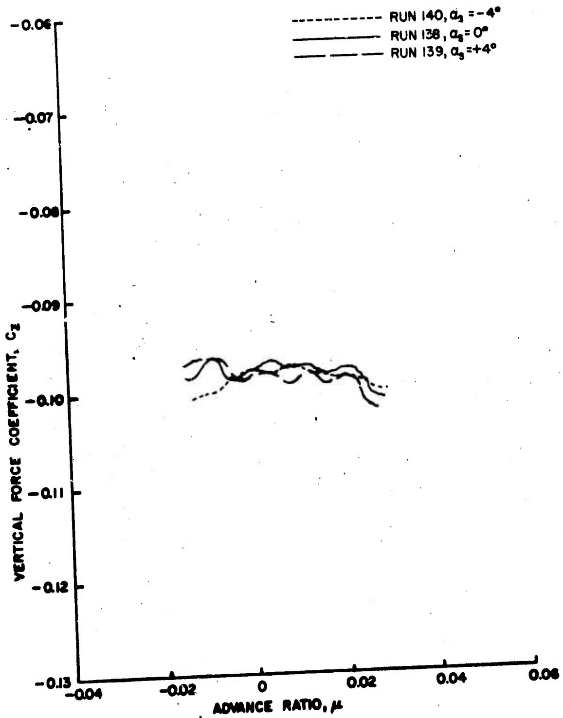
Figure 7(b). Rotor Force and Moment Coefficients as Functions of Advance Ratio, \theta = 10^\circ , Large Wing on High, .75R
