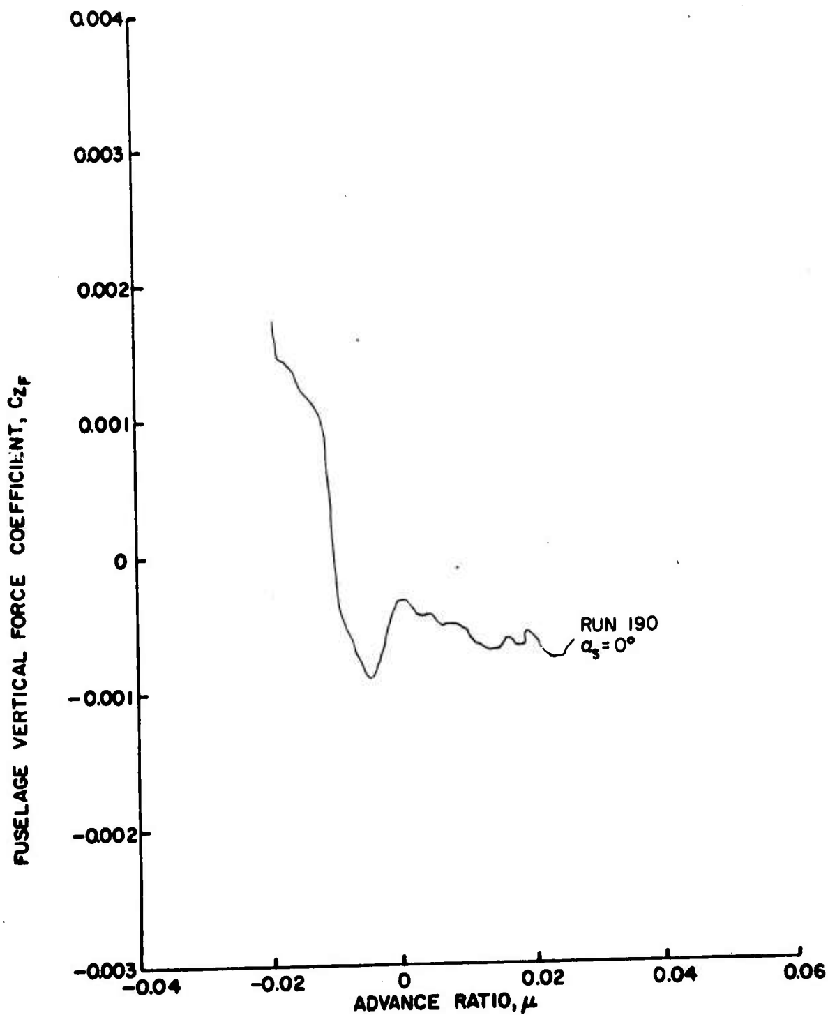
Figure 95a. Fuselage Vertical Force and Pitching Moment Coefficients as Functions of Advance Ratio, \theta_{.75R} = 12^\circ , Wing Off, Fuselage Q_m, \frac{h}{p} = 0.30 .
