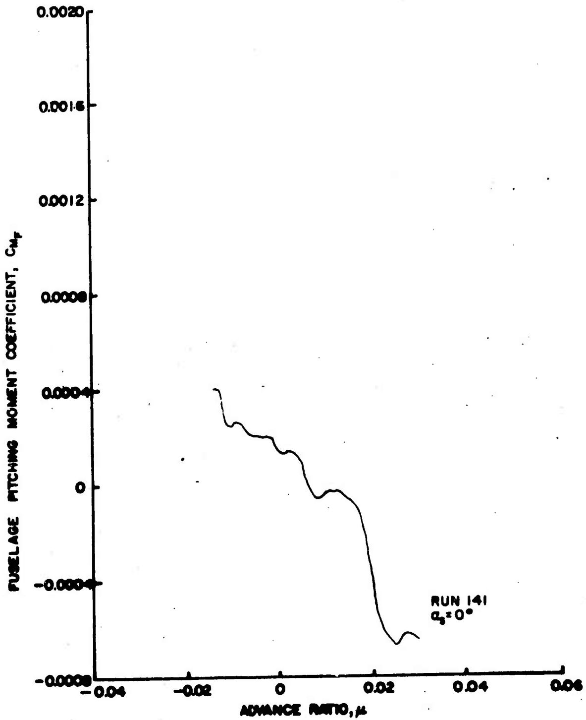
Figure 76. Fuselage Vertical Force and Pitching Moment Coefficients as Functions of Advance Ratio, \alpha_{.75R} = 8^\circ , Large Wing on High, \frac{h}{D} = 0.75 .
