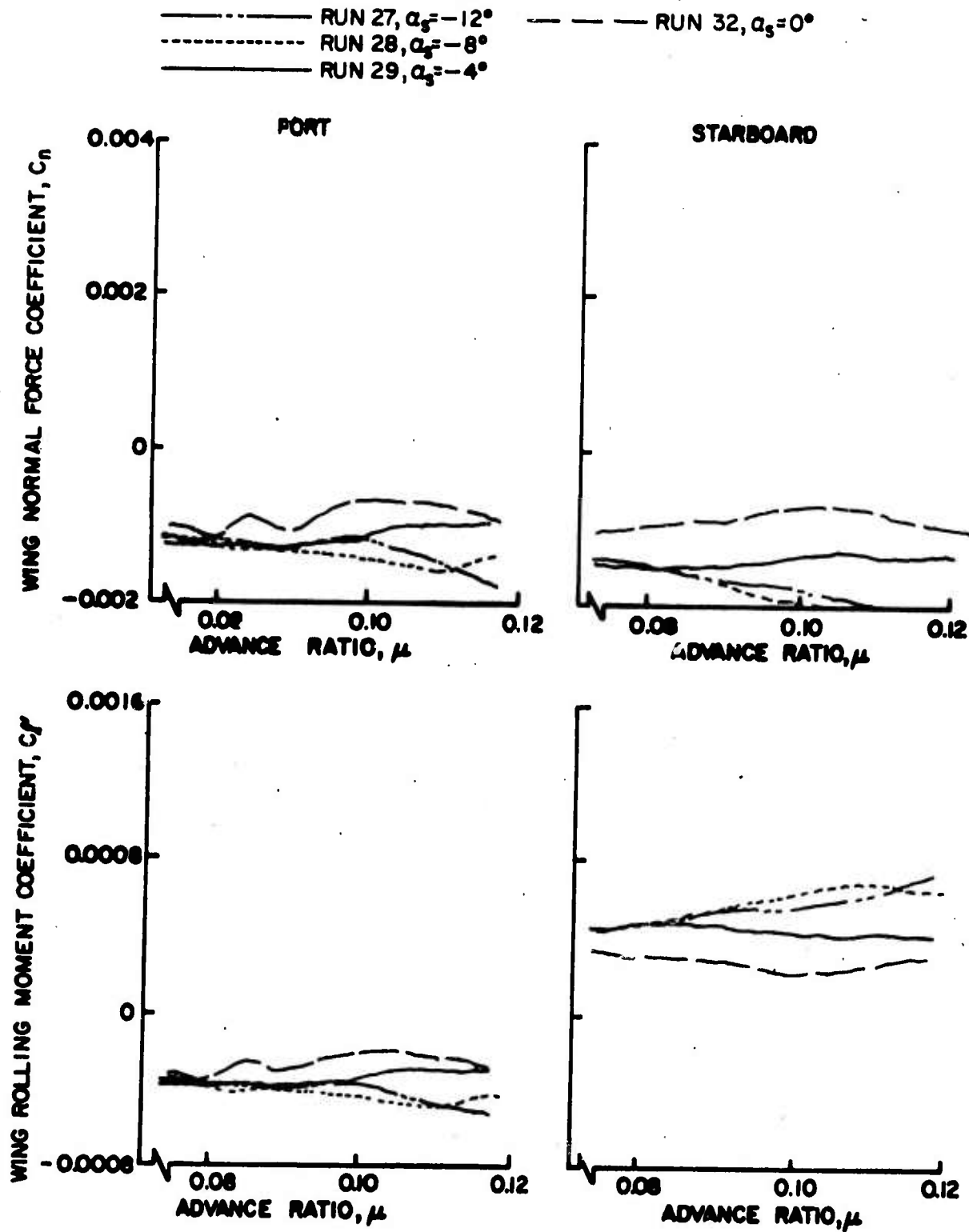
Figure 32. Wing Normal Force and Rolling Moment Coefficients as Functions of Advance Ratio, \theta = 10^\circ , Small Wing on High.
