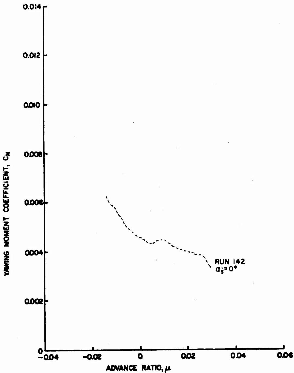
Figure 108e. Rotor Force and Moment Coefficients as Functions of Sideslip Ratio, \theta = 8^\circ , Large Wing on High,
