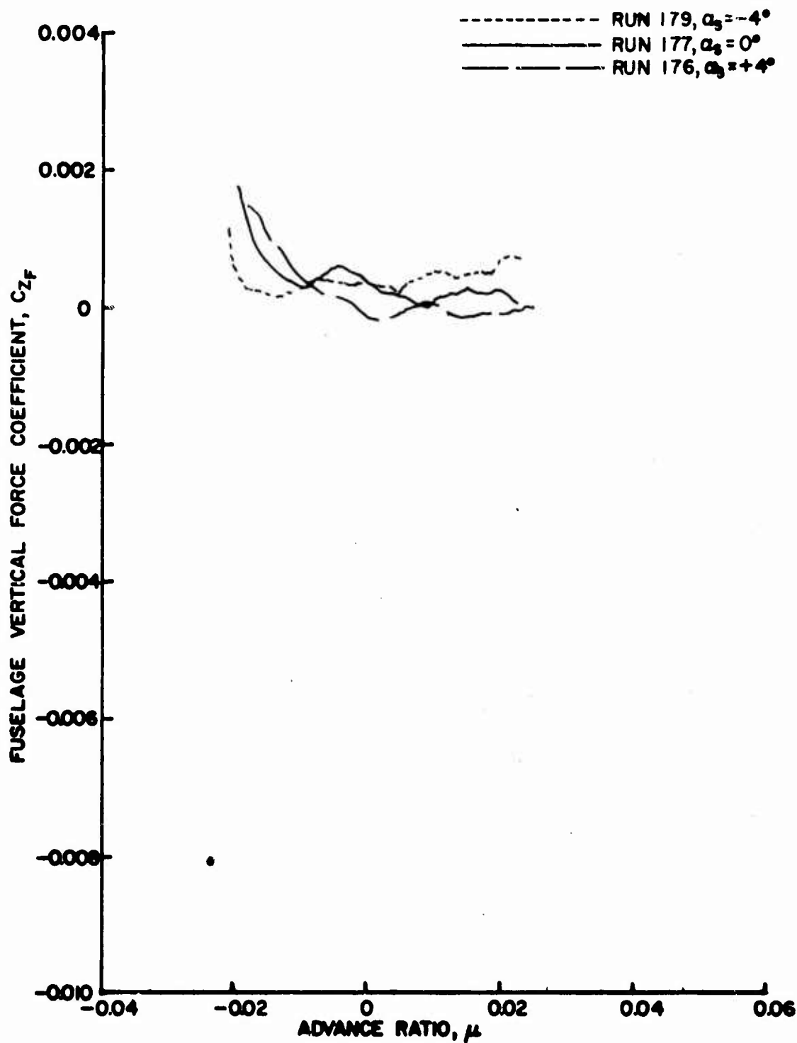
Figure 100a. Fuselage Vertical Force and Pitching Moment Coefficients as Functions of Advance Ratio, \theta = 10^\circ , Large Wing on High, \frac{h}{D} = 0.30 .
