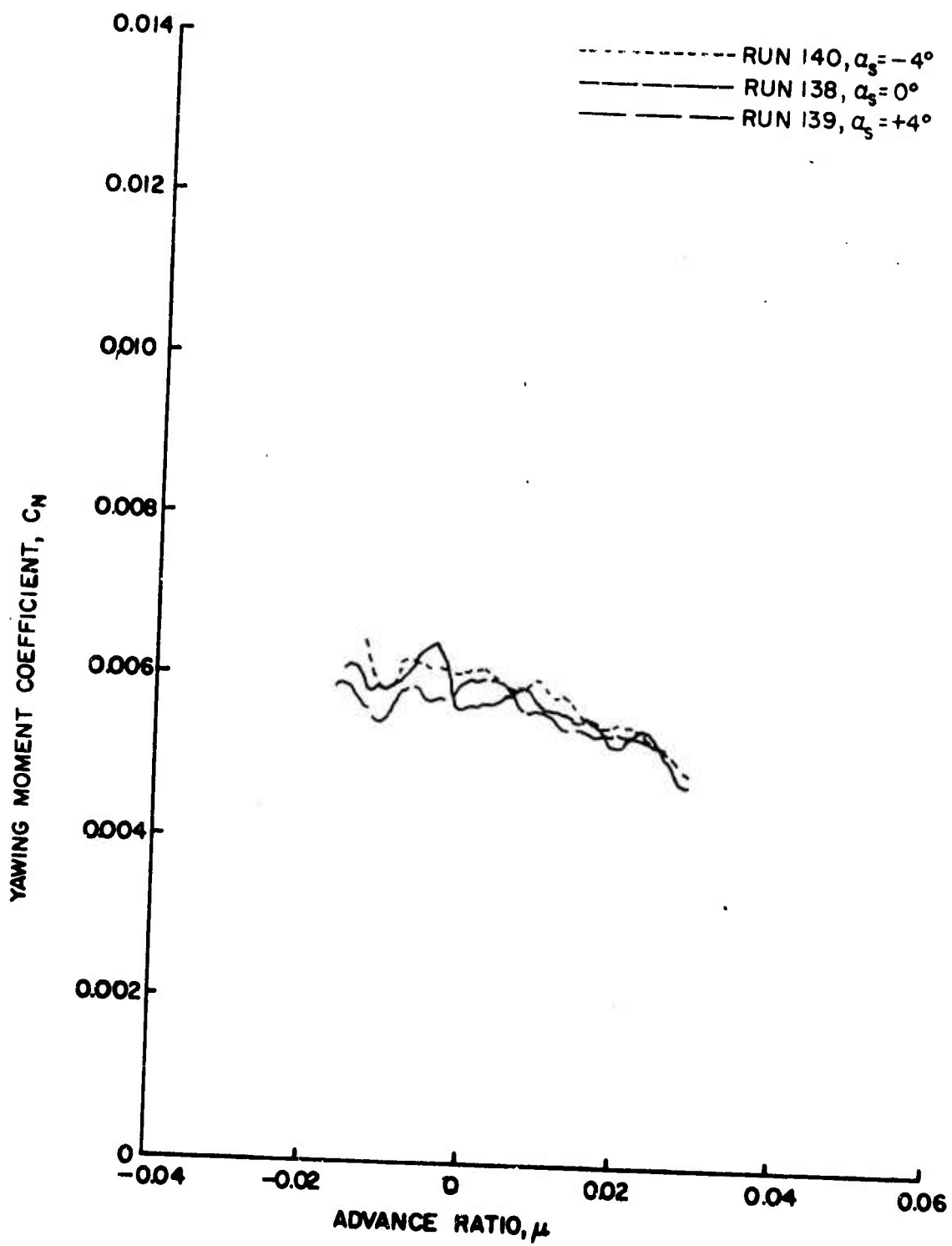
Figure 78e. Rotor Force and Moment Coefficients as Functions of Advance Ratio, \theta = 10^\circ , Large Wing on High, \frac{h}{D} = 0.75 .
