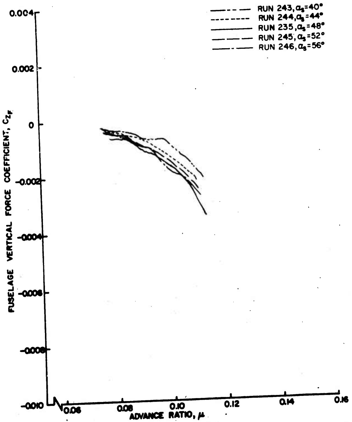
Figure 49a. Fuselage Vertical Force and Pitching Moment Coefficients as Functions of Advance Ratio, \theta = 4^\circ , Large Wing on High.
