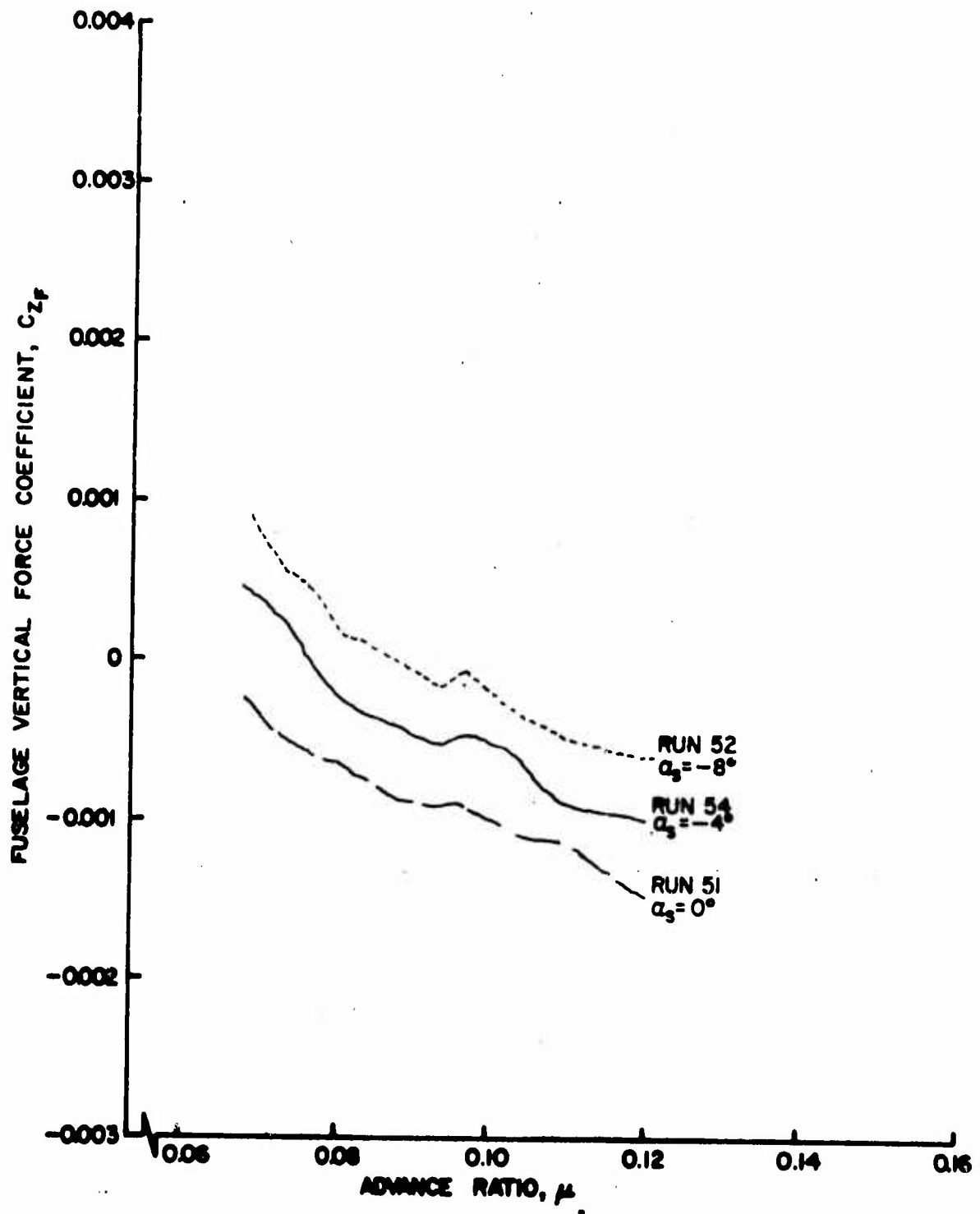
Figure 33a. Fuselage Vertical Force and Pitching Moment Coefficients as Functions of Advance Ratio, \theta = 10^\circ , Small Wing on Low.
