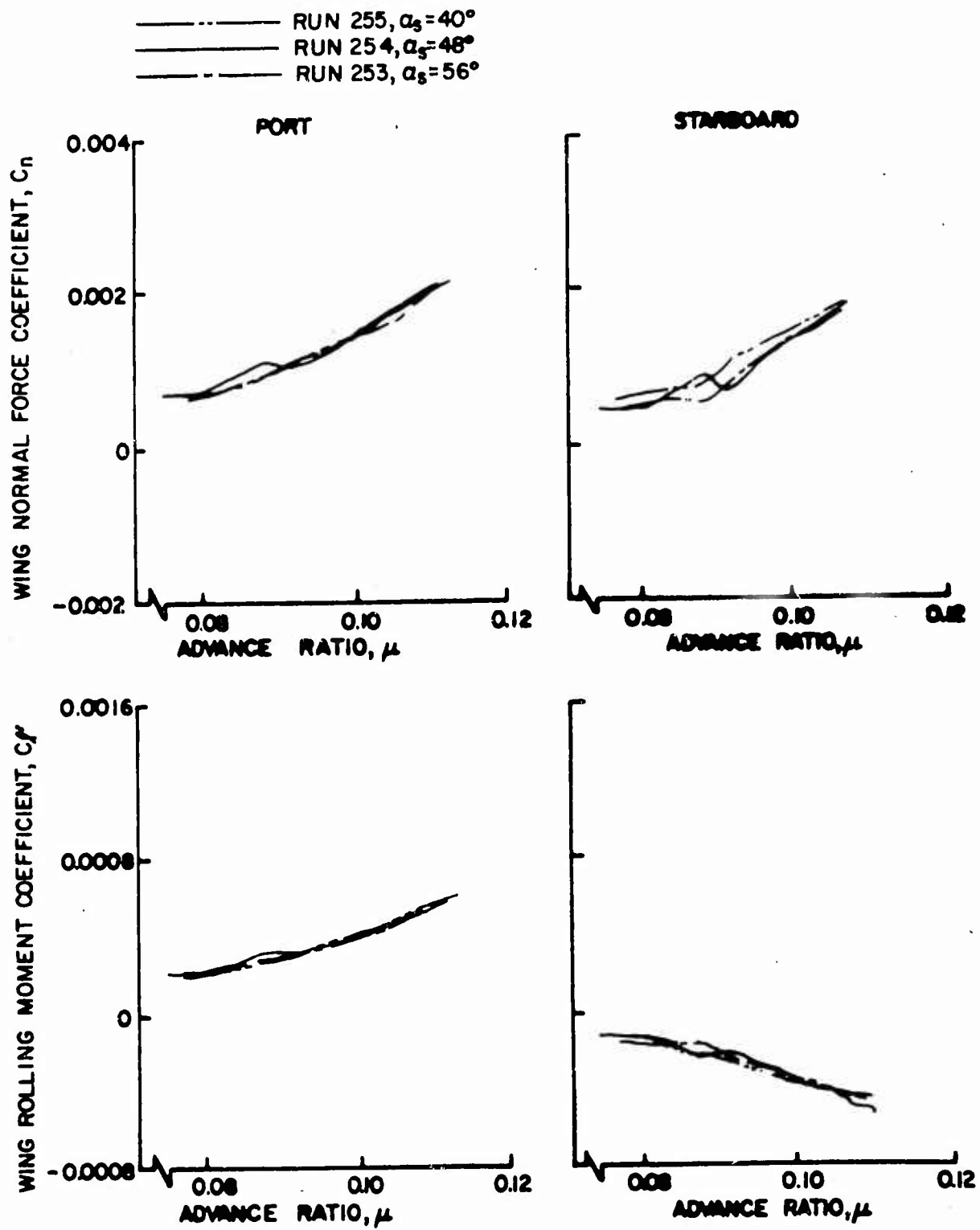
Figure 52. Wing Normal Force and Rolling Moment Coefficients as Functions of Advance Ratio, \theta = 4^\circ , Large Wing on Low.
