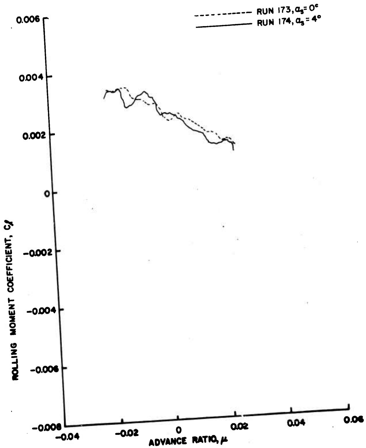
Figure 121c. Rotor Force and Moment Coefficients as Functions of Sideslip Ratio, \theta_{.75R} = 10^\circ , Large Wing on High, \frac{h}{D} = 0.30 .
