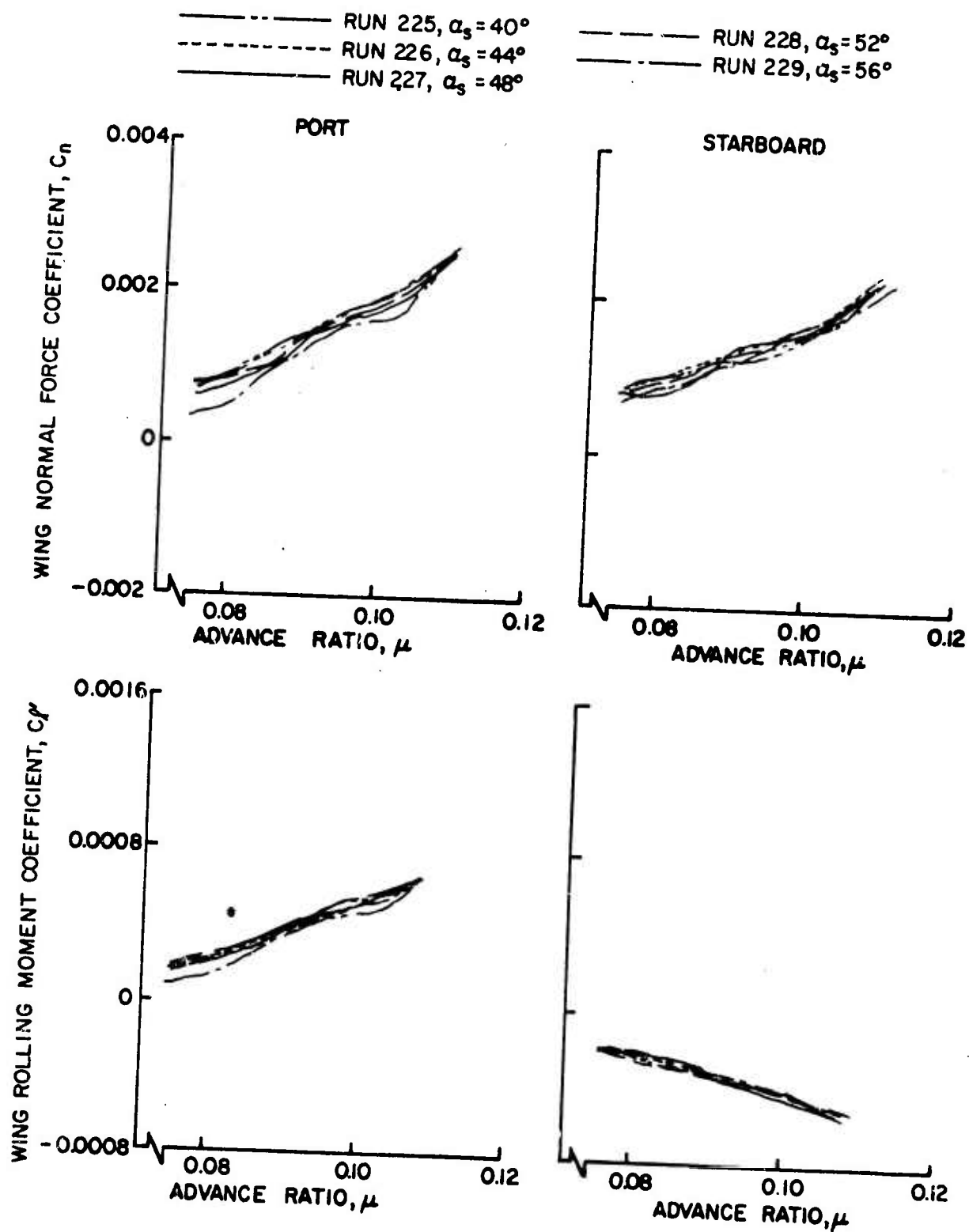
Figure 47. Wing Normal Force and Rolling Moment Coefficients as Functions of Advance Ratio, \theta = 2^\circ , .75R = 2^\circ , Large Wing on High.
