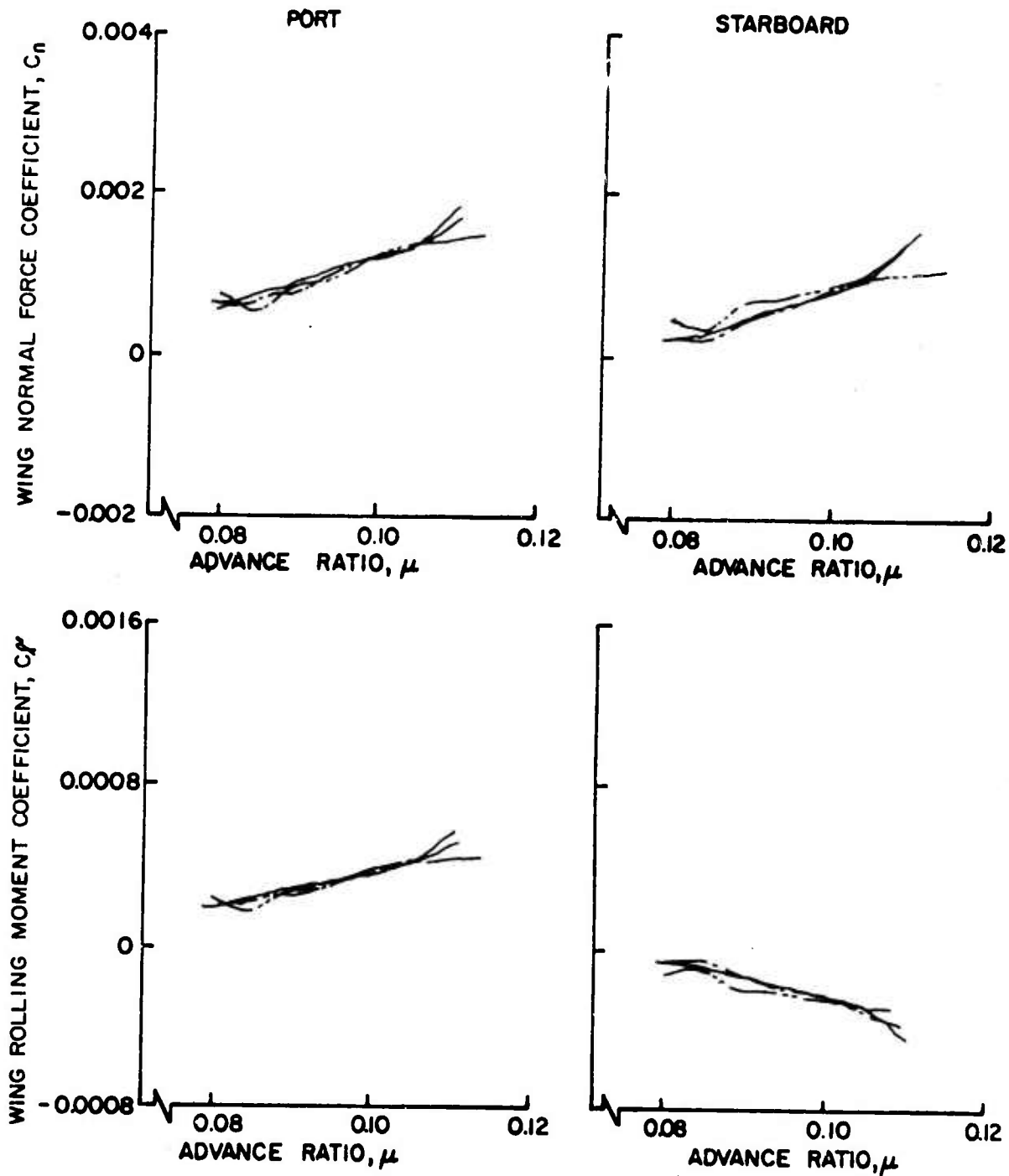
Figure 56. Wing Normal Force and Rolling Moment Coefficients as Functions of Advance Ratio, \theta_{.75R} = 4^\circ , Small Wing on Low.
