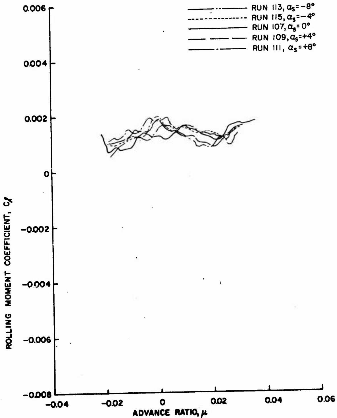
Figure 67c. Rotor Force and Moment Coefficients as Functions of Advance Ratio, \theta = 10^\circ , Wing Off, Fuselage Off, \frac{h}{D} = 0.75 .
