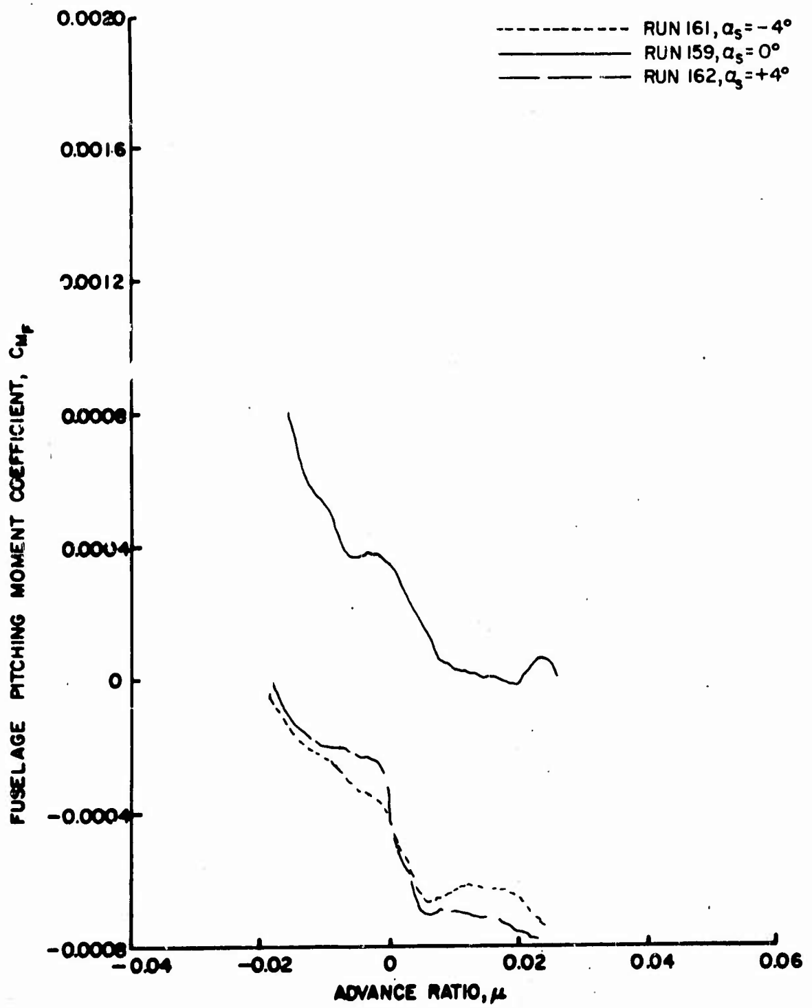
Figure 104b. Fuselage Vertical Force and Pitching Moment Coefficients as Functions of Advance Ratio, \theta = 10^\circ , Large Wing on Low, \frac{h}{D} = 0.30 .
