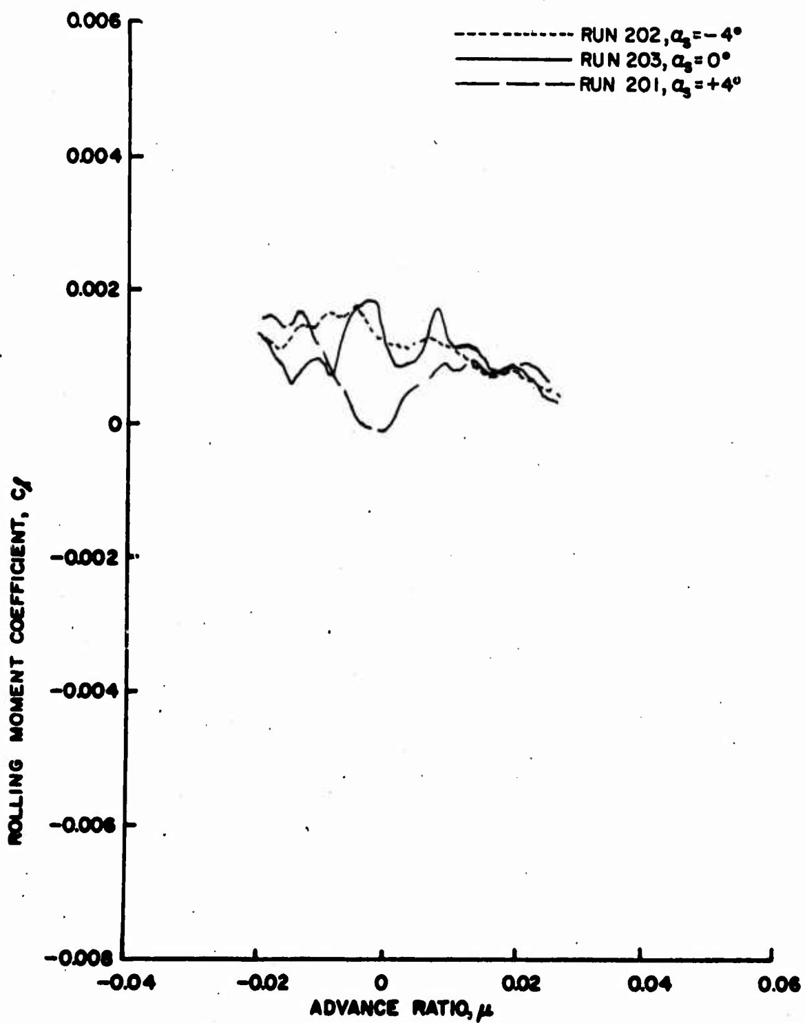
Figure 89c. Rotor Force and Moment Coefficients as Functions of Advance Ratio, \theta = 12^\circ , Wing Off, Fuselage Off, \frac{h}{D} = 0.30 .
