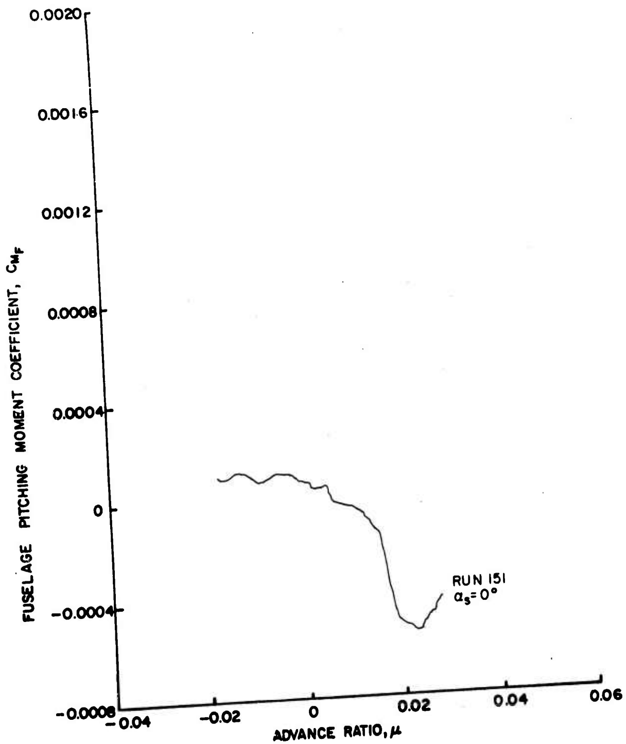
Figure 81. Fuselage Vertical Force and Pitching Moment Coefficients as Functions of Advance Ratio, \theta = 8^\circ , Large Wing on Low, \frac{h}{D} = 0.75 .
