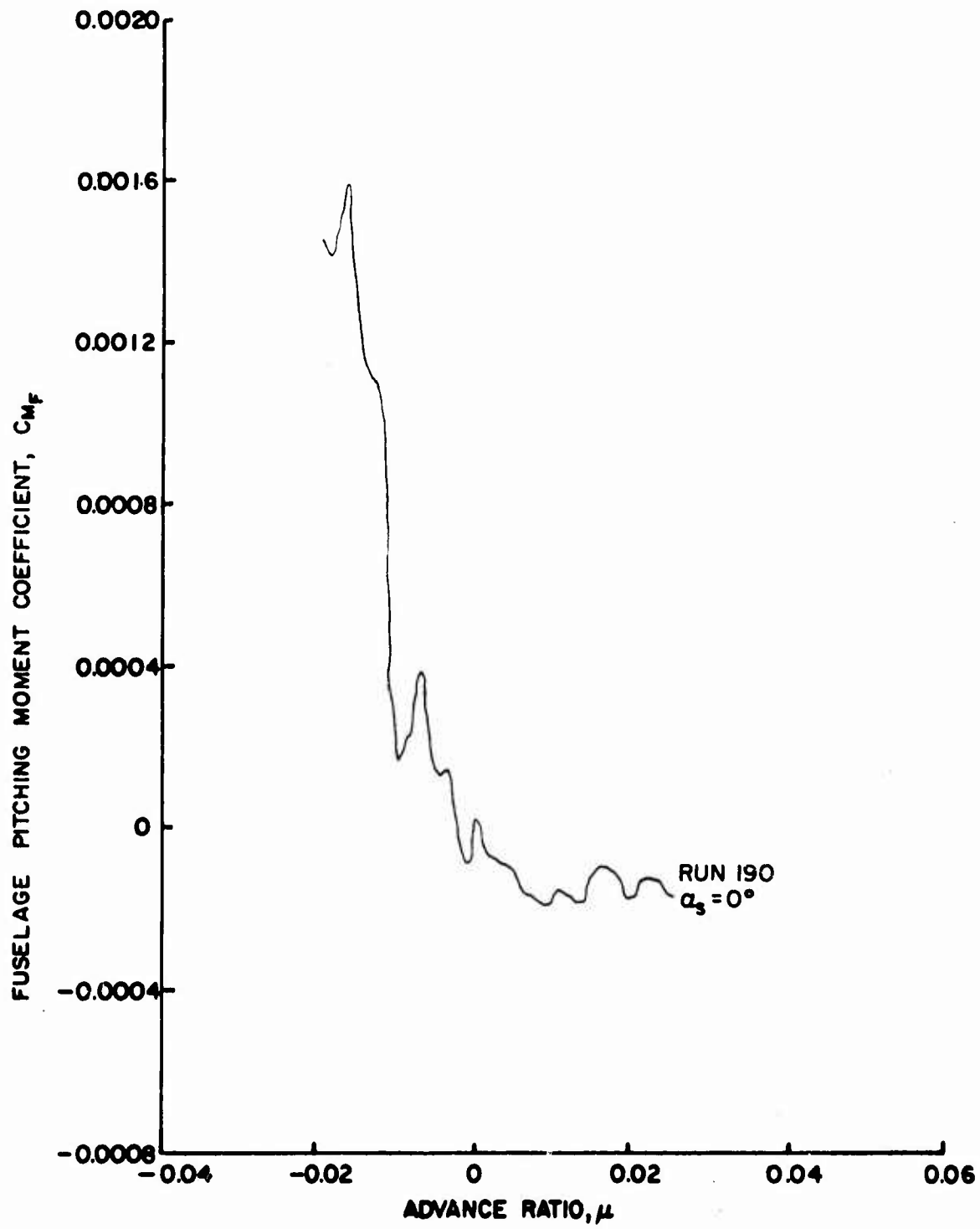
Figure 95b. Fuselage Vertical Force and Pitching Moment Coefficients as Functions of Advance Ratio, \theta = 12^\circ , Wing Off, Fuselage On, \frac{h}{D} = 0.30 .
