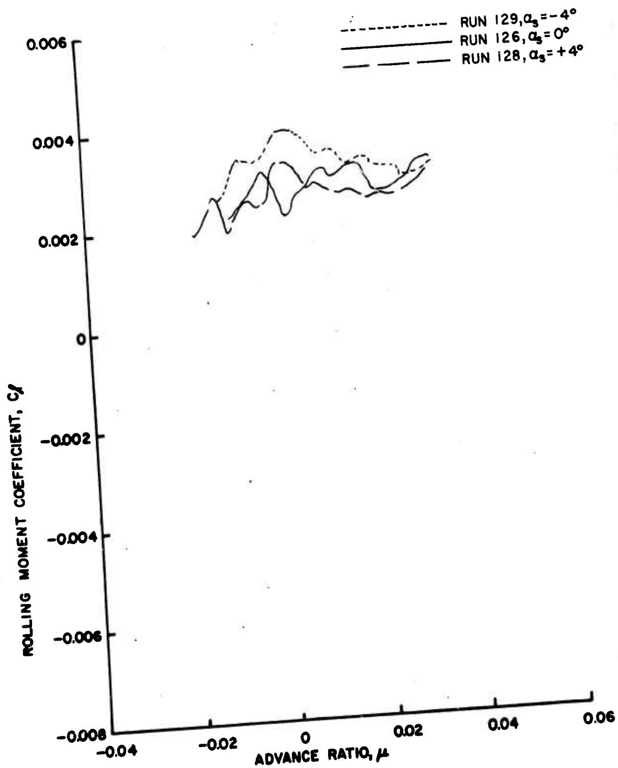
Figure 71c. Rotor Force and Moment Coefficients as Functions of Advance Ratio, \theta = 10^\circ , Wing Off, Fuselage On, \frac{h}{D} = 0.75 .
