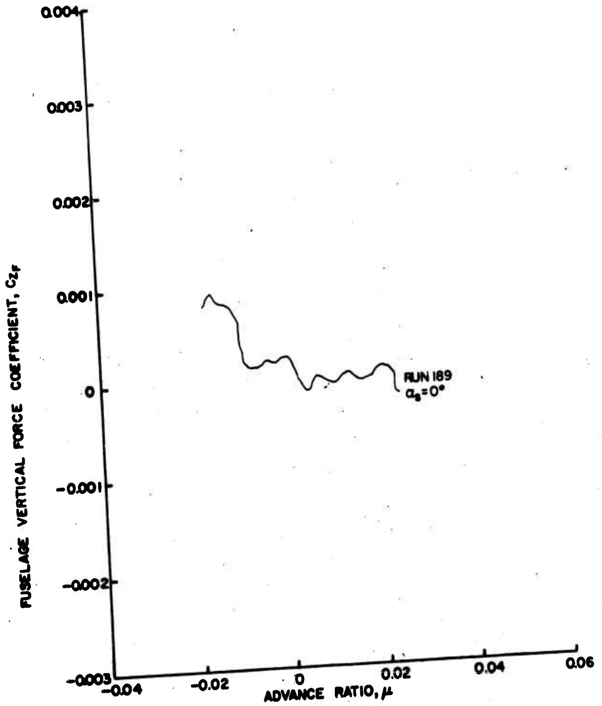
Figure 91a. Fuselage Vertical Force and Pitching Moment Coefficients as Functions of Advance Ratio, \theta = 8^\circ , Wing Off, Fuselage On, \frac{h}{D} = 0.30 .
