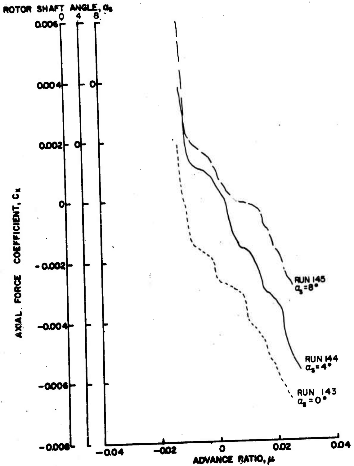
Figure 111a. Rotor Force and Moment Coefficients as Functions of Advance Ratio, \theta = 10^\circ , Large Wing on High, \frac{h}{D} = 0.75 .
