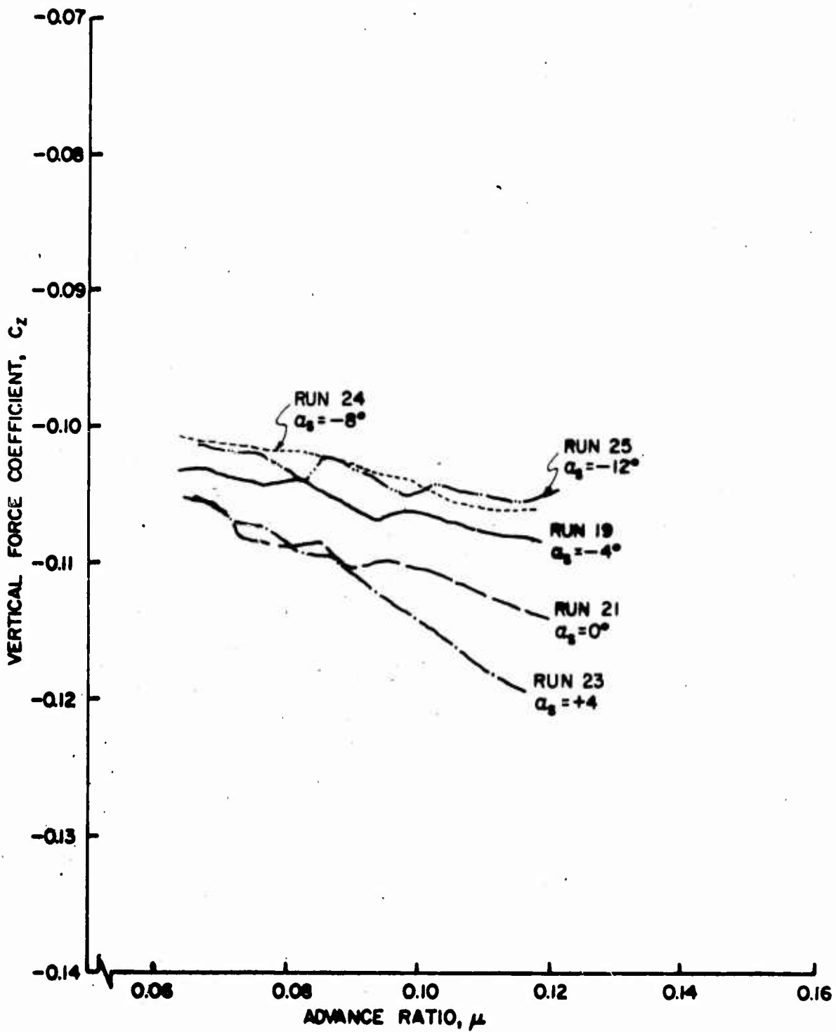
Figure 24b. Rotor Force and Moment Coefficients as Functions of Advance Ratio, \theta = 10^\circ , Wing Off.
