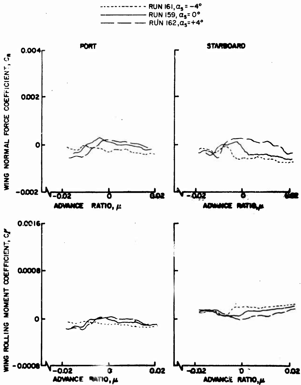
Figure 105. Wing Normal Force and Rolling Moment Coefficients as Functions of Advance Ratio, \theta = 10^\circ , Large Wing on \frac{b}{D} = 0.30 .
