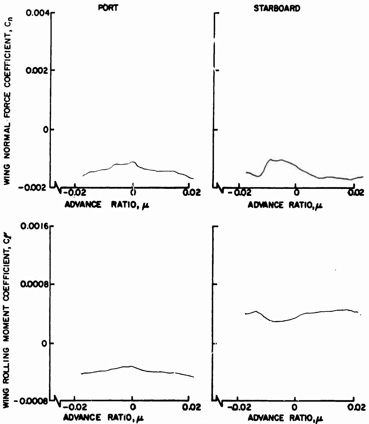
Figure 82. Wing Normal Force and Rolling Moment Coefficients as Functions of Advance Ratio, \theta = 8^\circ , Large Wing on Low, \frac{h}{D} = 0.75 .
