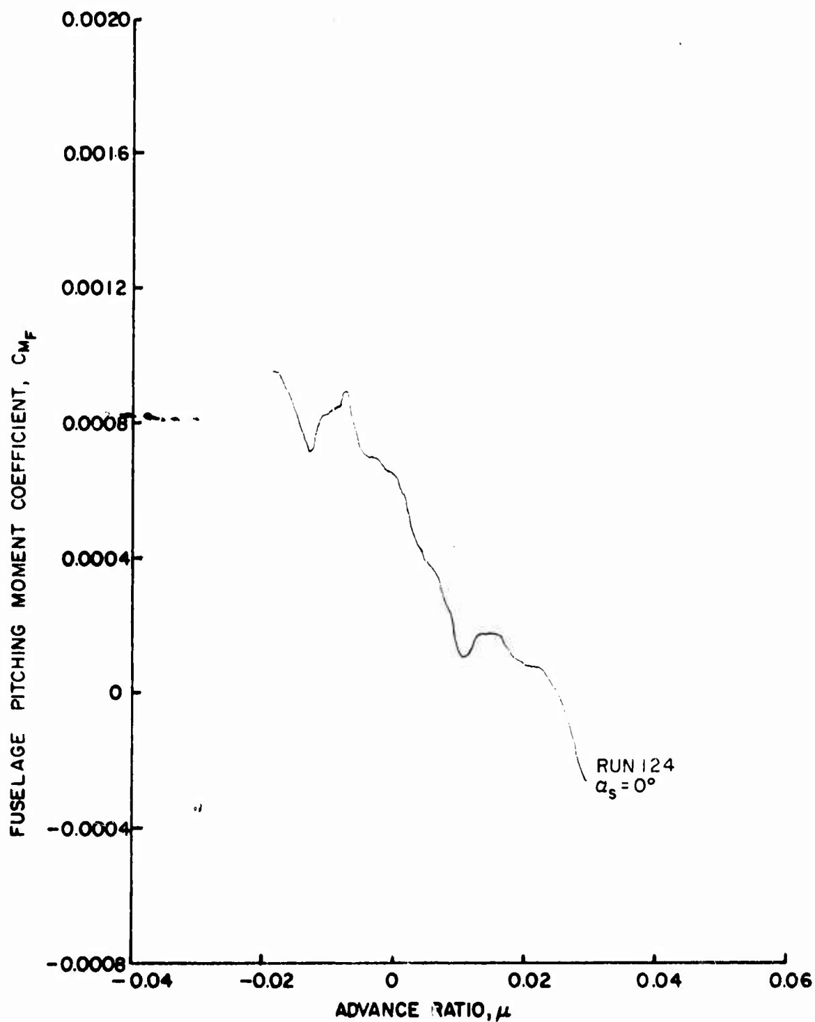
Figure 74b. Fuselage Vertical Force and Pitching Moment Coefficients as Functions of Advance Ratio, \theta_{15R} = 12^\circ , Wing Off, Fuselage On, \frac{h}{D} = 0.75 .
