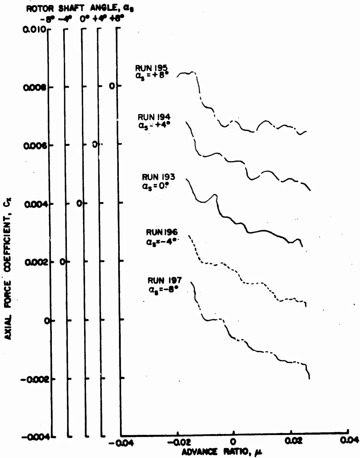
Figure 88a. Rotor Force and Moment Coefficients as Functions of Advance Ratio, \theta = 10^\circ , Wing Off, Fuselage Off, \frac{h}{D} = 0.30 .
