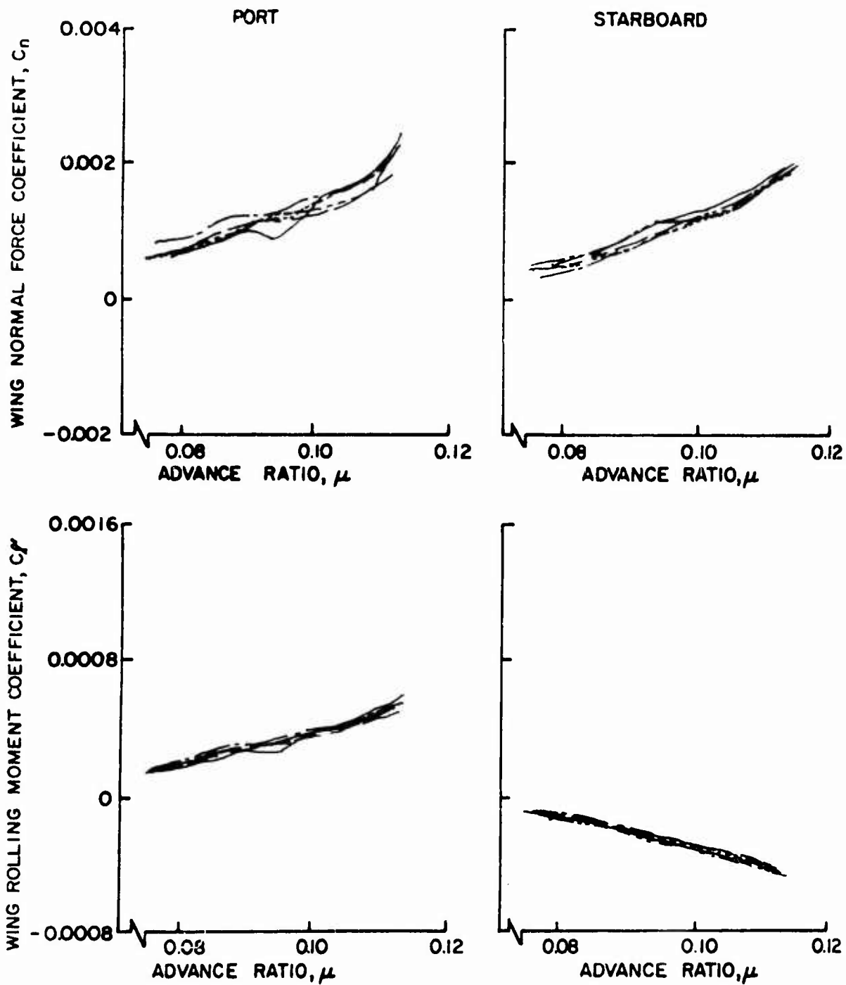
Figure 50. Wing Normal Force and Rolling Moment Coefficients as Functions of Advance Ratio, \theta = 4^\circ , Large Wing on High.
