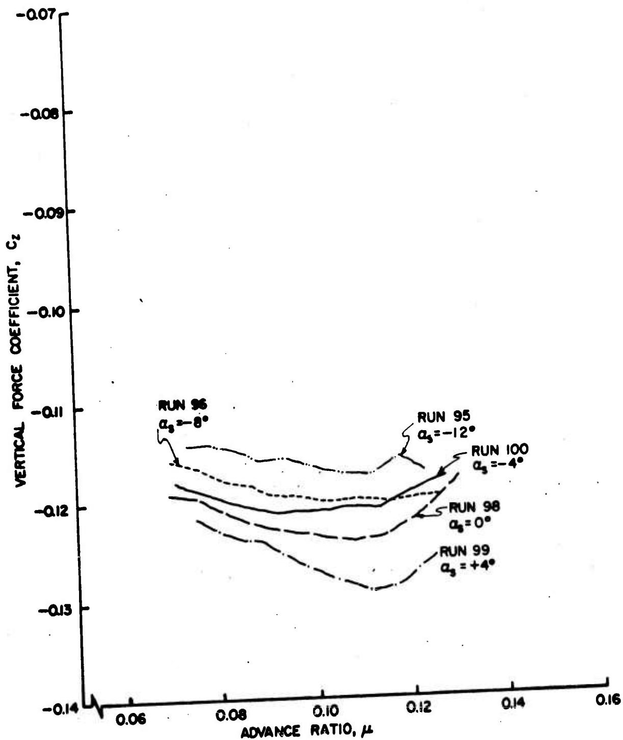
Figure 37b. Rotor Force and Moment Coefficients as Functions of Advance Ratio, \theta = 12^\circ , Large Wing on High.
