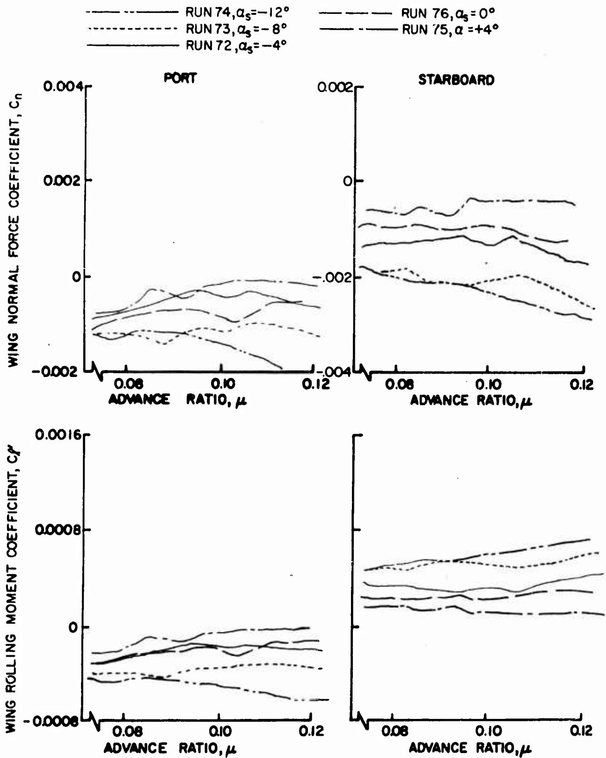
Figure 17. Wing Normal Force and Rolling Moment Coefficients as Functions of Advance Ratio, \theta = 8^\circ , Large Wing on High.
