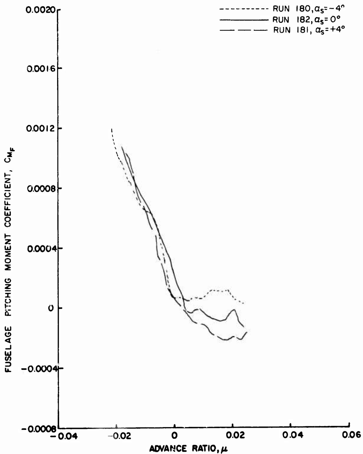
Figure 106b. Fuselage and Vertical Force and Fitching Moment Coefficients as Functions of Advance Ratio, \theta_{.75R} = 10^\circ , Small Wing on High, \frac{h}{D} = 0.30 .
