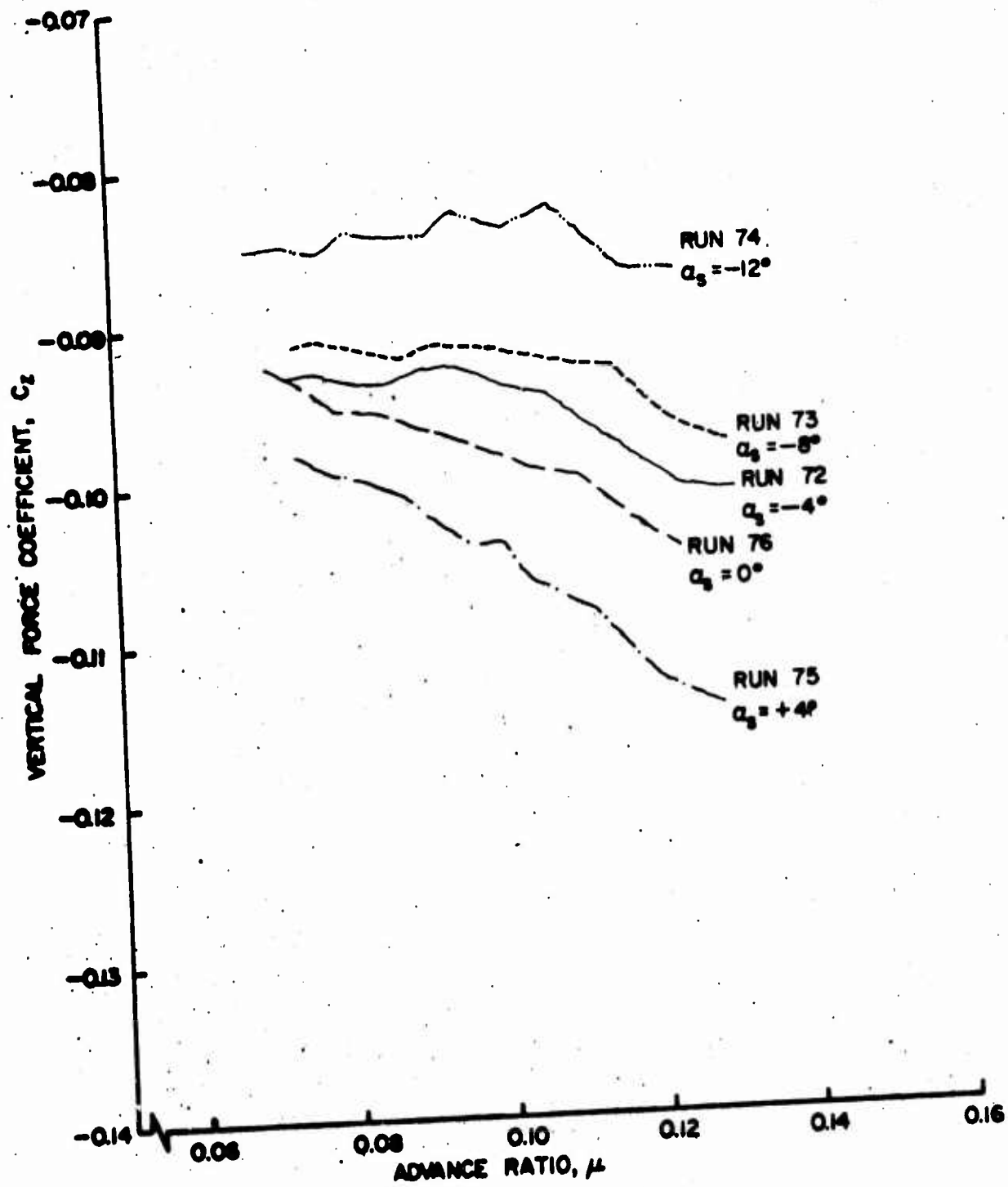
Figure 15b. Rotor Force and Moment Coefficients as Functions of Advance Ratio, \theta = 8^\circ , Large Wing on High.
