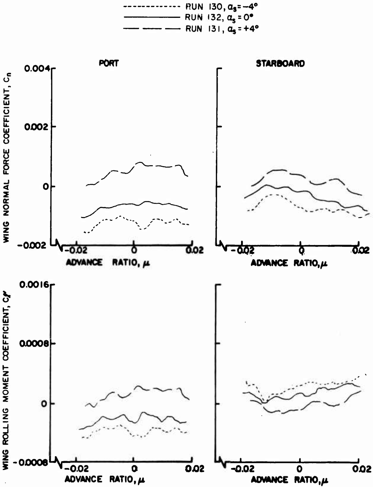
Figure 86. Wing Normal Force and Rolling Moment Coefficients as Functions of Advance Ratio, \theta = 10^\circ , Small Wing on High, \frac{h}{D} = 0.75 .
