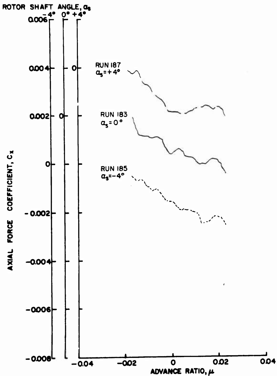
Figure 92a. Rotor Force and Moment Coefficients as Functions of Advance Ratio, \theta_{75^\circ} = 10^\circ , side off, Fuselage On, \frac{h}{D} = 0.30 .
