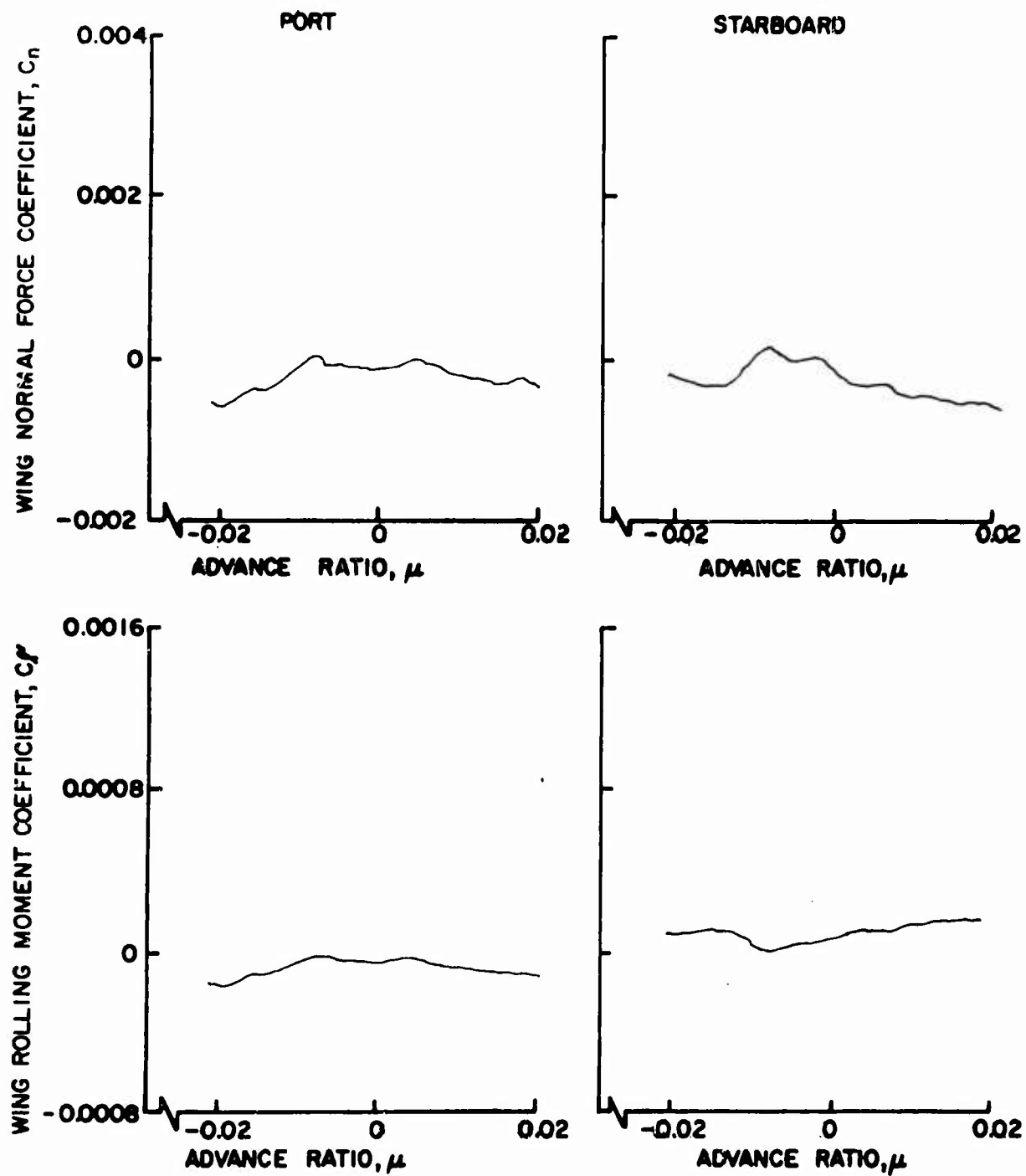
Figure 103. Wing Normal Force and Rolling Moment Coefficients as Functions of Advance Ratio, \theta = 8^\circ , Large Wing on Low, \frac{h}{D} = 0.30 .
