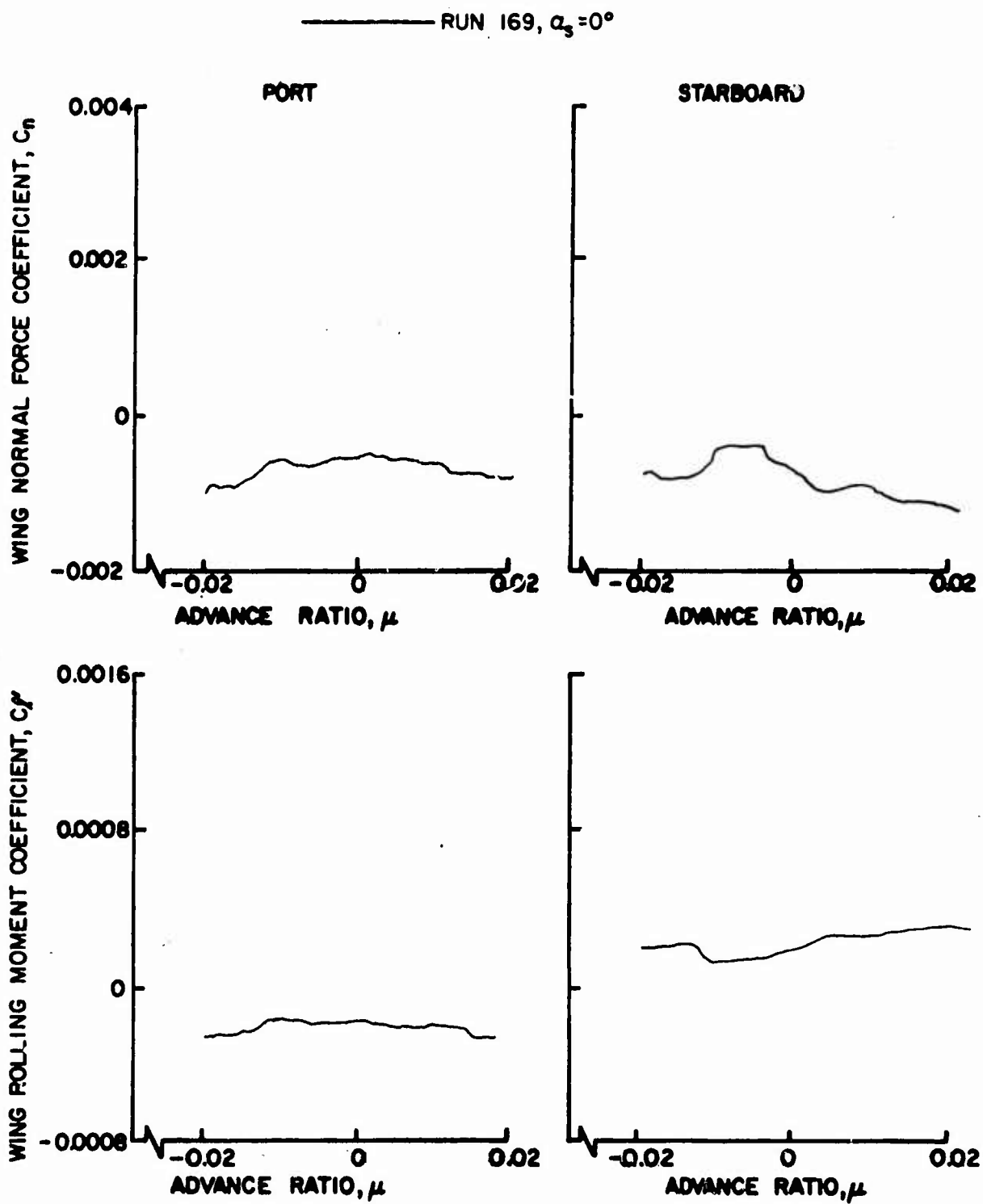
Figure 98. Wing Normal Force and Rolling Moment Coefficients as Functions of Advance Ratio, \theta = 8^\circ , Large Wing on High, \frac{h}{D} = 0.30 .
