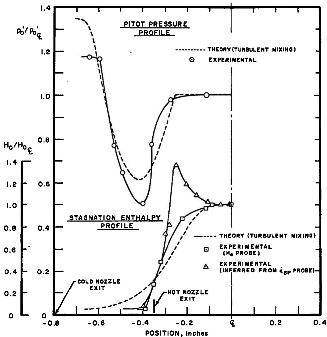
Fig. 21 Comparison of Theoretical and Experimental Profiles of Pitot Pressure and Stagnation Enthalpy, p_{oH} = 20.1 atm, H_{oHB} = 2350 Btu/lbm
