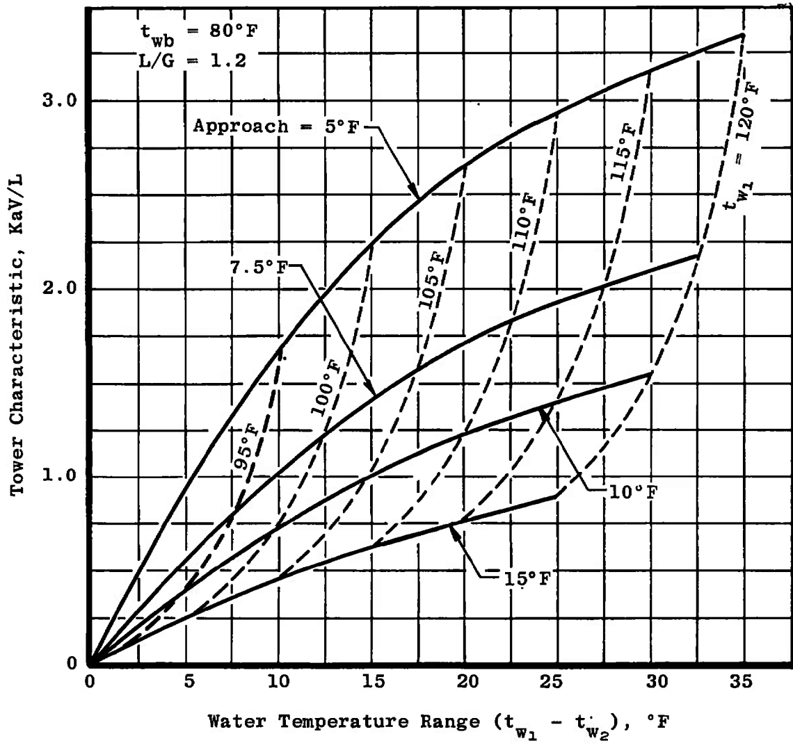
Fig. 11 Tower Characteristic versus Water Temperature Range for t_{wb} = 80^{\circ}F and L/G = 1.2
