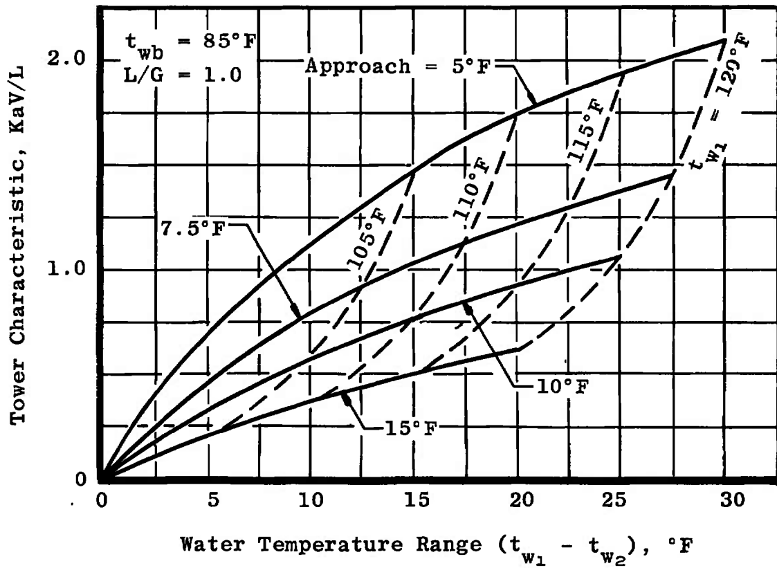
Fig. 13 Tower Characteristic versus Water Temperature Range for t_{wb} = 85^{\circ}\text{F} and L/G = 1.0
