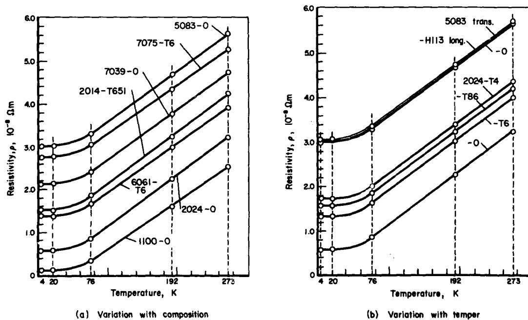
FIGURE 3. ELECTRICAL RESISTIVITY OF ALUMINUM ALLOYS AT LOW TEMPERATURE(8)
