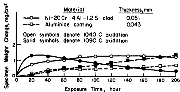
FIGURE 1. COMPARISON OF CYCLIC OXIDATION RESISTANCE OF Ni-20Cr-4Al-1.2Si CLAD IN-100 AND COMMERCIAL ALUMINIDE-COATED IN-100 AT 1040 AND 1090 C. (4)
