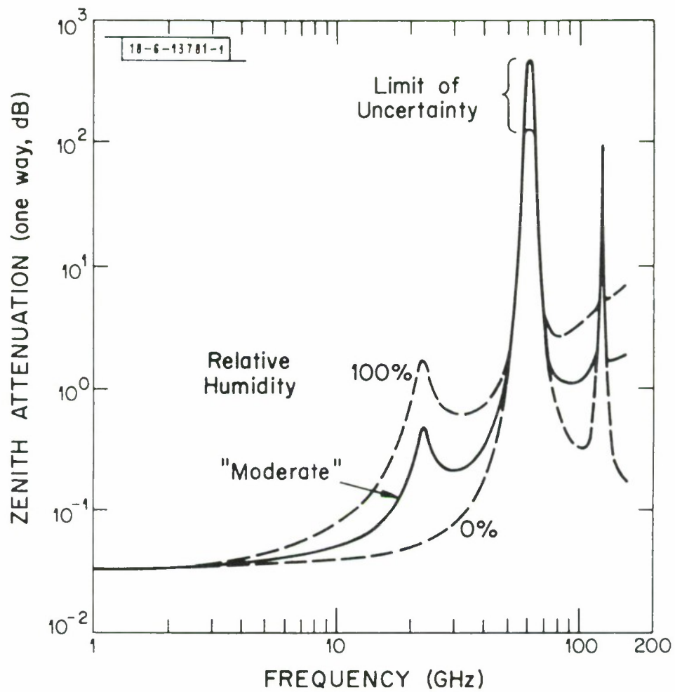
Fig. 1. Zenith attenuation vs frequency. (After R. K. Crane, Ref. 24.)
