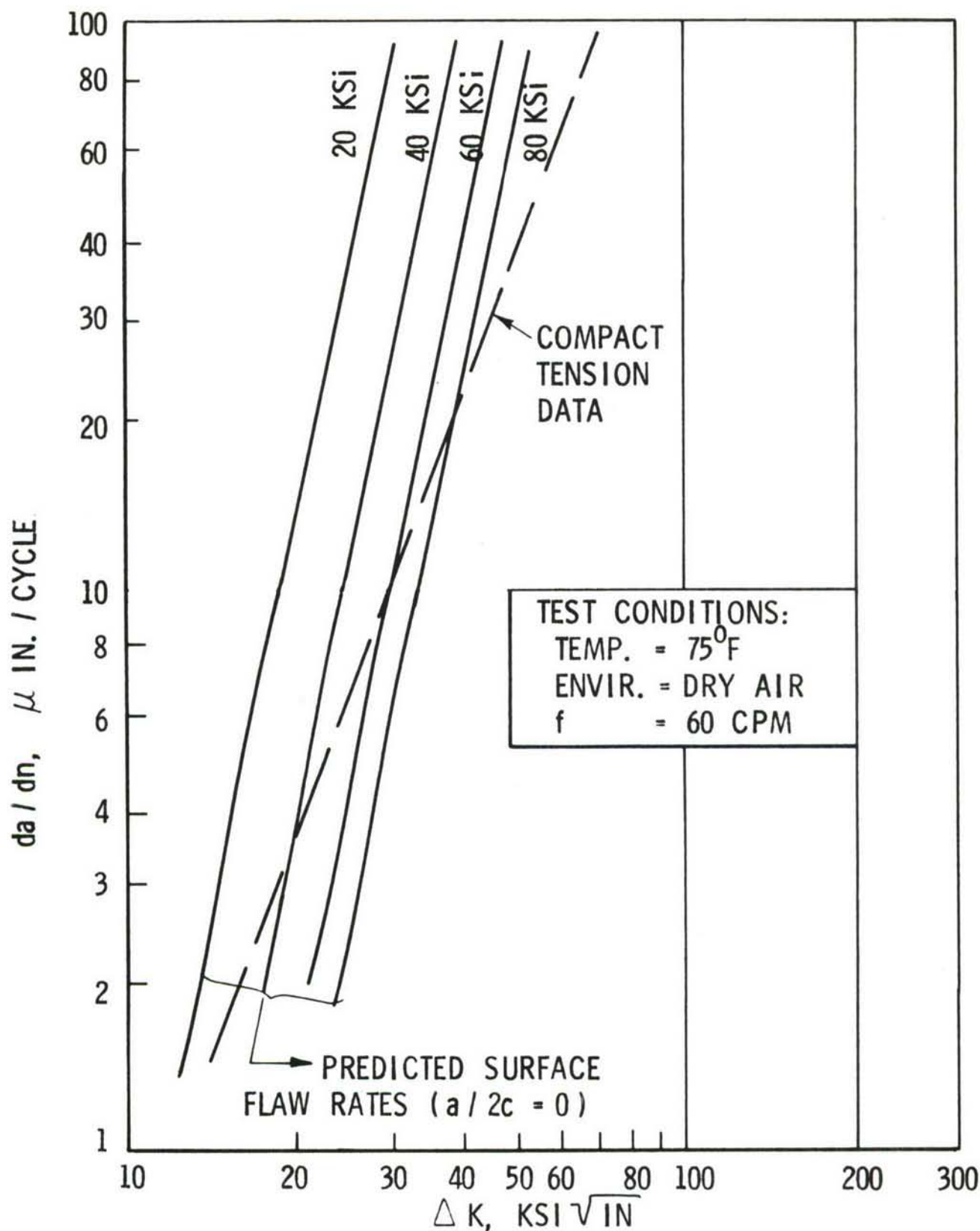
FIGURE 26: SURFACE FLAW DATA ADJUSTED TO a/2c = 0 & COMPARED WITH COMPACT TENSION DATA (REF. 15)
