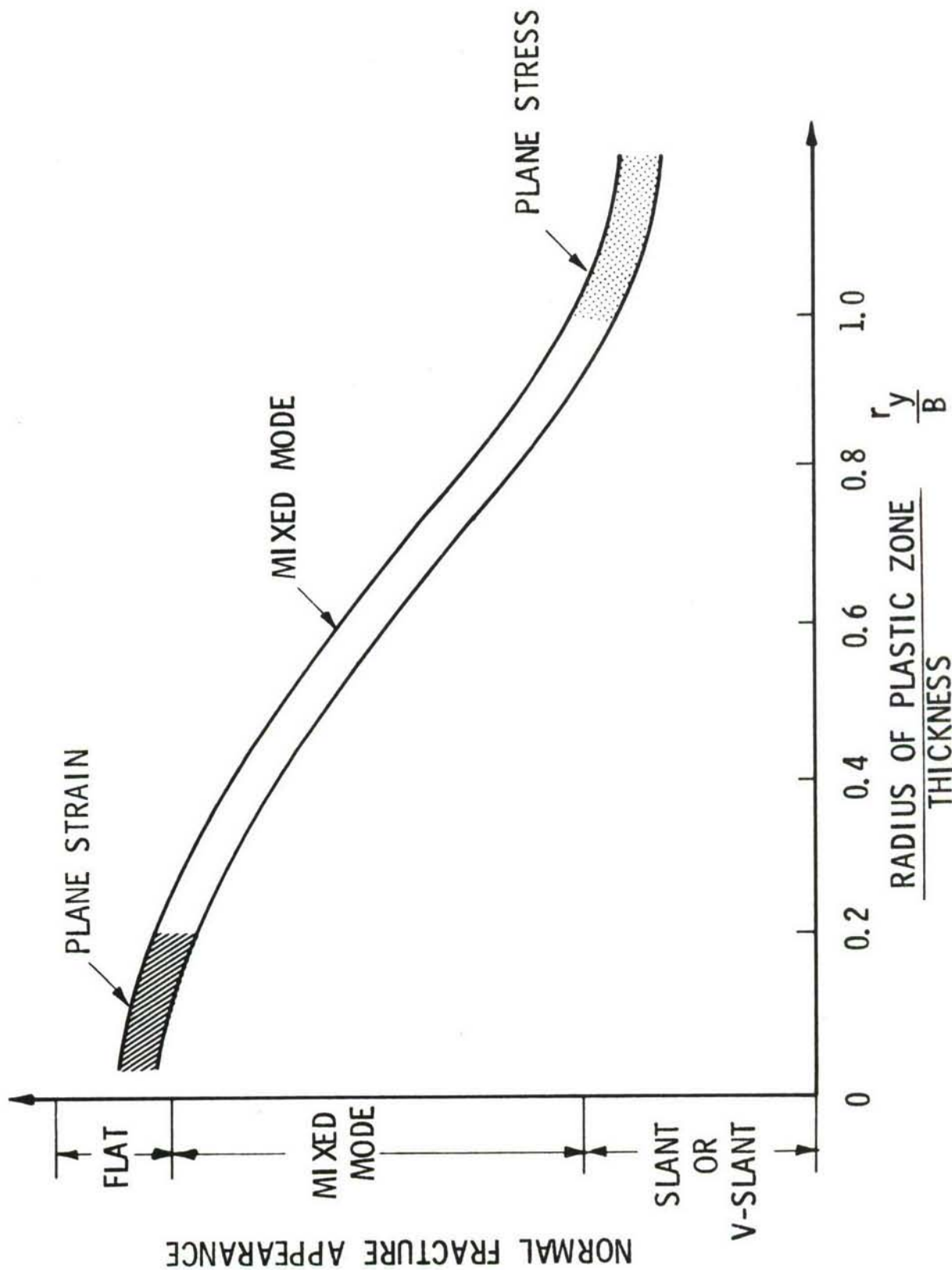
FIGURE 7. TREND IN FRACTURE MODE APPEARANCE VS. CRACK TIP PLASTIC ZONE PARAMETER REF. 4
