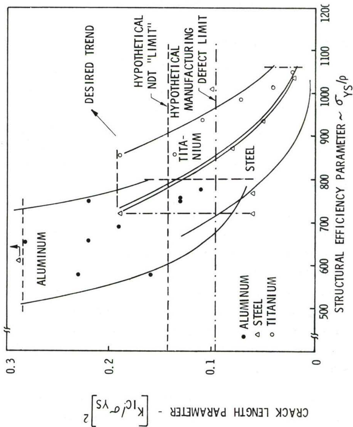
FIGURE 4. CRACK LENGTH PARAMETER VARIATION WITH STRUCTURAL EFFICIENCY PARAMETER
