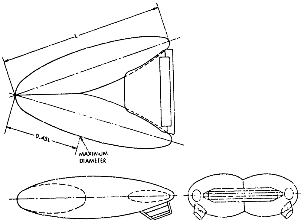
Figure 2. Vee-Balloon Configuration
