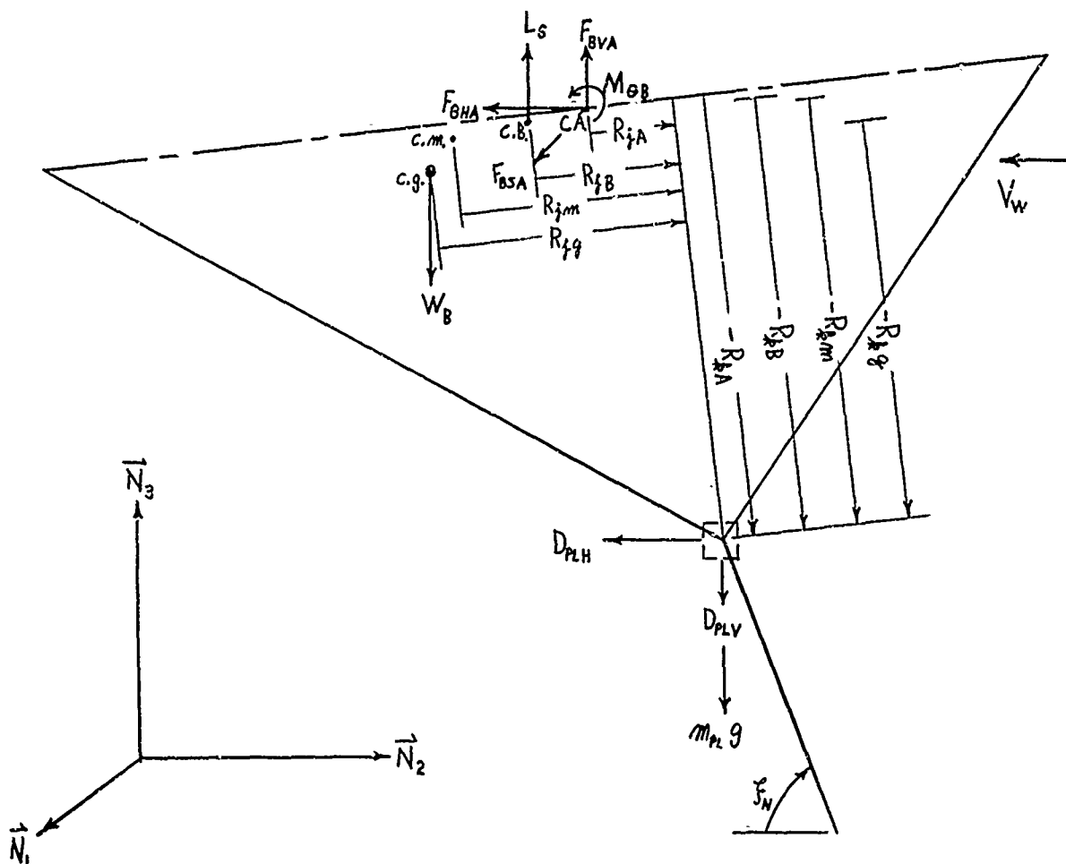
Figure 59 Applied Forces Acting on Balloon
