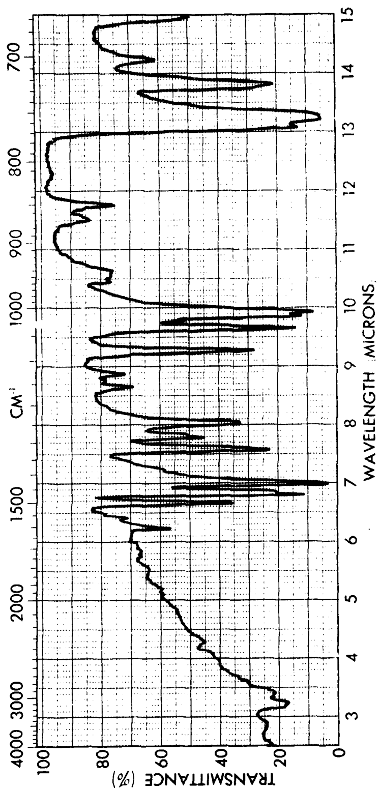
FIGURE III - 25% MBT, 75% BTD
