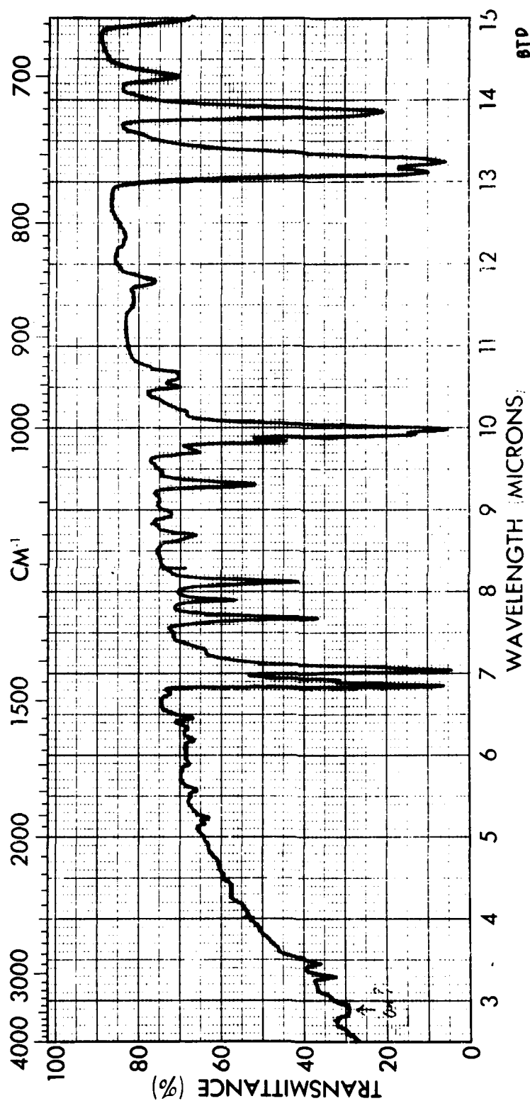
FIGURE 11 - BENZOTHIAZYL DISULFIDE
