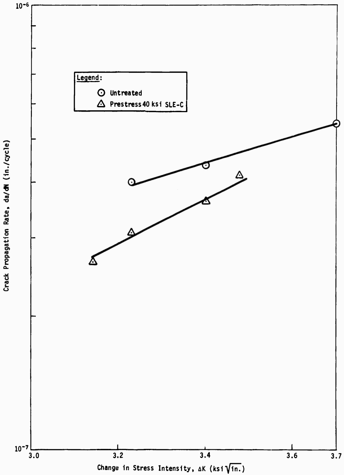
Fig. III-16 Crack Propagation Behavior of Aluminum 2014-T6 Under Plane Stress Conditions, Center-Cracked Specimens 0.125-Inch Thick
