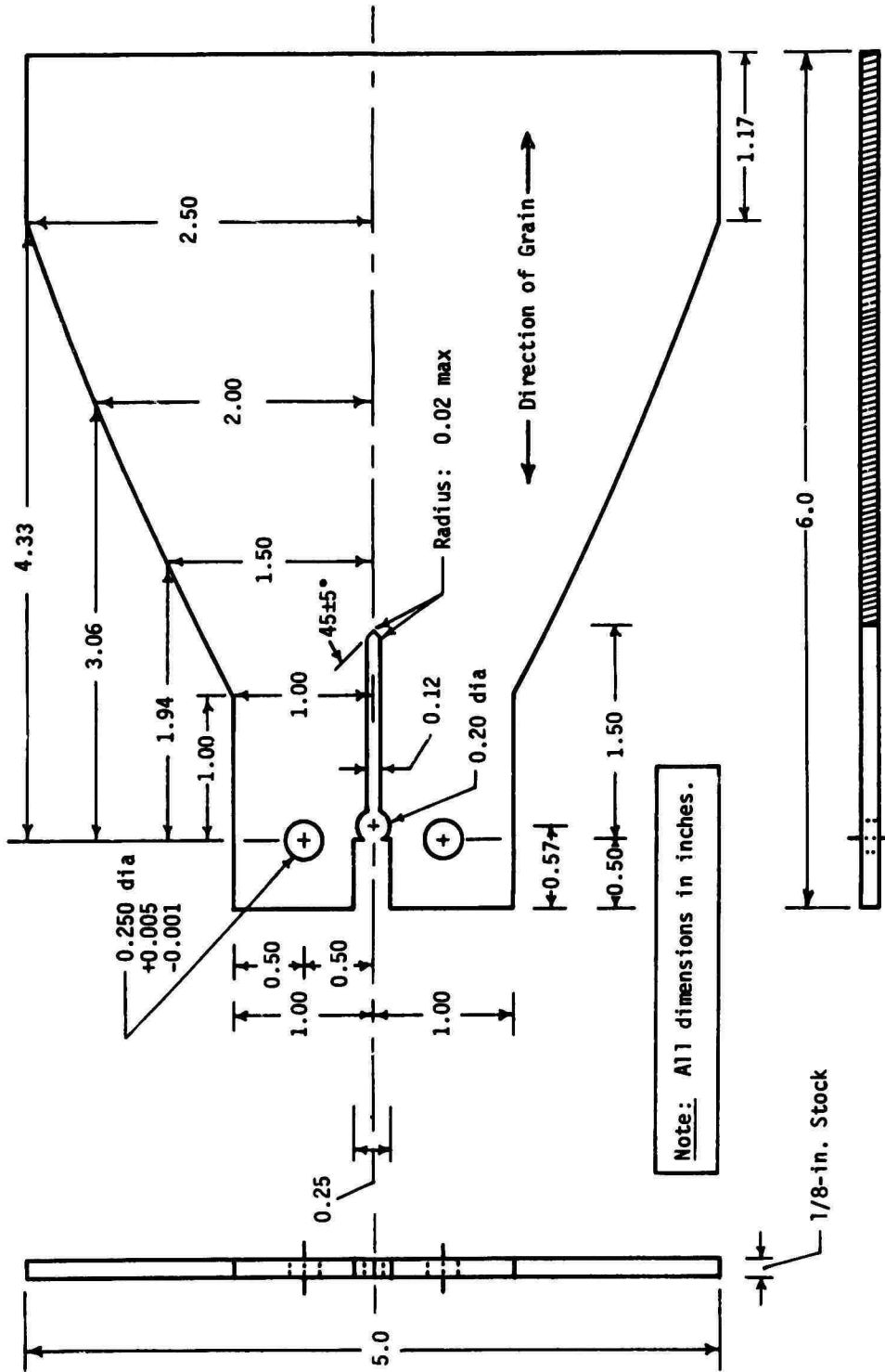
Fig. II-6 Ripling Type M-4 Test Specimen
