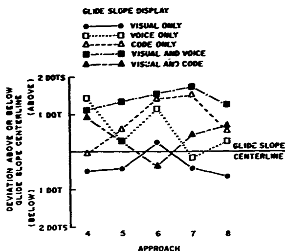
FIGURE 8. Mean glide slope deviation (algebraic) at middle marker.
