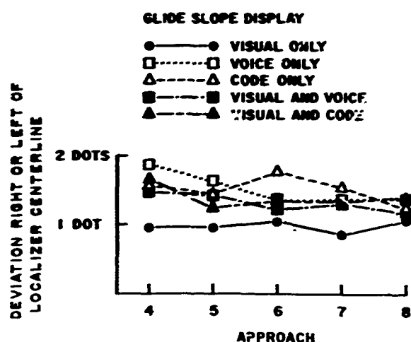
FIGURE 7. Means of maximum deviation right or left of localizer centerline, for all segments combined within groups.
