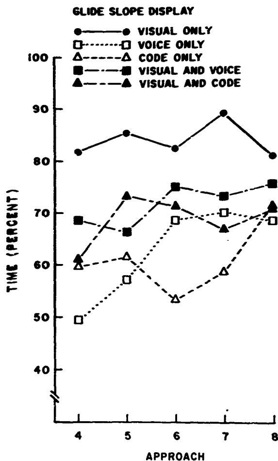
FIGURE 6. Time (percent) in which localizer deviation did not exceed one dot.
