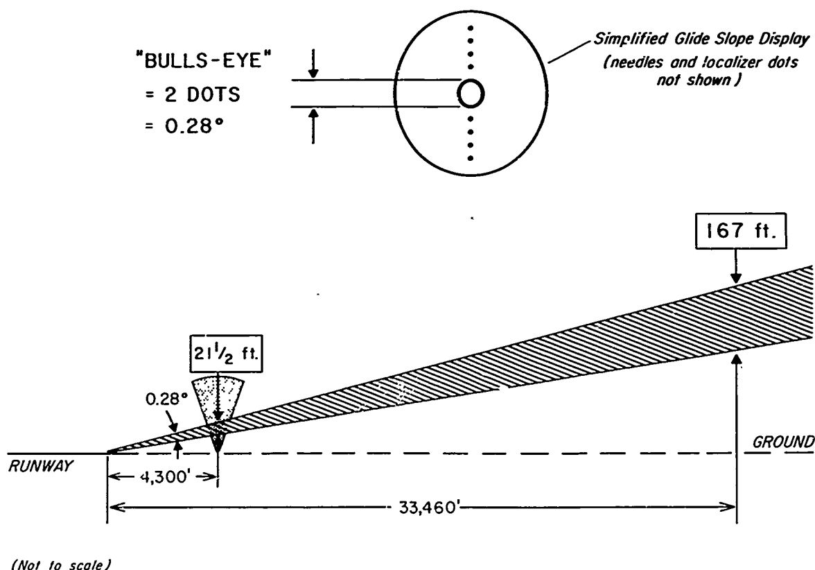
FIGURE 12. A two dot deviation, equal to a vertical displacement of the glide slope needle across the span of the crosspointer bull's eye, is equal to about 0.28 of subtended angle, resulting in a narrowing of the glide slope "beam" as the middle marker is approached.
