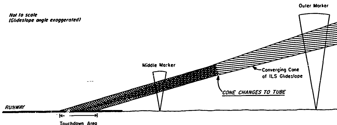
FIGURE 13. Man's response characteristics might be more compatible with display interface if rate and magnitude of needle movement were a function of a tubular, rather than a conical, ILS glide slope "beam".
