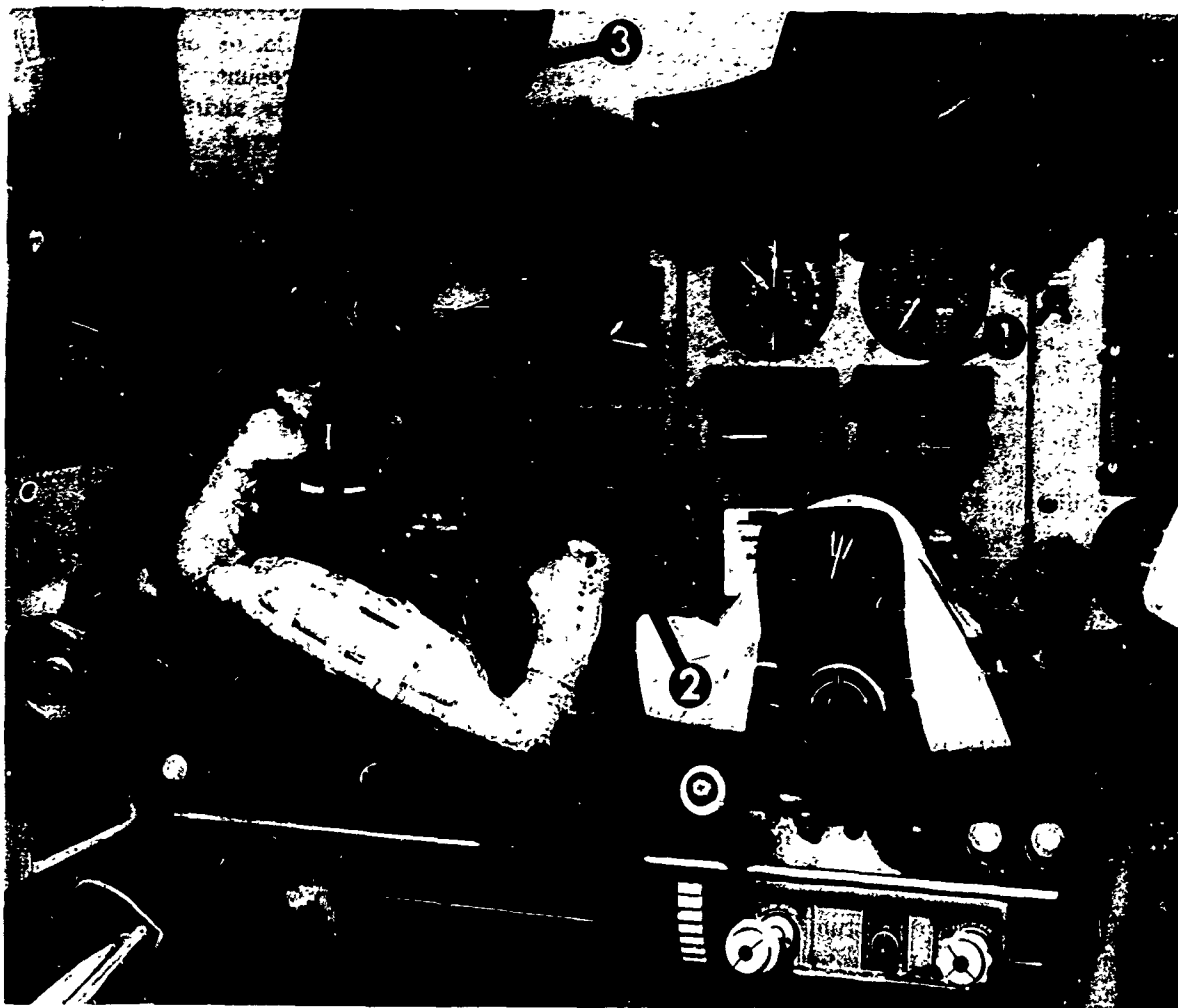
FIGURE 2. Primary flight instruments in research aircraft were arranged in "T" configuration with exception of vertical speed indicator (Arrow #1), which was moved to the right to permit a more centrally located glide slope/localizer indicator (Arrow #2). Removable "slats" (Arrow #3) simulated instrument weather environment for subjects without interfering with safety pilot's outside vision.
