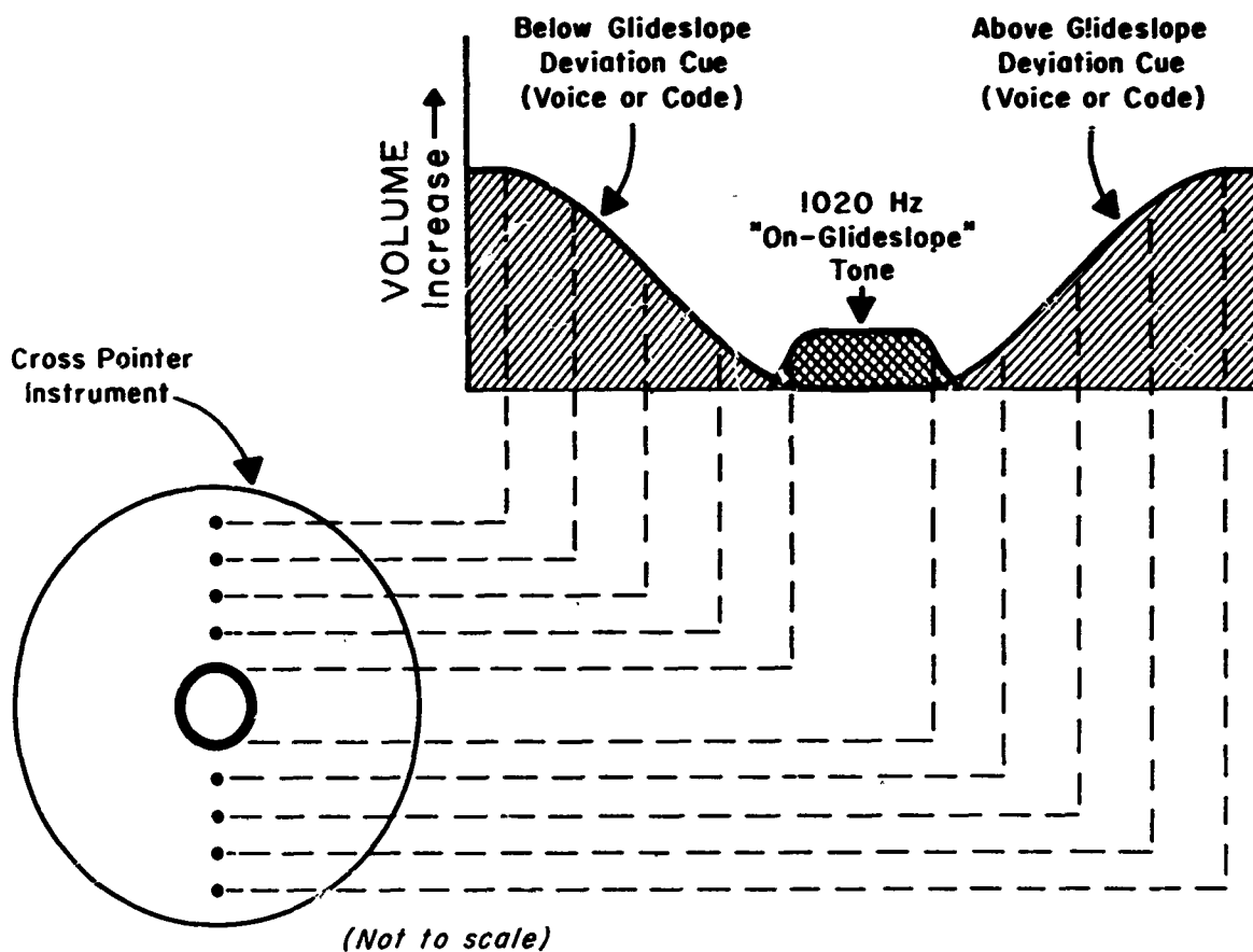
FIGURE 4. Idealized illustration shows relationships of volume of aural cues to aircraft deviation above or below glide slope centerline. A 1020 Hz tone provided "on-course" guidance.
