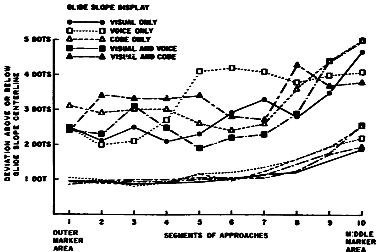
FIGURE 5. Maximum deviations in either direction from glide slope centerline during approach segments. The upper group of curves indicate the largest single deviation during any experimental approach (#4 through #8) by any subject in the respective groups. The lower group of curves represents the combined means for all experimental approaches for all five groups.
