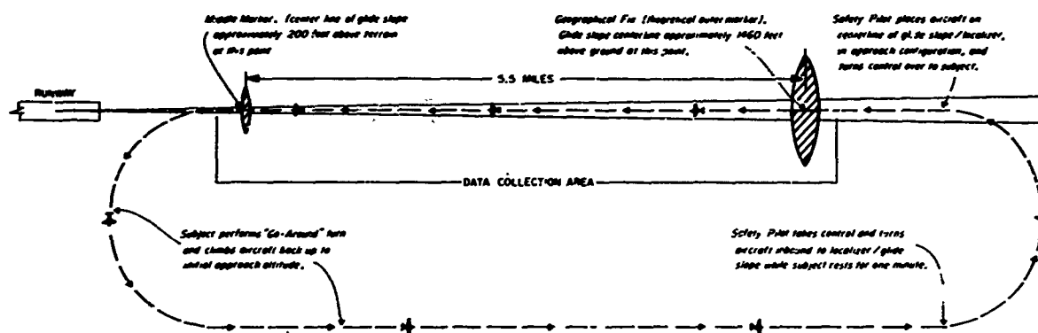
FIGURE 3. Flight path used during simulated instrument approaches. Each circuit required approximately ten minutes.
