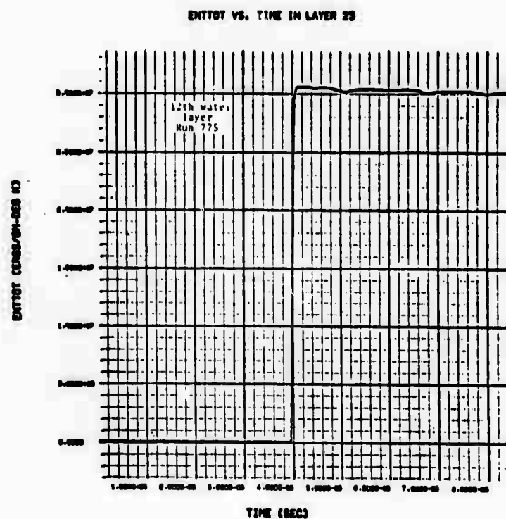
Fig. 3.6--Total entropy (ENTOT) in water and tuff laminates as a function of time.
