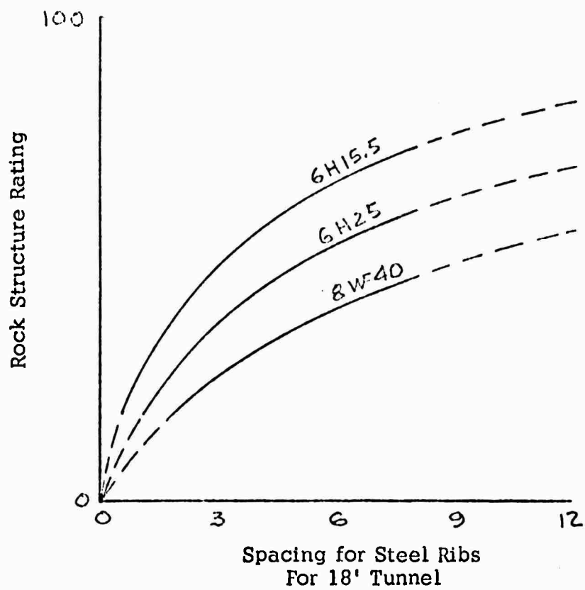
TYPICAL RIB SUPPORT CURVES
