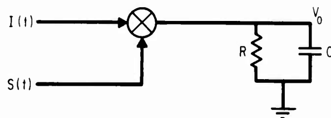
Fig. 6. Idealized Demodulator and Output Filter
